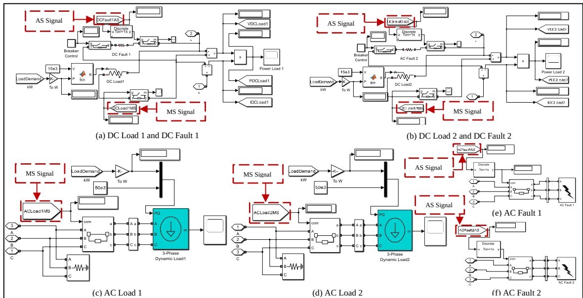
Figures D-4 (a) to (f): Integration of Manual and Automatic Switches into Loads (AC and DC) and Faults (AC and DC)
