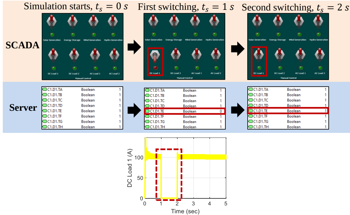
Figure 4.29: Manual Control of DC Load 1
