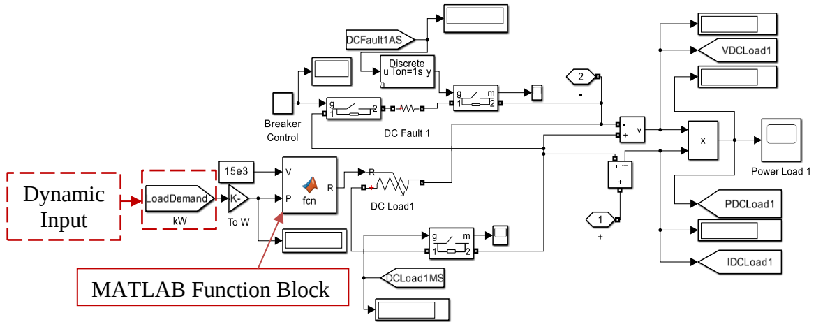
Figure 3.23: Dynamic DC Load Modeling
