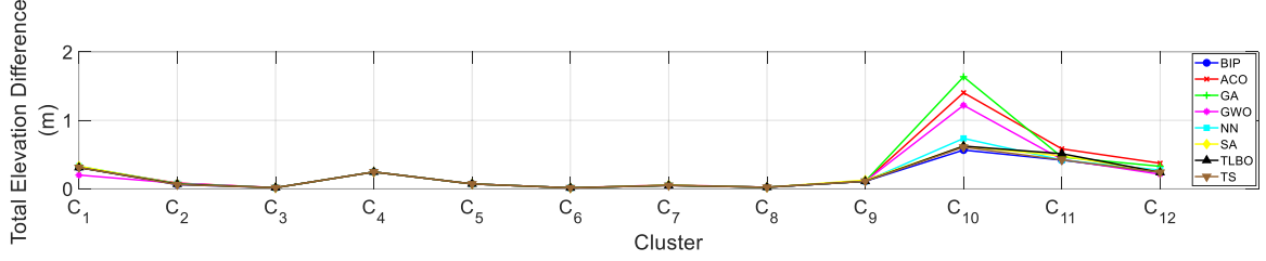
(b) \min (\sum \Delta e) of Fuzzy TSP Algorithms
