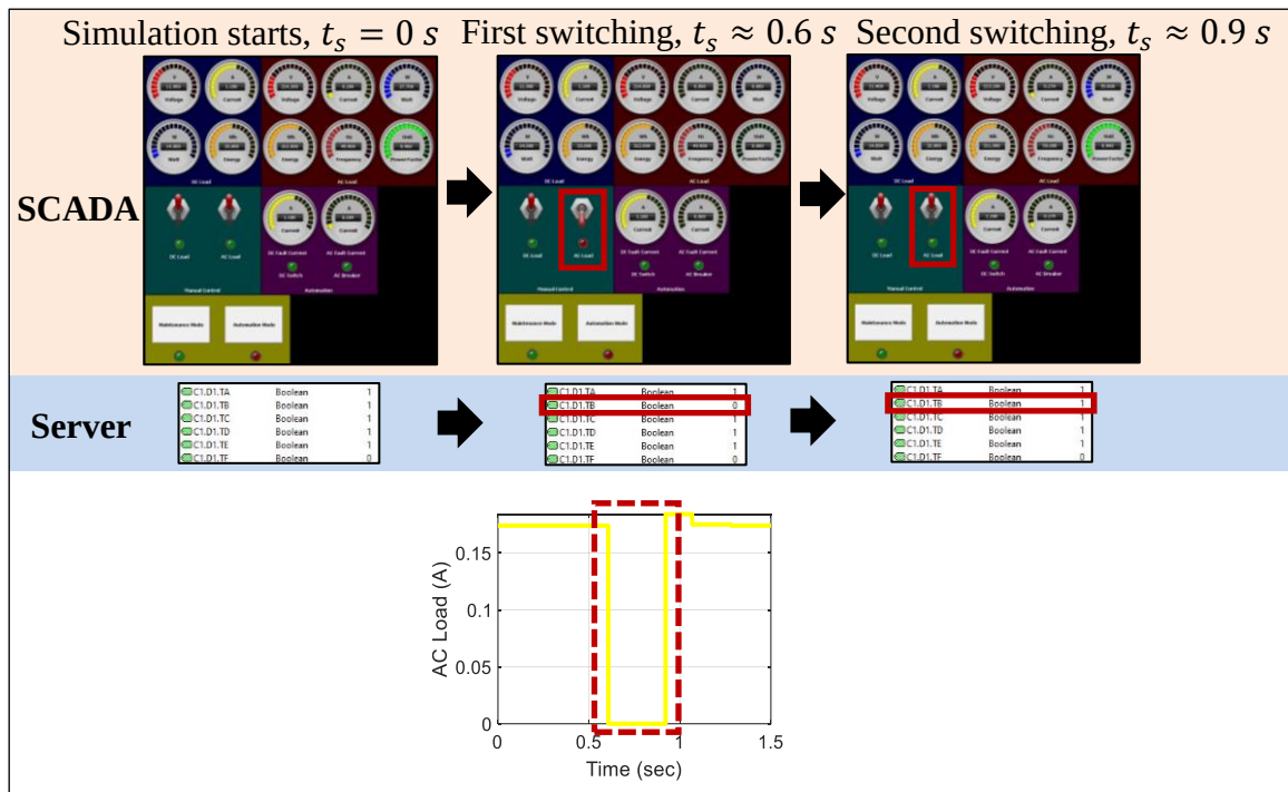
Figure 4.37: Manual Control of Actual AC Load
