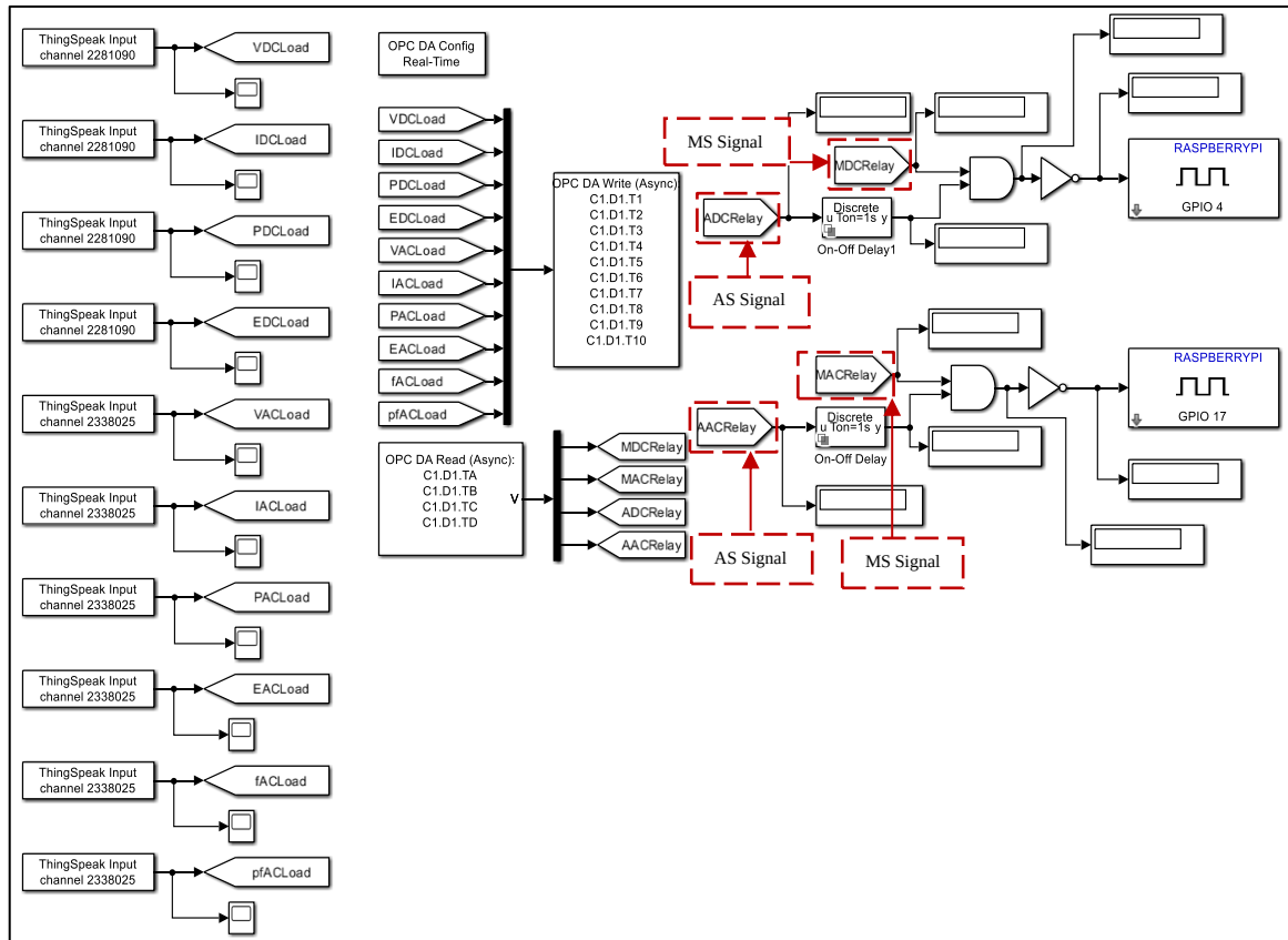
Figure D-5: MATLAB Communication Framework for Hardware Prototype
