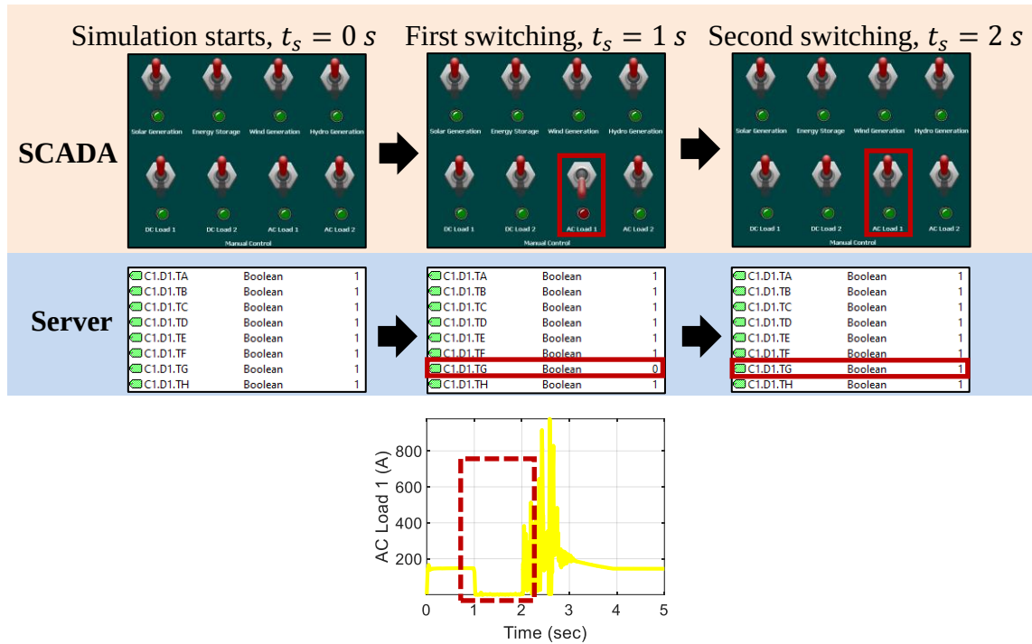
Figure 4.28: Manual Control of AC Load 1
