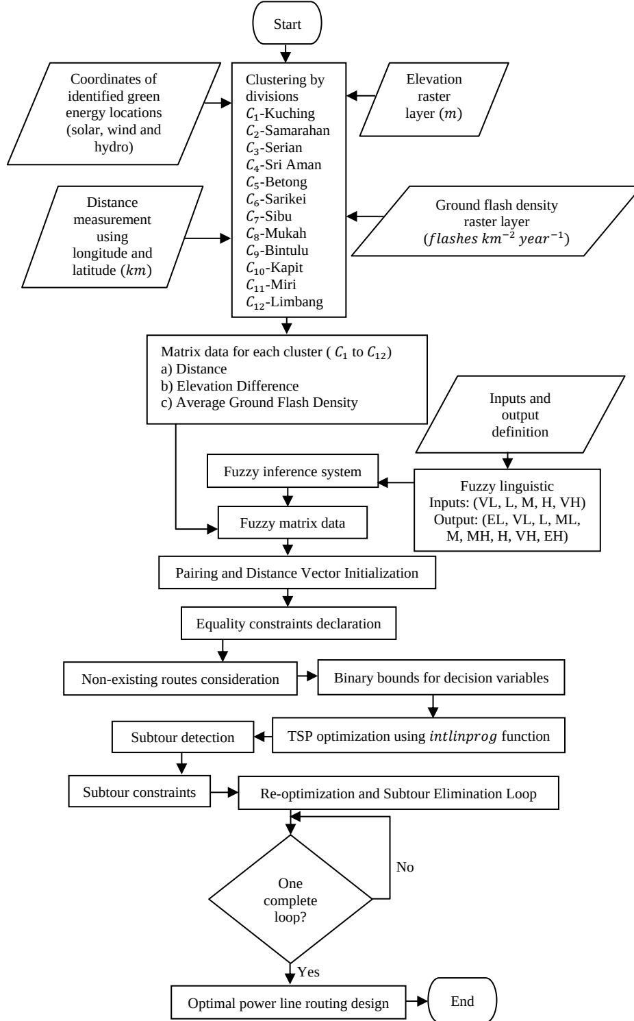
Figure 3.8: Flowchart of Proposed GIS-driven Fuzzy TSP-BIP Algorithm
