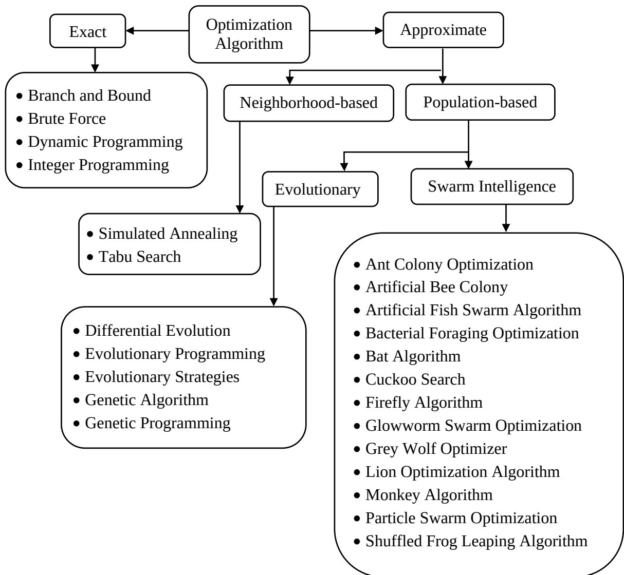
Figure 2.1: Overview of Optimization Algorithms
