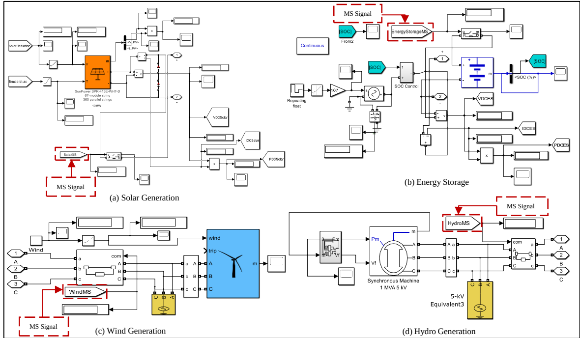
Figures D-3 (a) to (d): Integration of Manual Switches with Signal Channels into Green Energy Generations and Energy Storage Systems
