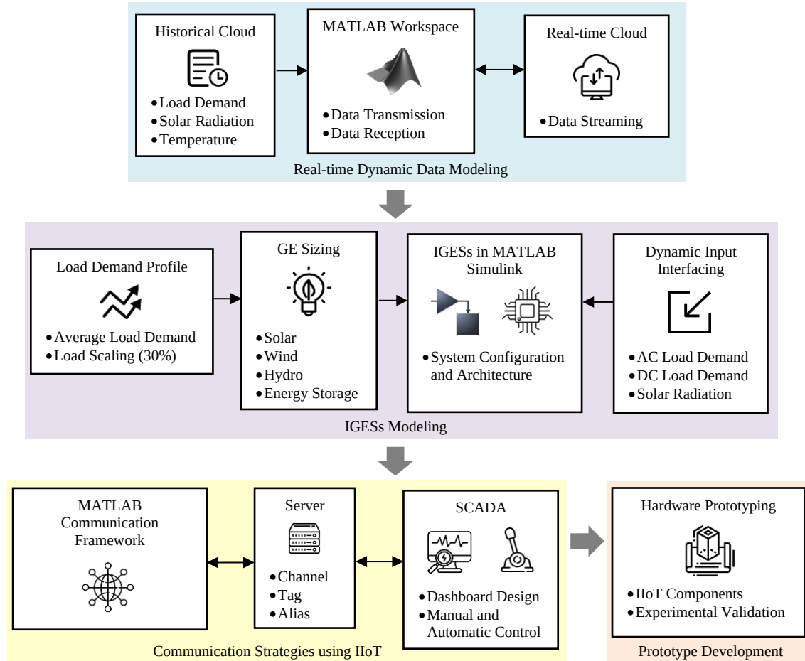
Figure 3.18: Block Diagram of Proposed IIoT-based System for IGESs
