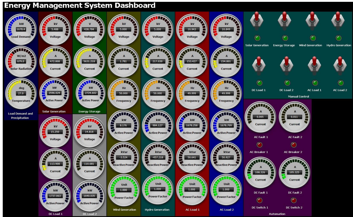
Figure 4.26: Monitoring Data at 2.5 s in SCADA
