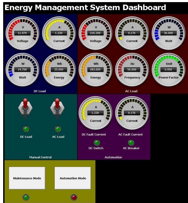
Figure 4.36: Monitoring Data on Actual Loads at 3.0 s in SCADA
