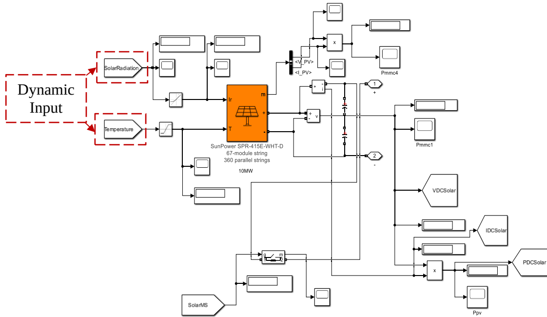
Figure 3.24: Dynamic PV Panel Modeling
