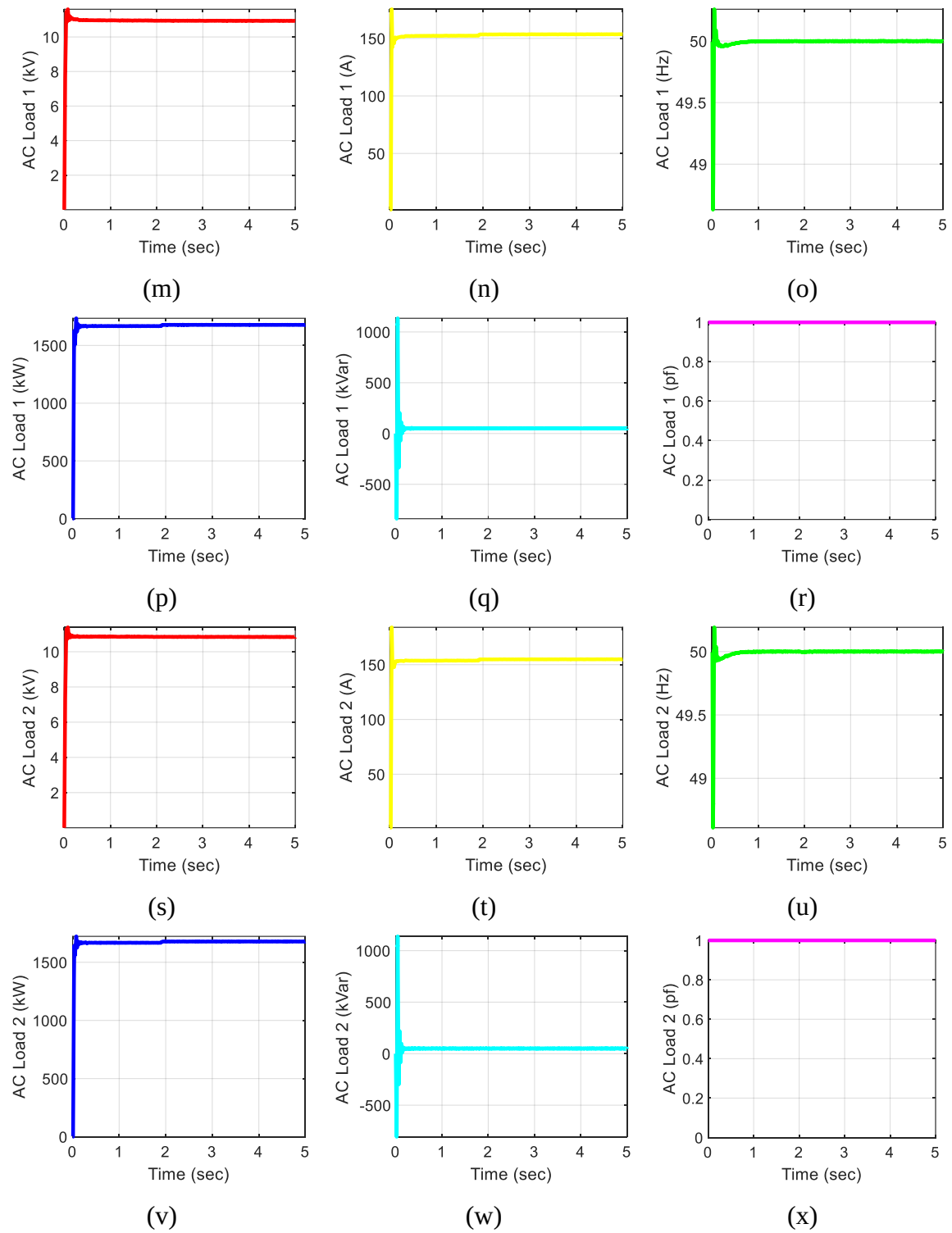
Figure 4.24 (a) to (x): Monitoring Data on Wind Generation, Hydro Generation, AC Load 1 and AC Load 2
