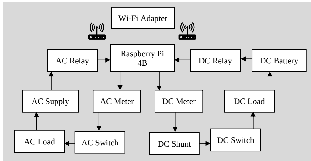
Figure 3.31: Hardware Prototype Development
