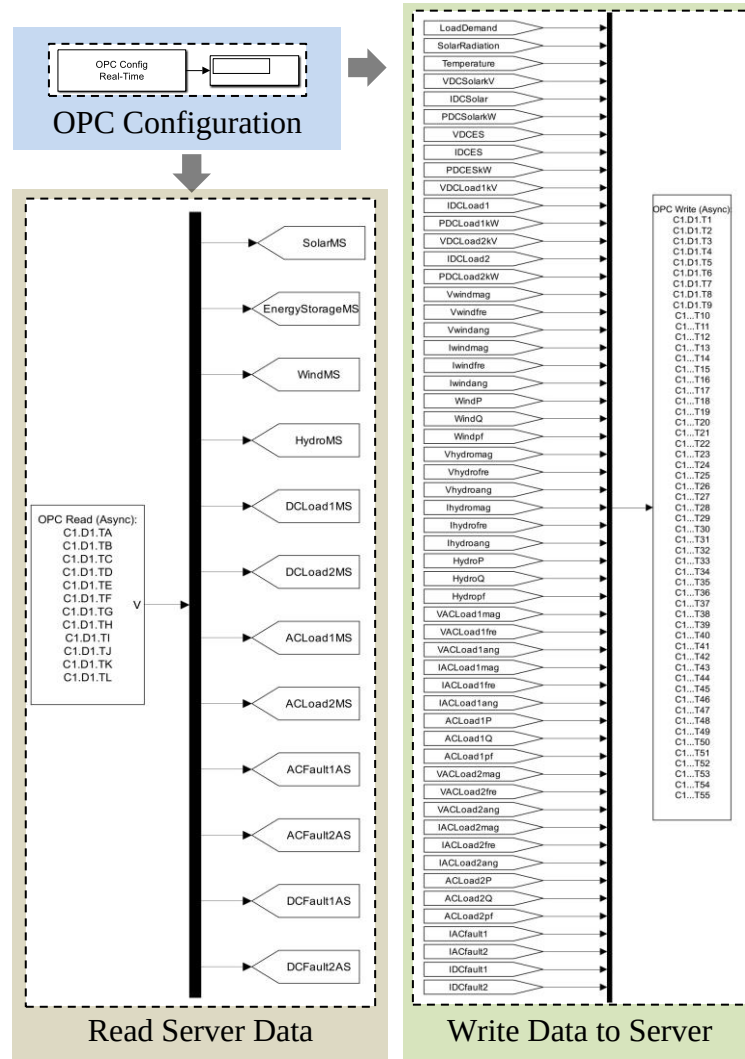
Figure 3.27: OPC Framework in MATLAB Simulink
