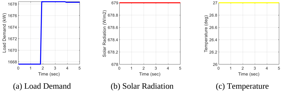
Figure 4.22 (a) to (c): Monitoring Data on Load Demand, Solar Radiation and Temperature
