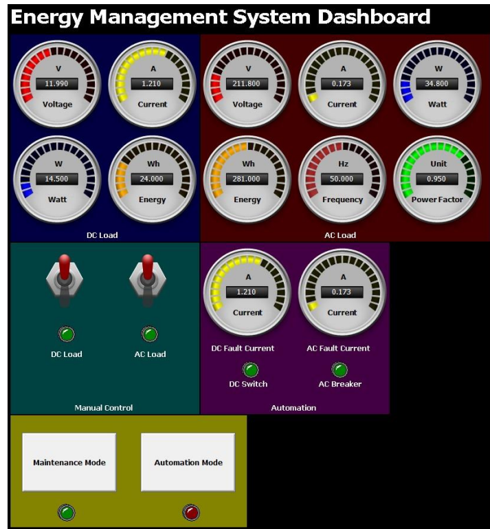
Figure 4.35: Monitoring Data on Actual Loads at 1.5 s in SCADA
