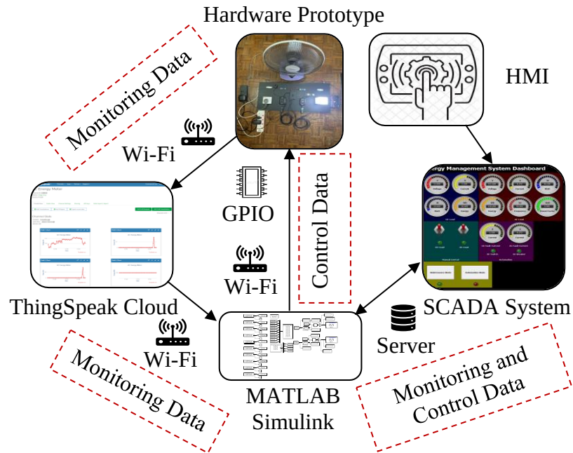
Figure 3.30: Operational Workflow of Hardware Prototype
