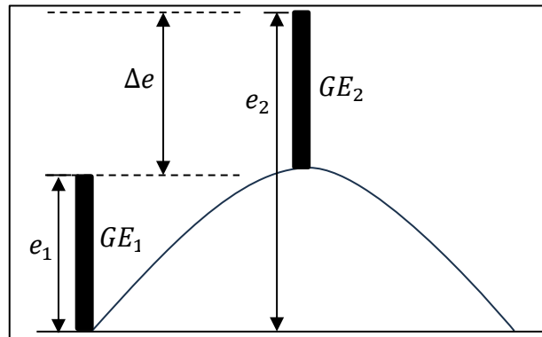
Figure 3.10: Measurement of Elevation Difference
