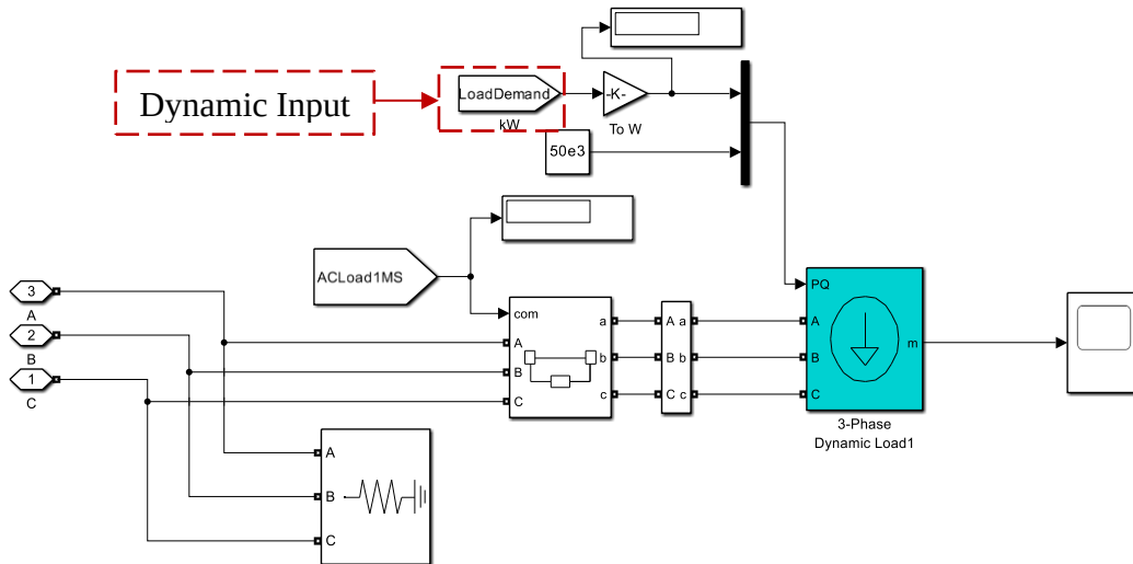
Figure 3.22: Dynamic AC Load Modeling
