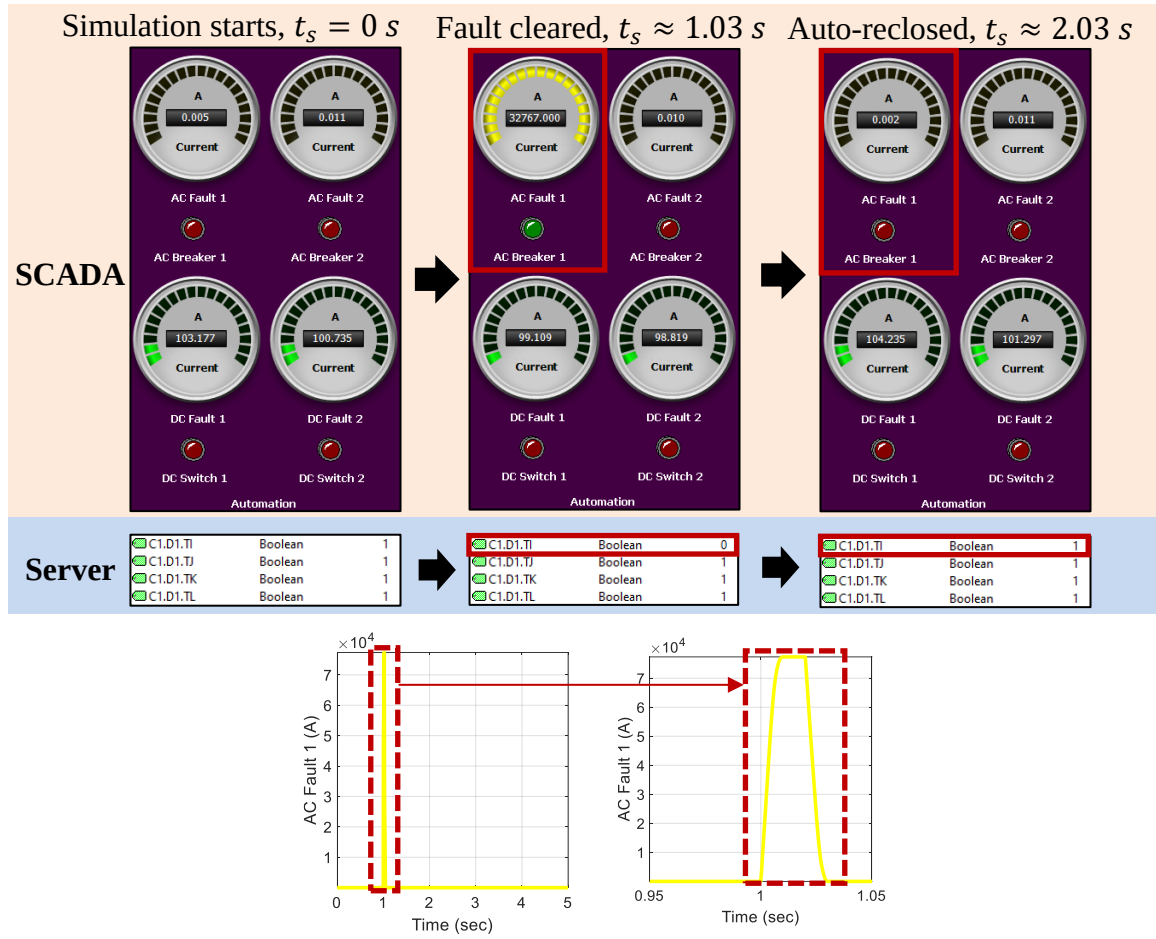
Figure 4.30: Automation Process for Clearing AC Fault 1
