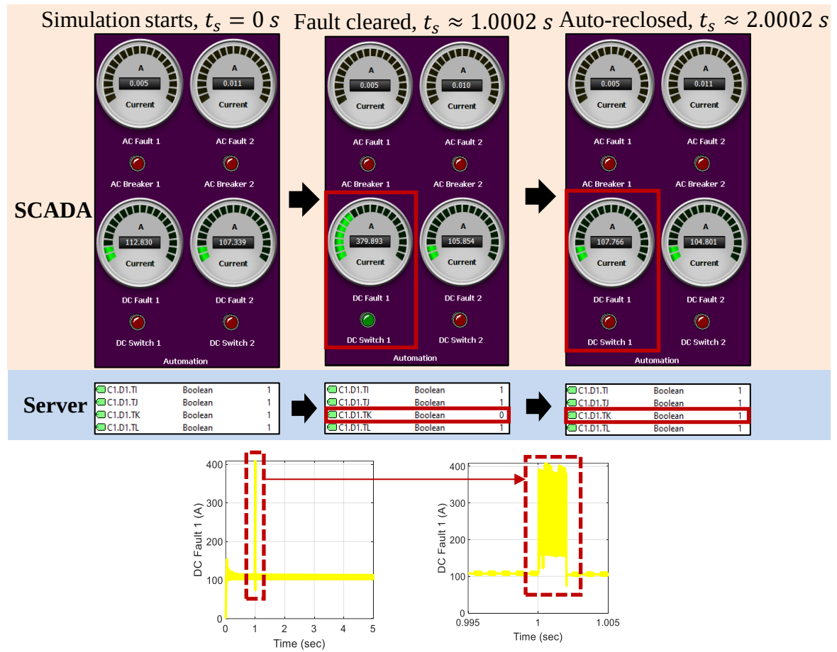
Figure 4.31: Automation Process for Clearing DC Fault 1
