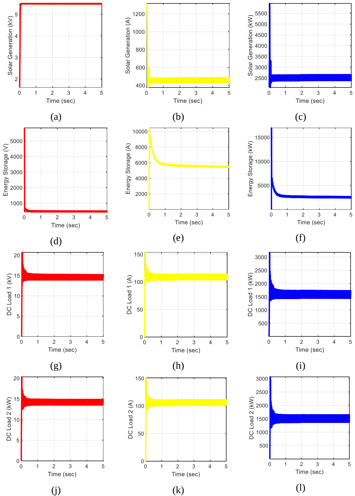
Figure 4.23 (a) to (l): Monitoring Data on Solar Generation, Energy Storage, DC Load 1 and DC Load 2
