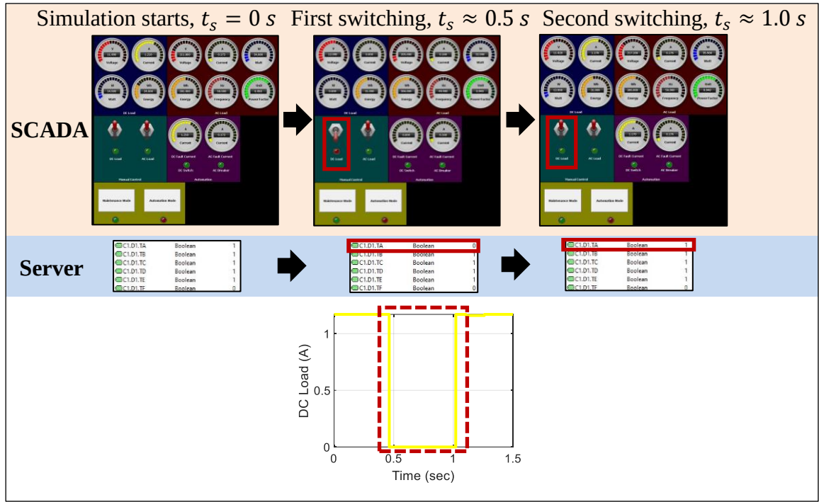
Figure 4.38: Manual Control of Actual DC Load
