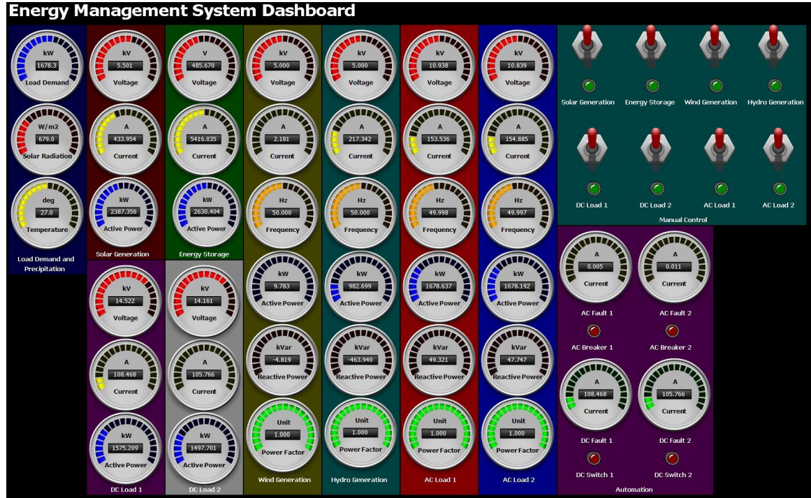
Figure 4.27: Monitoring Data at 5.0 s in SCADA
