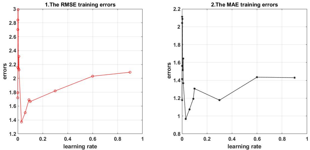
Figure 4.6: The Model Training Errors Based on Different Initial Parameter Learning Rate
