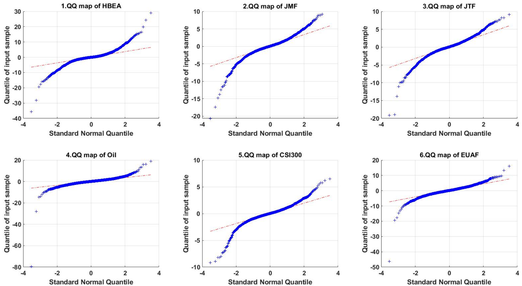
Figure 4.3: Q-Q Distribution of Carbon Price and its Infected Market Prices
