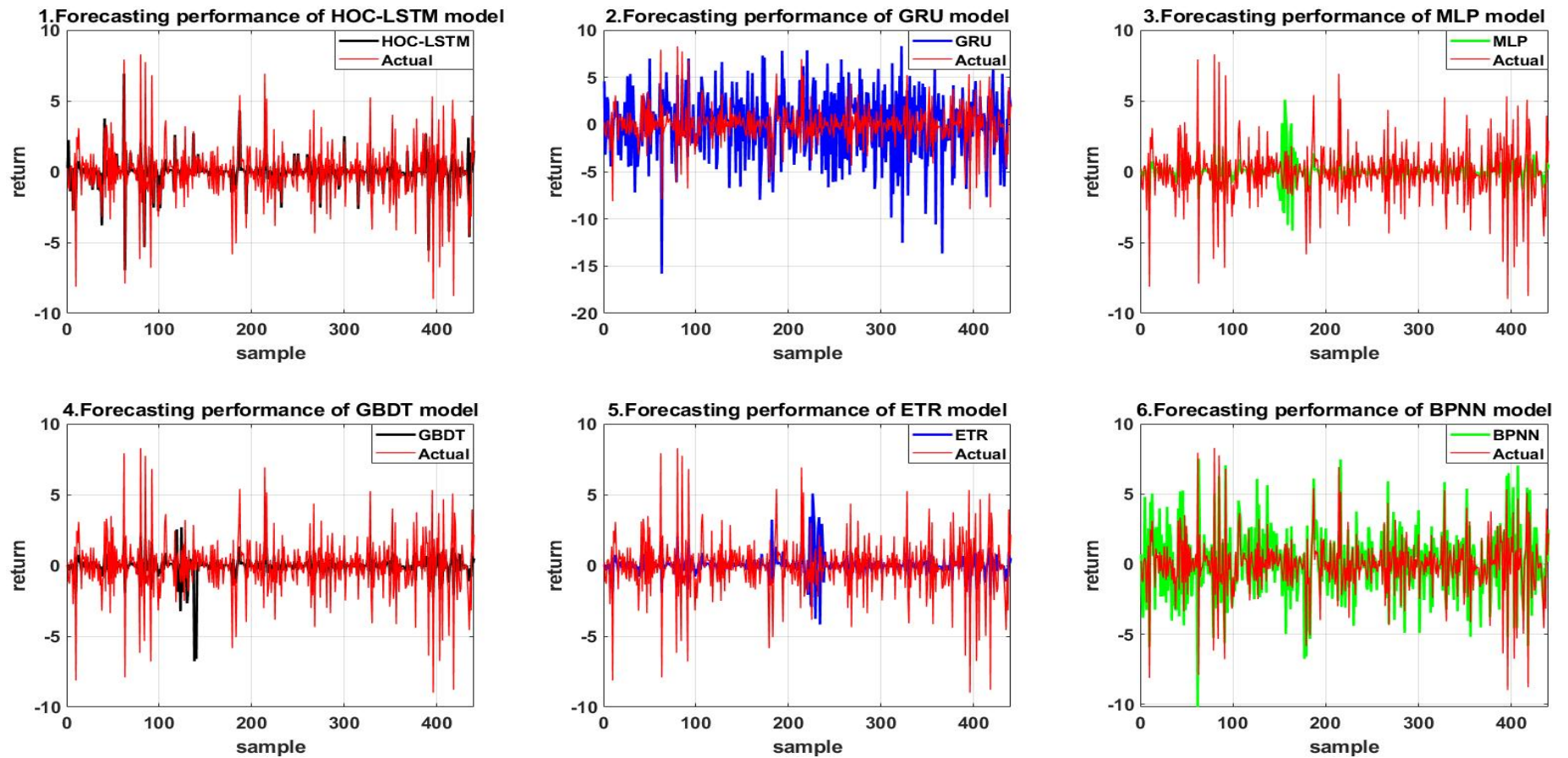
Figure 4.8: The China Carbon Price Out-of-Sample Forecasting Curve Based on the Impact of High Order Risk Contagion (The 20% Testing Sample of HOC-LSTM Model and its Comparative Models)
