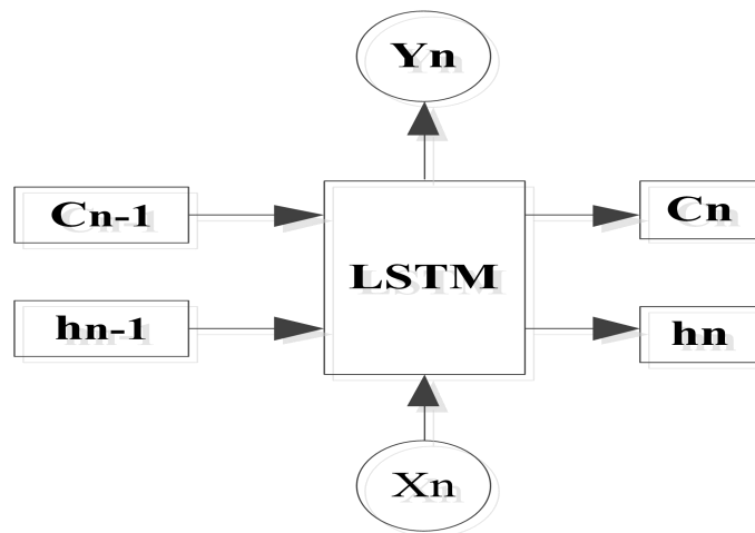
Figure 3.3: The Structure of LSTM
