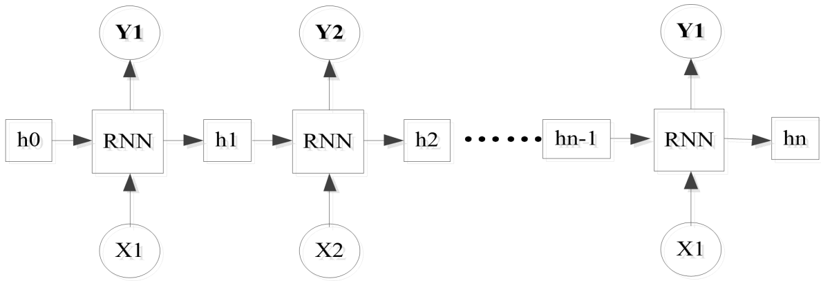
Figure 3.2: The Structure of RNN
