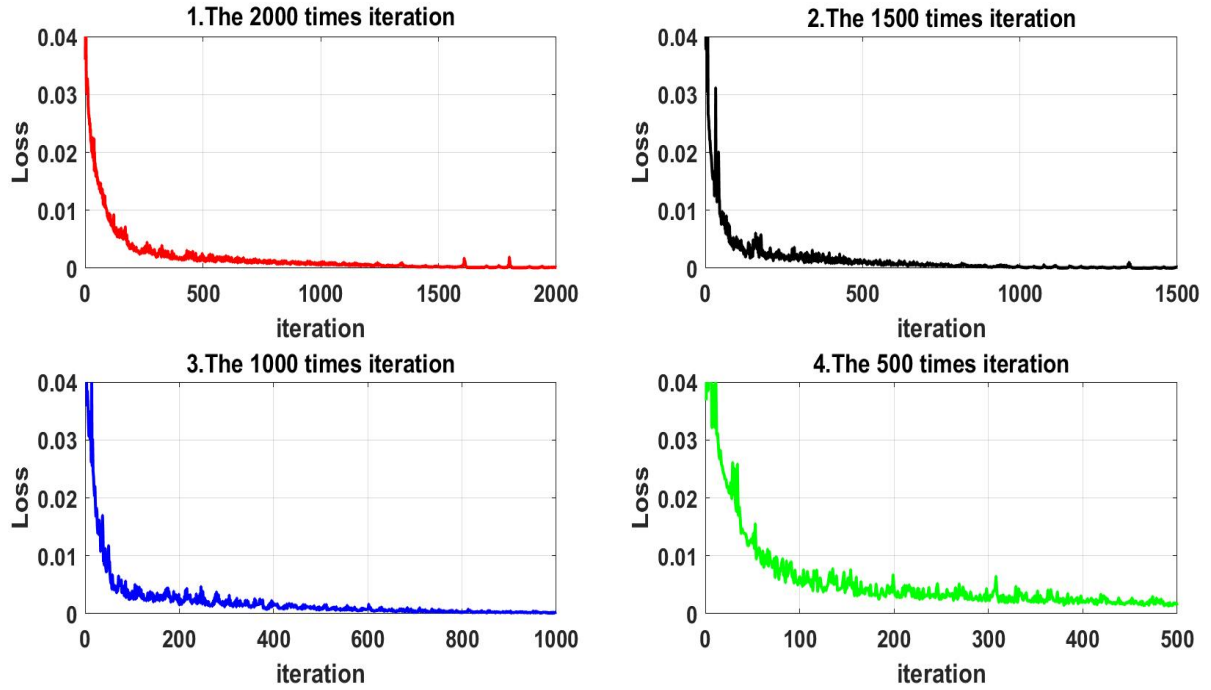
Figure 4.5: The Model Convergence Errors in Different Iteration Times
