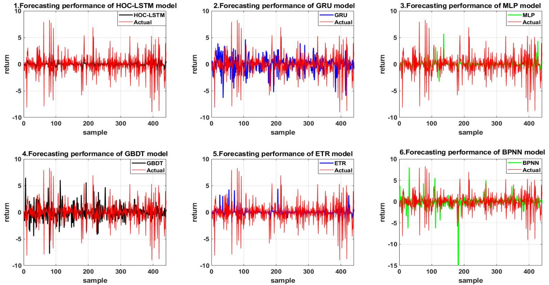
Figure 4.10: The China Carbon Price Out-of-Sample Forecasting Curve that Without Impact of High Order Risk Contagion (The 20% Testing Sample of HOC-LSTM Model and its Comparative Models)
