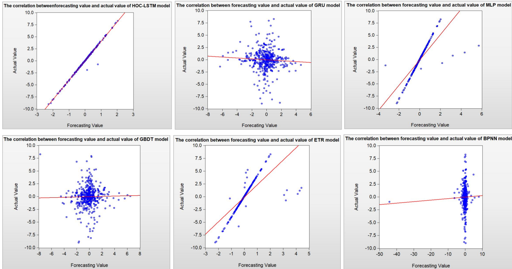
Figure 4.11: The Correlation Between Forecasting Value and Actual Value Without Impact of High Order Risk Contagion (The 20% Testing Sample of HOC-LSTM Model and its Comparative Models)
