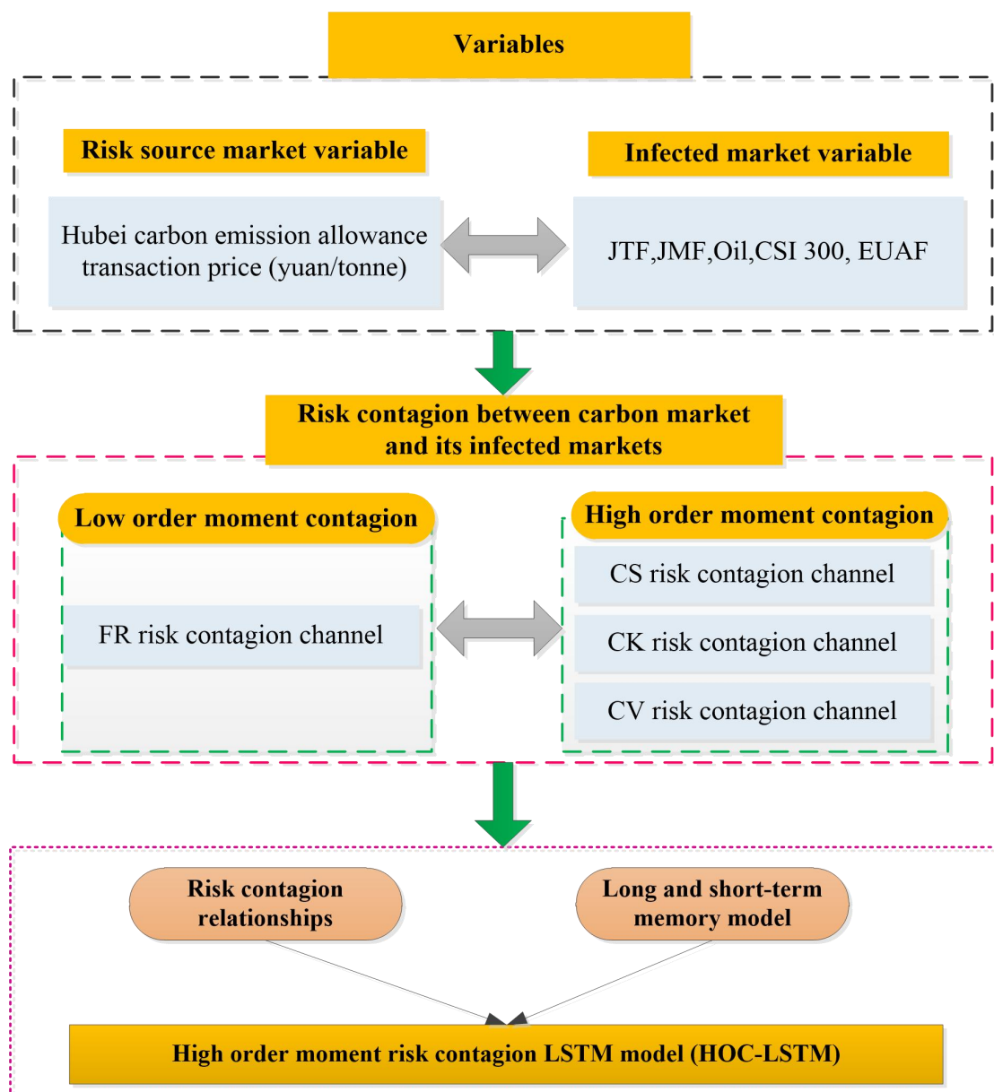
Figure 3.1: The Theoretical Framework of Methodology
