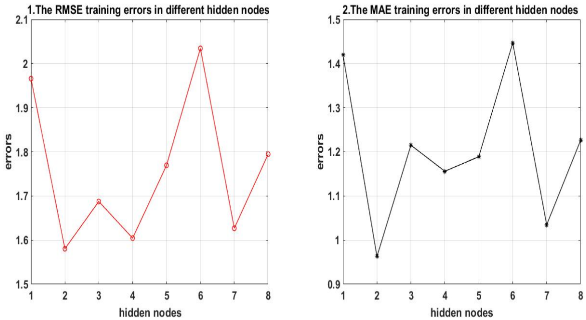
Figure 4.7: The Training Errors on Different Hidden Layers Nodes of HOC-LSTM
