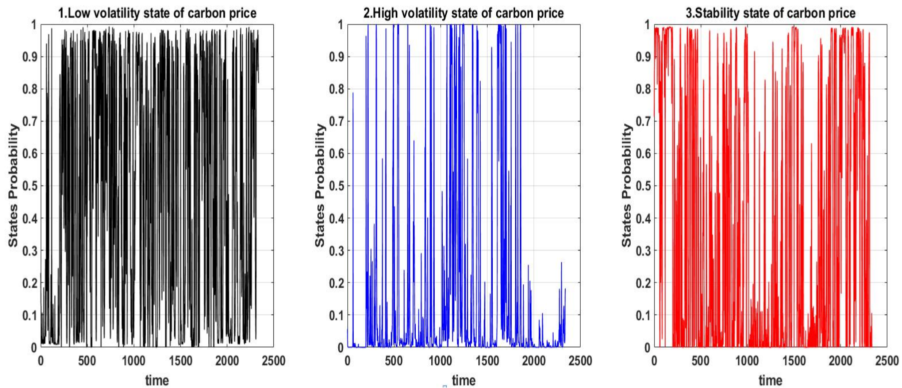
Figure 4.4: Smooth Probability Curve of the Three Volatility State Recognized by the MS(3)-AR(1) Model
