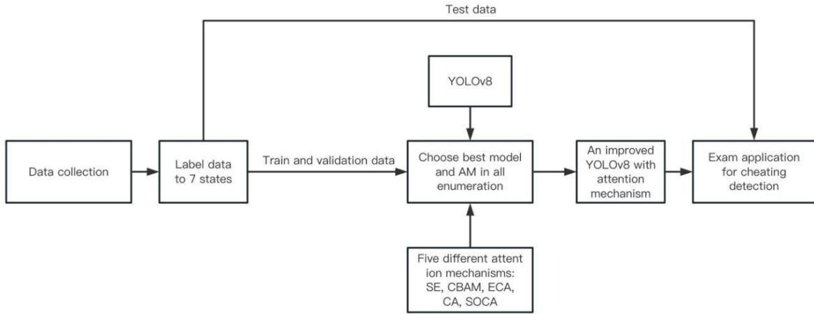
Figure 3.1: Methodology of the study
