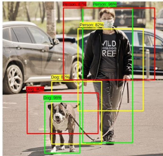
Figure 2.2: Right Bounding Box Using Non-Max Suppression
