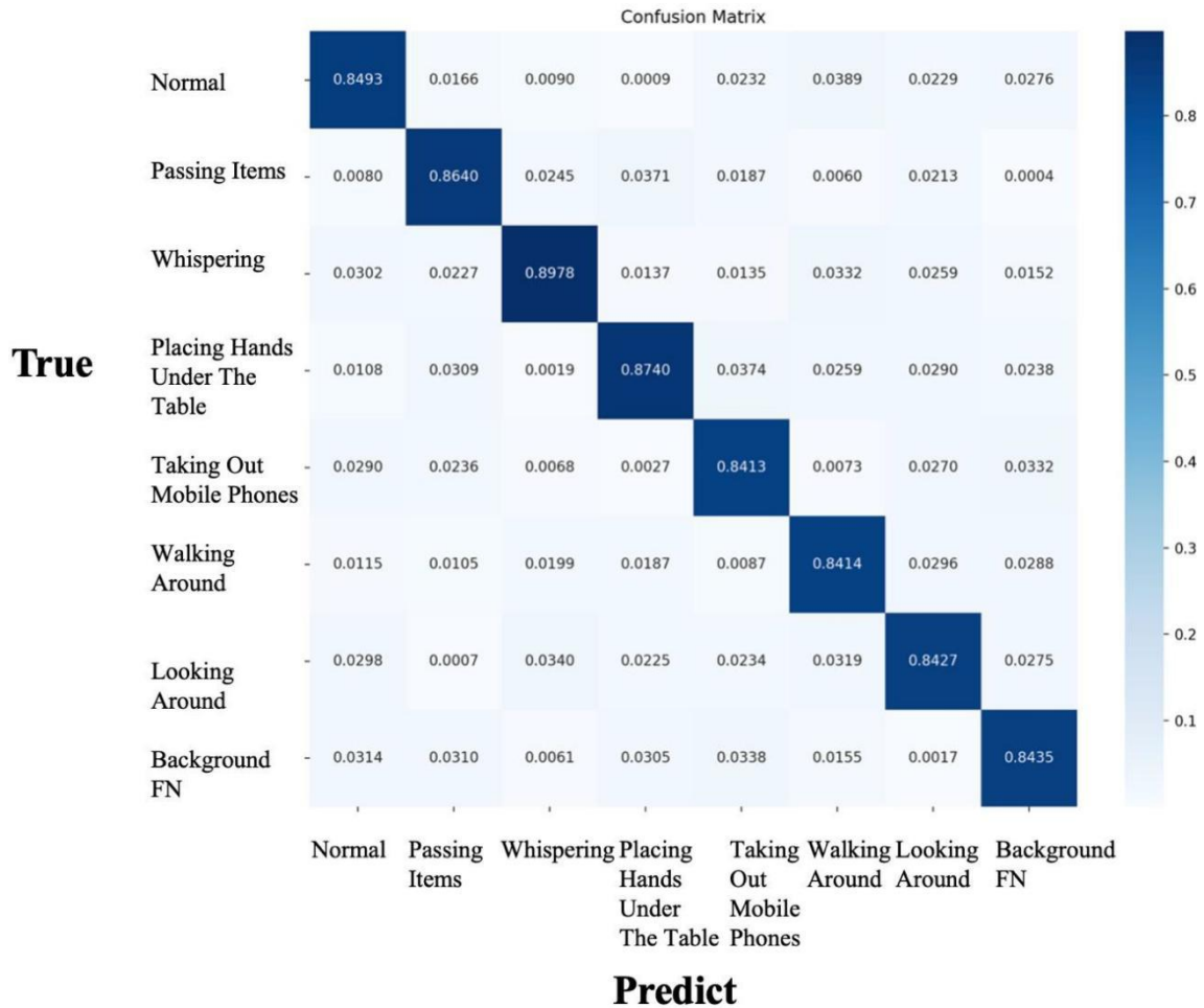
Figure 4.2: Confusion matrix of YOLOv8l-ECA
