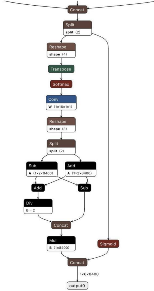
Figure 3.5: Detection head for YOLOv8
