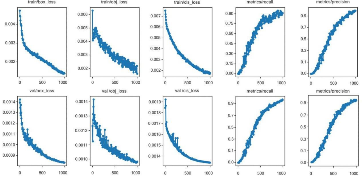
Figure 4.1: Training results of YOLOv8l-ECA
