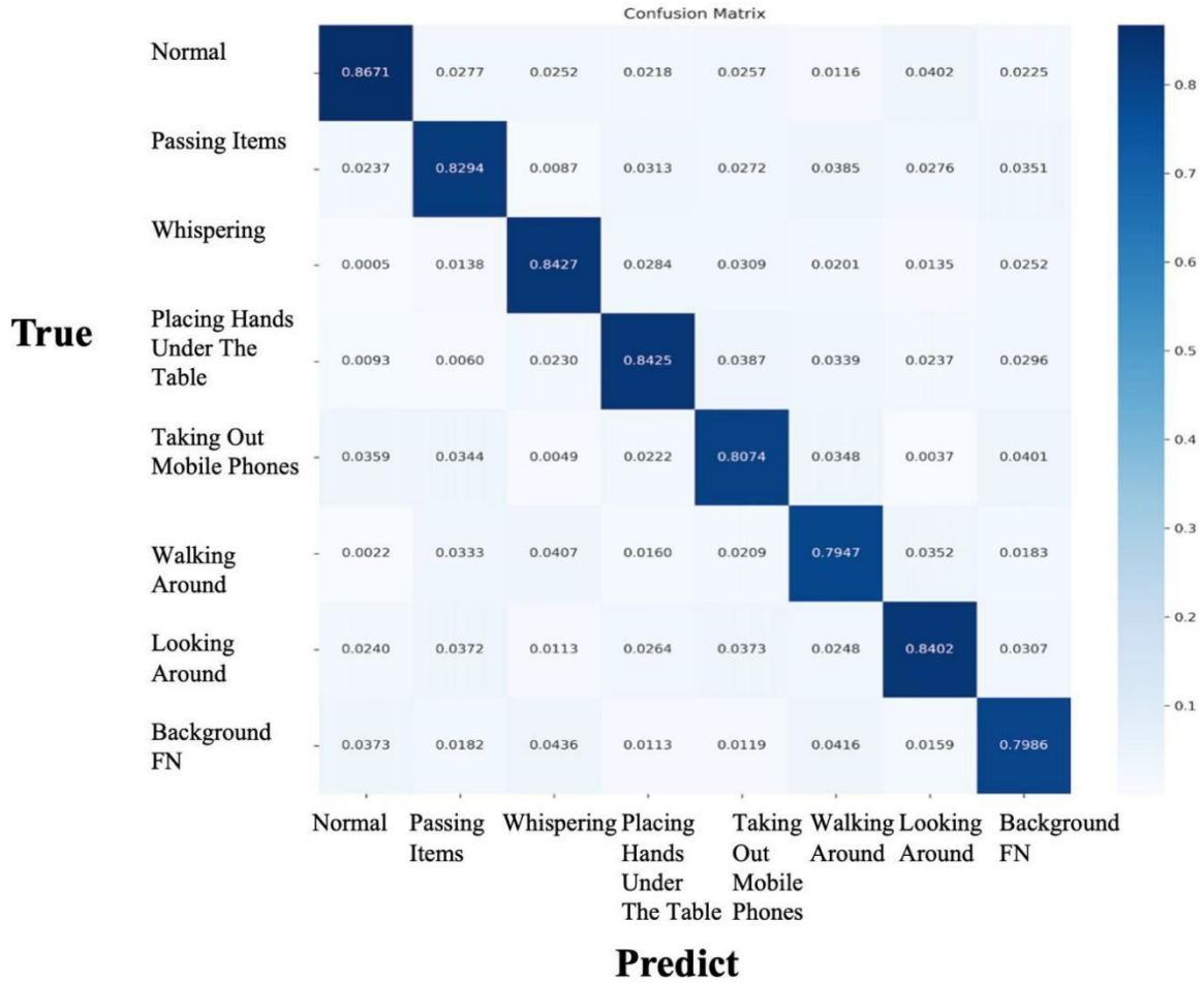
Figure 4.4: Test results of YOLOv8l-ECA
