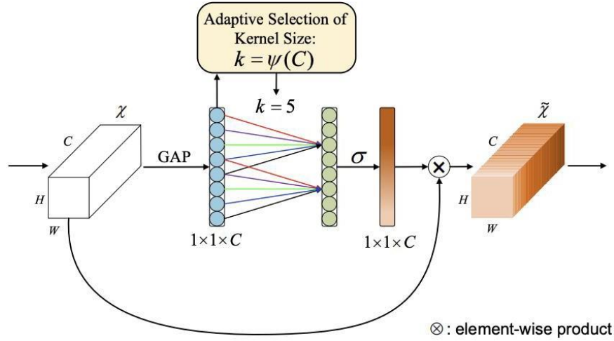
Figure 3.8: Diagram of the ECA module
