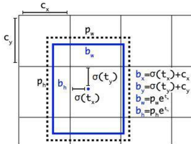
Figure 3.4: Visualization of an anchor box in YOLO (Solawetz, 2020)
