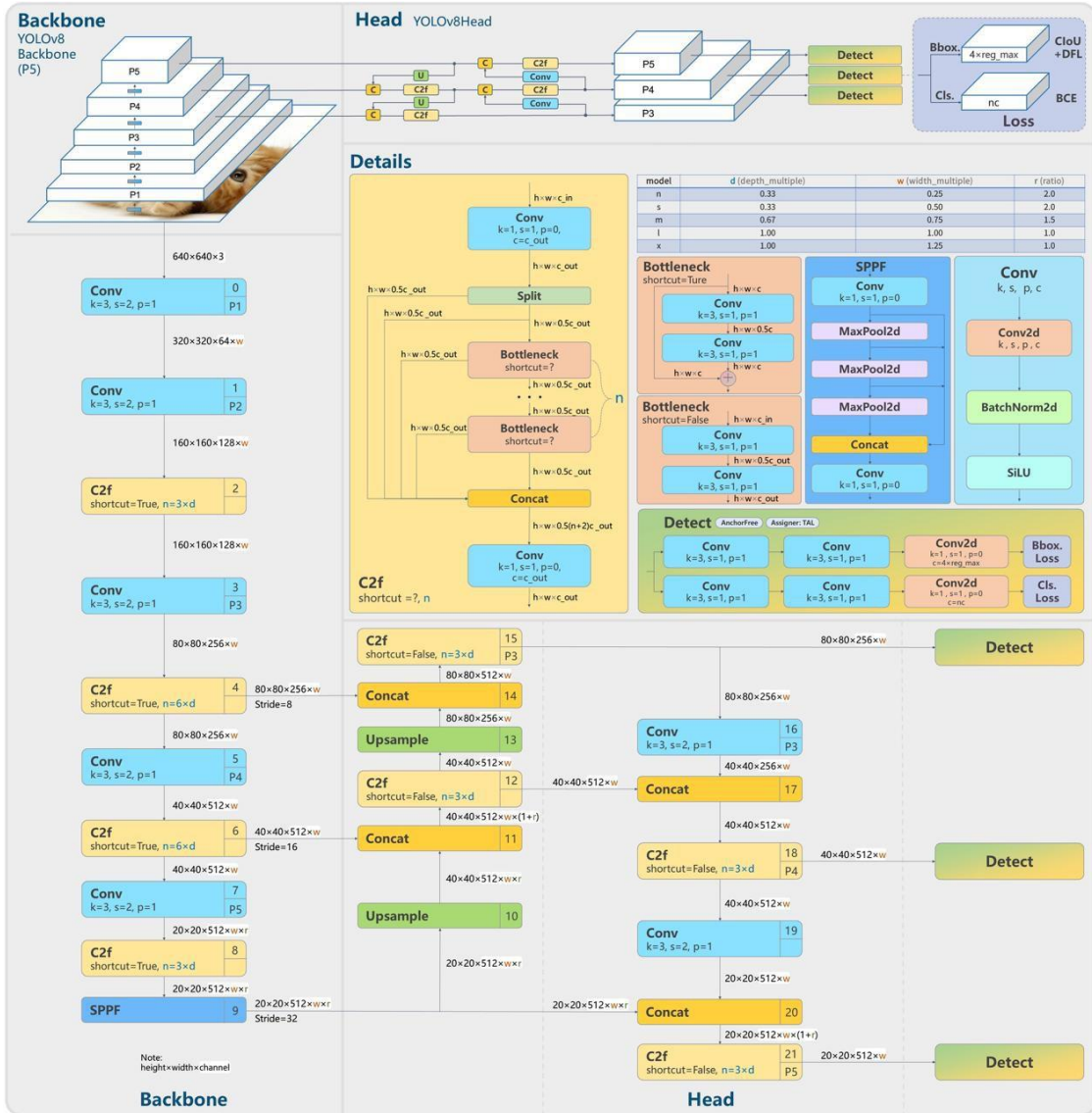
Figure 3.3: YOLOv8 architecture (Terven et al., 2023)
