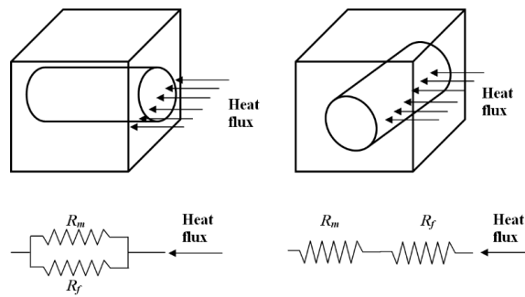
Figure 3.7: Thermal resistance model used to estimate thermal conductivity of FRP in axial and transverse direction (Pan & Hocheng, 1996)
