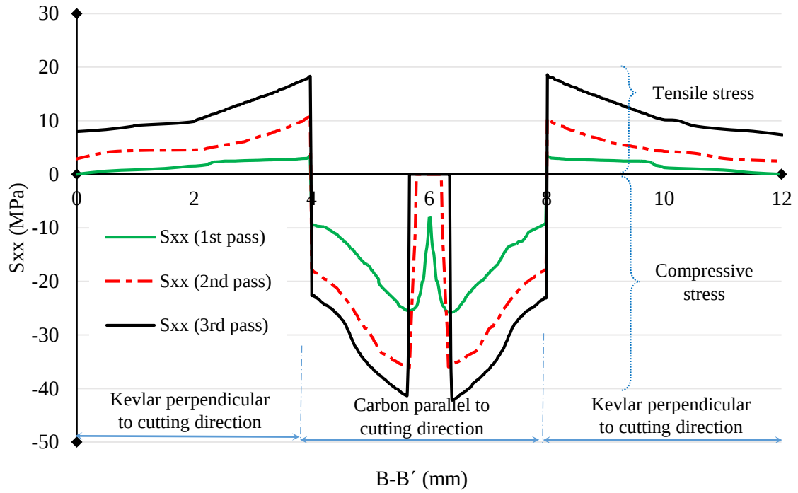
Figure 4.19: S_{xx} distribution along path B-B'
