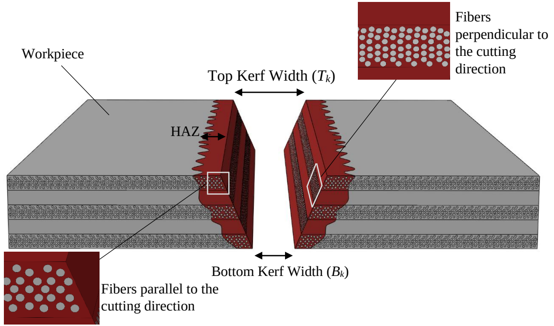
Figure 2.4: The schematic diagram of the composite laser cutting
