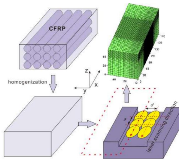
Figure 2.10: The schematic view of CFRP model and laser direction (Xu & Hu, 2017)
