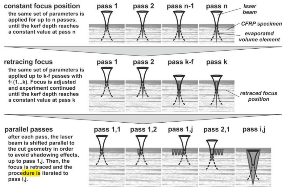
Figure 2.5: The schematic of three different methods for CFRP ablation (Herzog et al., 2016)
