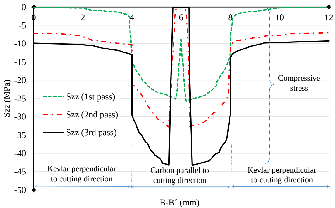
Figure 4.20: S_{zz} distribution along path B-B'
