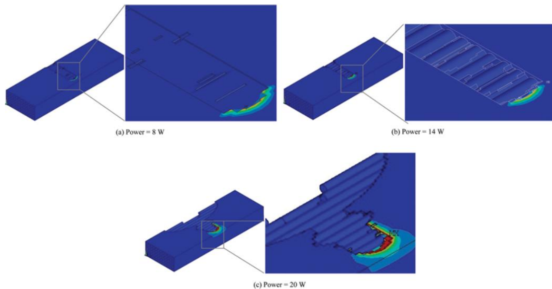
Figure 2.8: The effect of laser power on the ablation characteristics (Nattapat et al., 2015)
