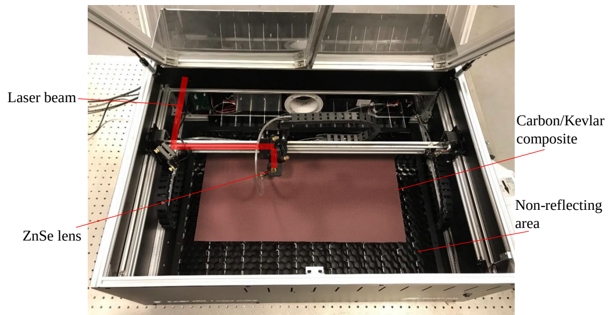
Figure 3.3: Cutting table
