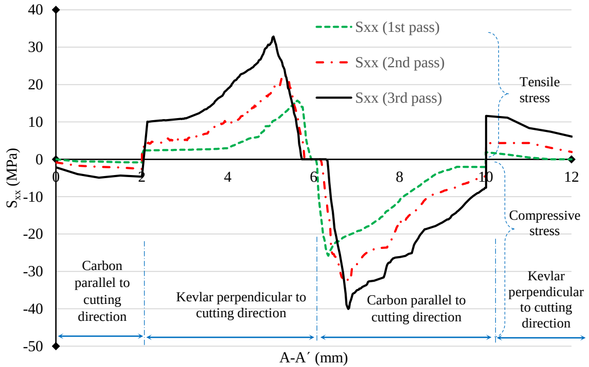
Figure 4.17: In-plane stress in x-direction ( S_{xx} ) along path A-A'
