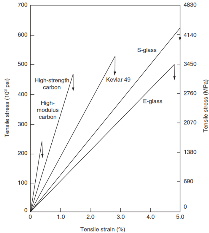
Figure 2.2: Comparison the strength of some fibers (Mallick, 2007)
