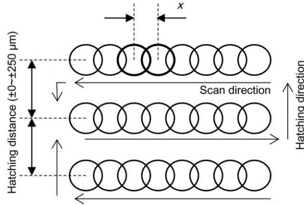
Figure 2.7: Definition of scanning direction and hatching distance (Takahashi et al., 2015)
