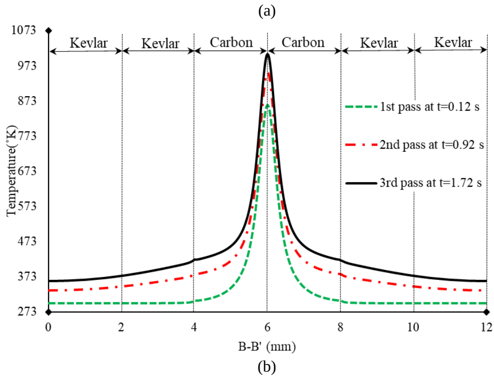
Figure 4.15: Temperature distribution along, (a) path A-A'; (b) path B-B
