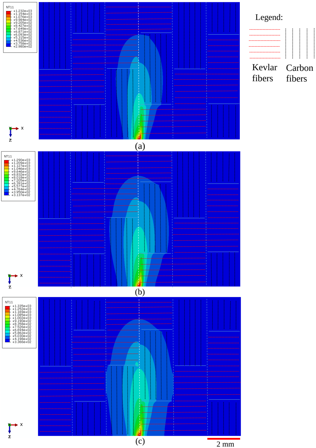
Figure 4.13: Temperature gradient for each laser pass, (a) 1 st pass (max temperature = 1232°K, t = 0.24 s); (b) 2 nd pass (max temperature = 1290°K, t = 1.04 s); (c) 3 rd pass (max temperature = 1335°K, t = 1.84 s)
