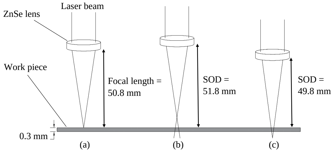
Figure 3.4: Schematic diagram of focal plane position and standoff distance with regard to the surface of the work piece
