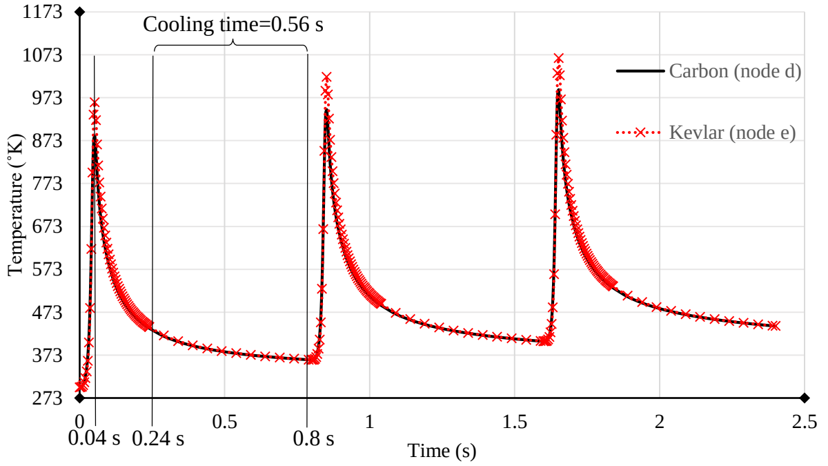
Figure 4.14: Temperature histories of specific nodes (d & e) for cutting parameters: power= 37.6 W and speed= 25 mm/s
