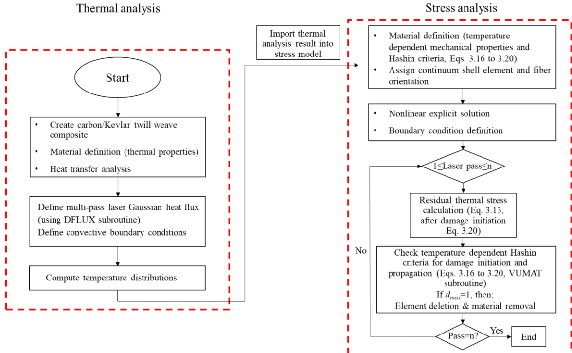
Figure 3.10: Analysis procedure for the modelling in Abaqus
