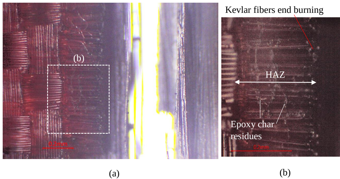
Figure 4.10: (a) The cutting area of optimum laser parameters; (b) less heat affected zone of cutting area and fibers burning
