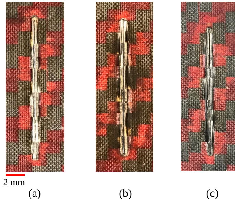
Figure A: Samples of laser cutting at different regions of carbon/Kevlar composite (experiment standard order No. 1)
