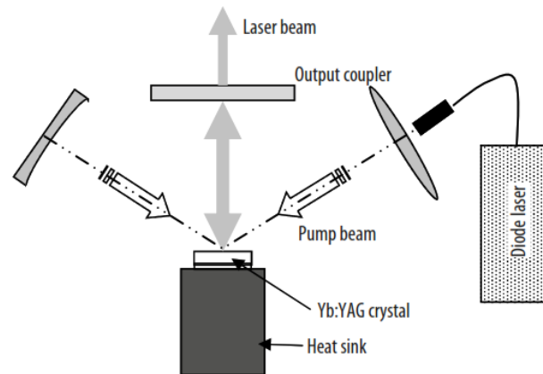
Figure 2.3: The schematic of a disk laser (Steen & Mazumder, 2010)
