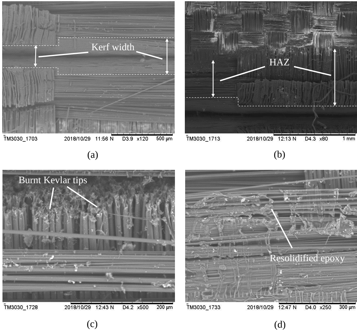
Figure 4.8: The effect of bidirectional fiber orientation on, (a) kerf width; (b) HAZ extent; (c) Kevlar fibers; (d) epoxy matrix. Sample of experiment standard no. 4
