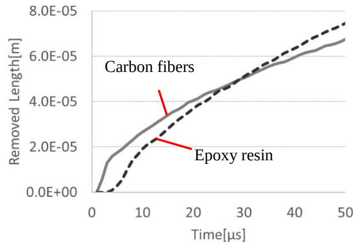
Figure 2.11: Removed length for both fiber and resin (Ohkubo et al., 2017)
