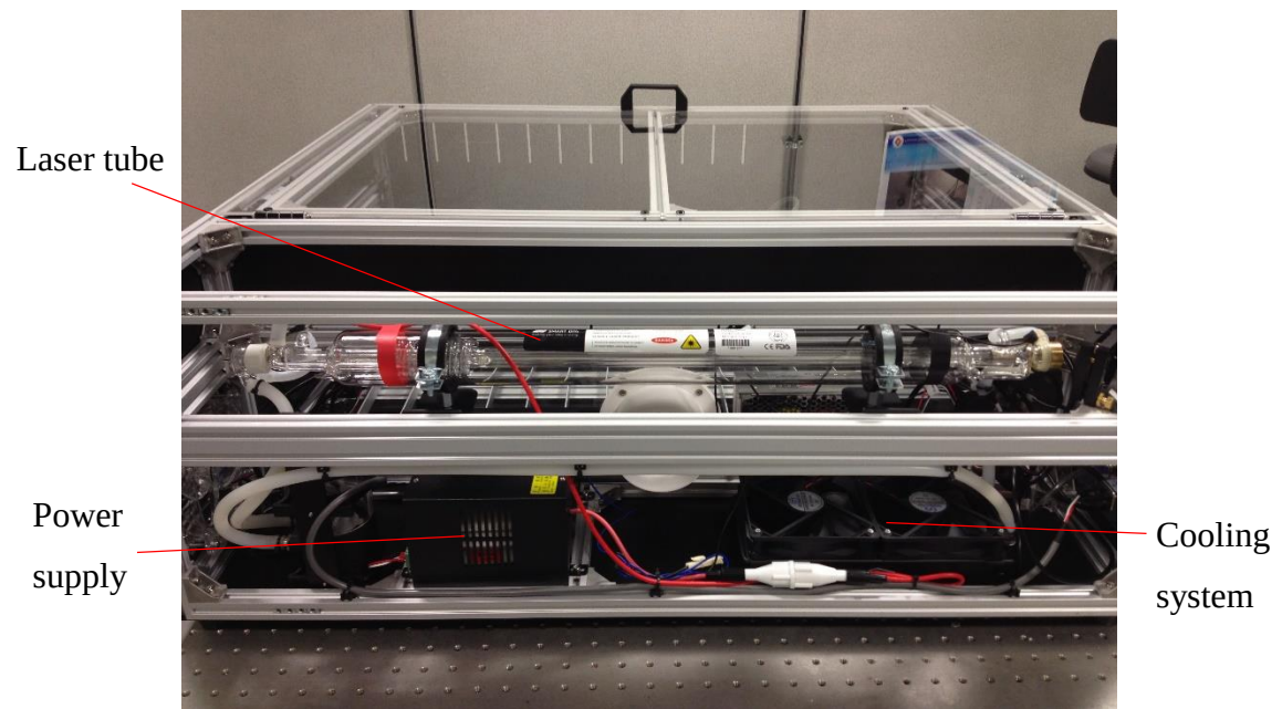
Figure 3.2: CO 2 laser system
