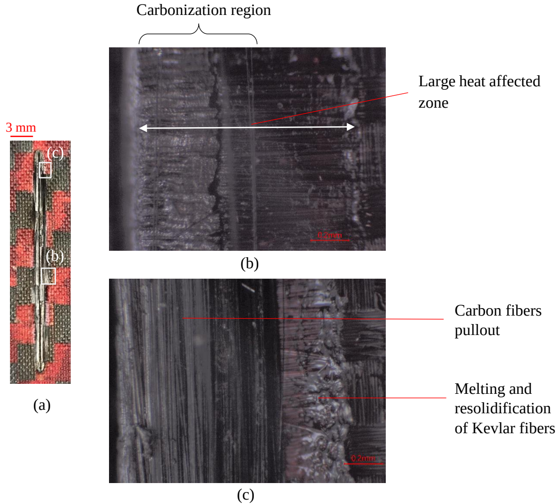
Figure 3.6: Optical micrographs, (a) a sample of laser cut (38 W, 5 mm/s and 50.8 mm SOD); (b) excessive carbonization and large HAZ; (c) carbon fibers pullout and melting of Kevlar fibers
