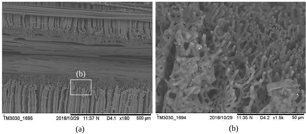
Figure 4.6: SEM micrographs of, (a) cutting area at 50.8 mm SOD; (b) enlarged Kevlar fibers. Sample of experiment standard no. 3
