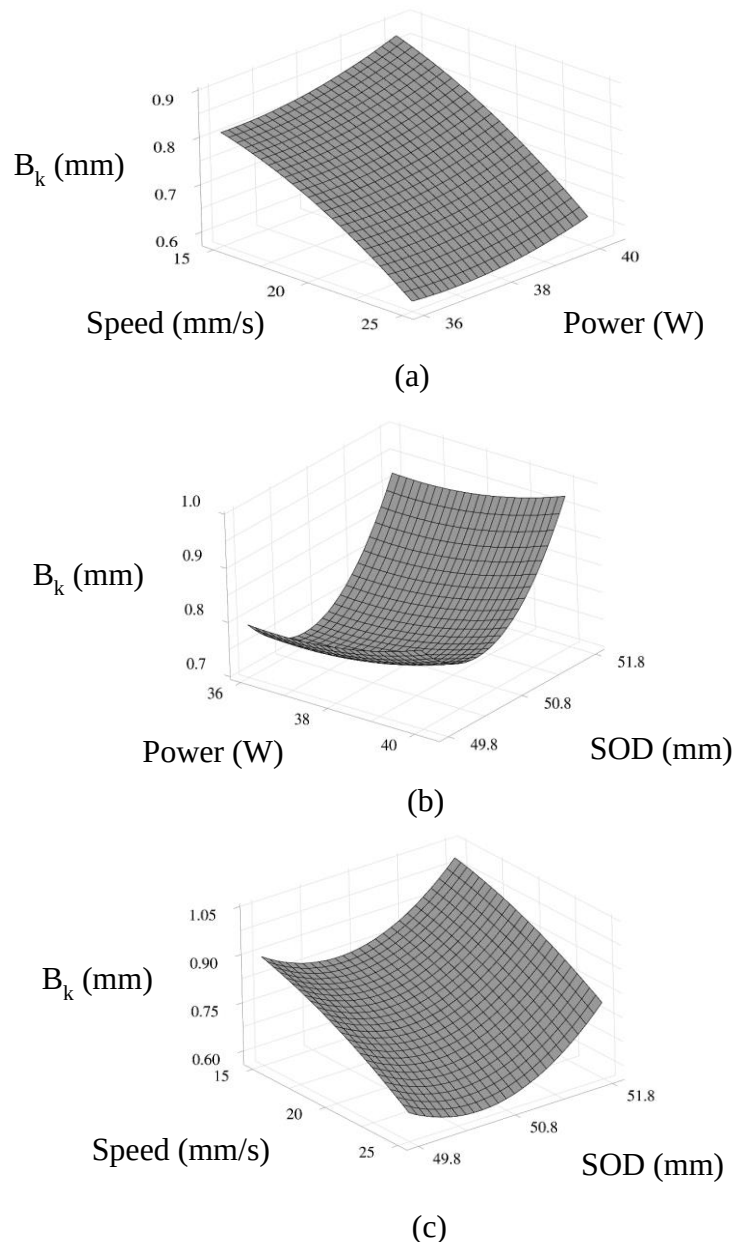
Figure 4.4: Response surface plots of bottom kerf width with respect to different combinations of the input process parameters, (a) power - speed; (b) power - SOD; (c) speed - SOD
