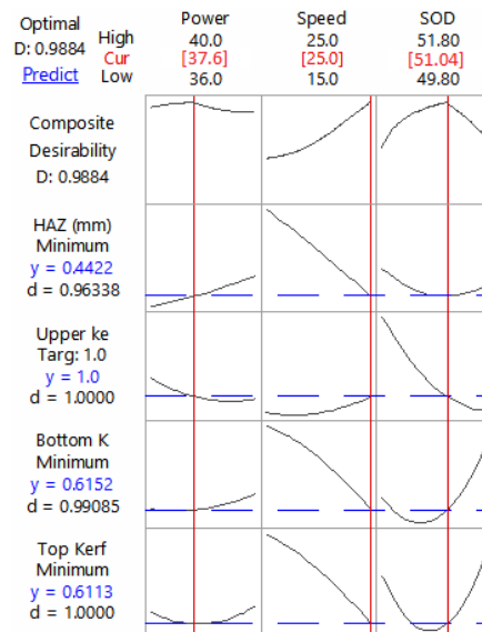
Figure 4.9: Optimum parameters of cutting and the predicted results of HAZ, top kerf width, bottom kerf width and kerf ratio
