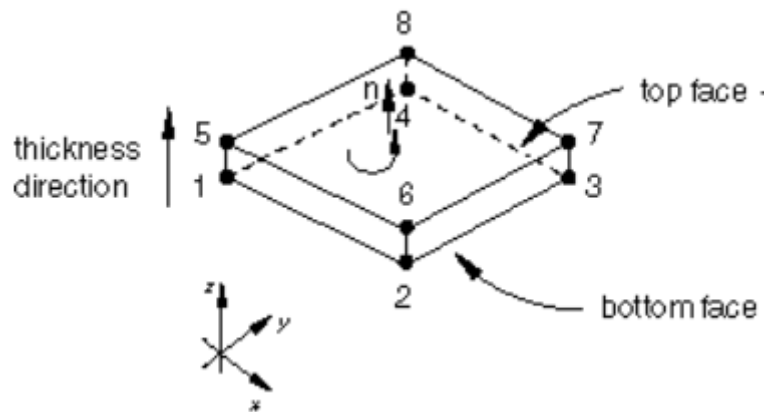
Figure 3.9: Normal and thickness direction for continuum shell element (SC8R) (Abaqus, 2014)
