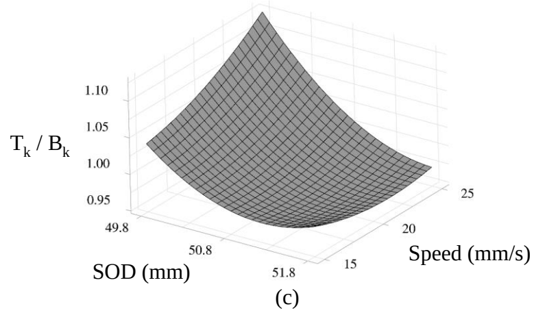
Figure 4.5: Response surface plots of kerf ratio with respect to different combinations of the input process parameters, (a) power – speed; (b) power – SOD; (c) speed - SOD
