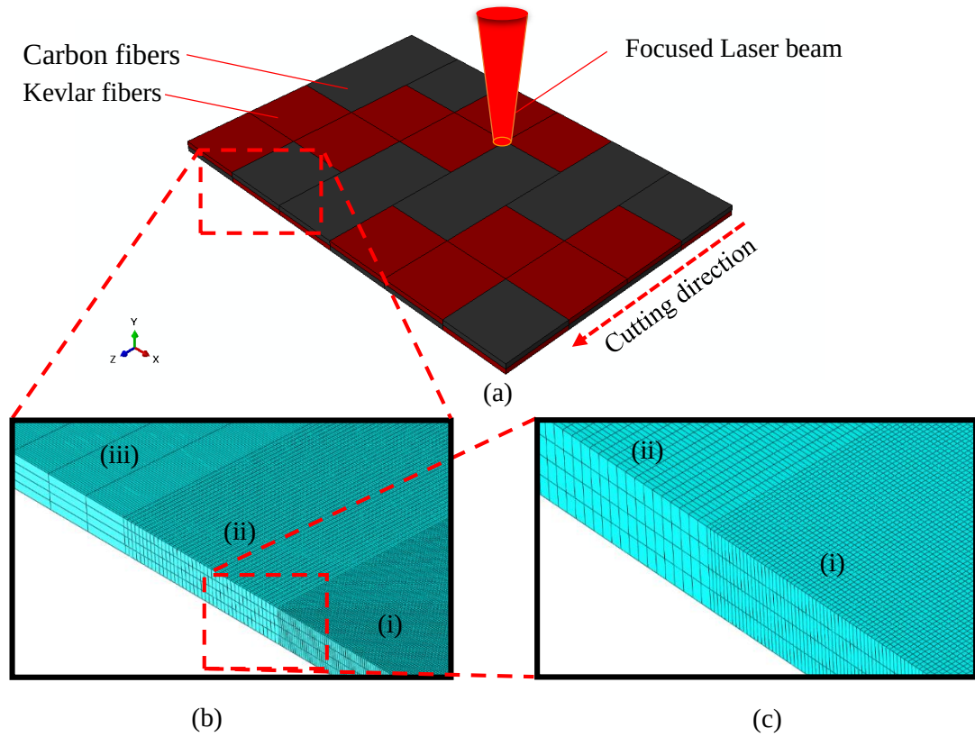
Figure 3.8: (a) The schematic view of carbon/Kevlar hybrid composite and laser position; (b) the mesh distribution perpendicular to cutting direction; (c) magnified image of denser mesh near cutting area
