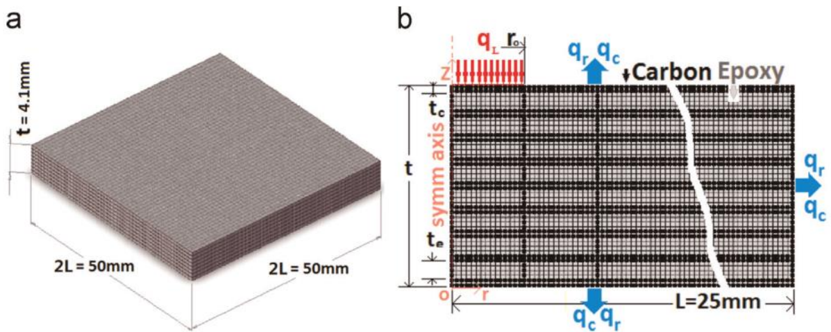
Figure 2.9: CFRP model and definition of thermal loads and boundary condition (Wu et al., 2015)
