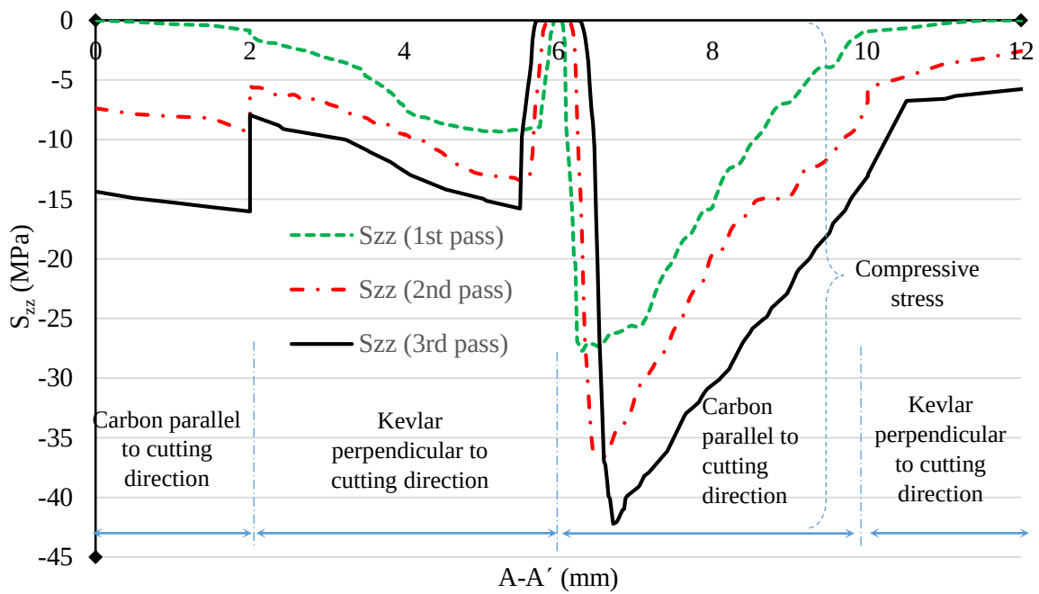
Figure 4.18: In-plane stress in z-direction ( S_{zz} ) along path A-A'
