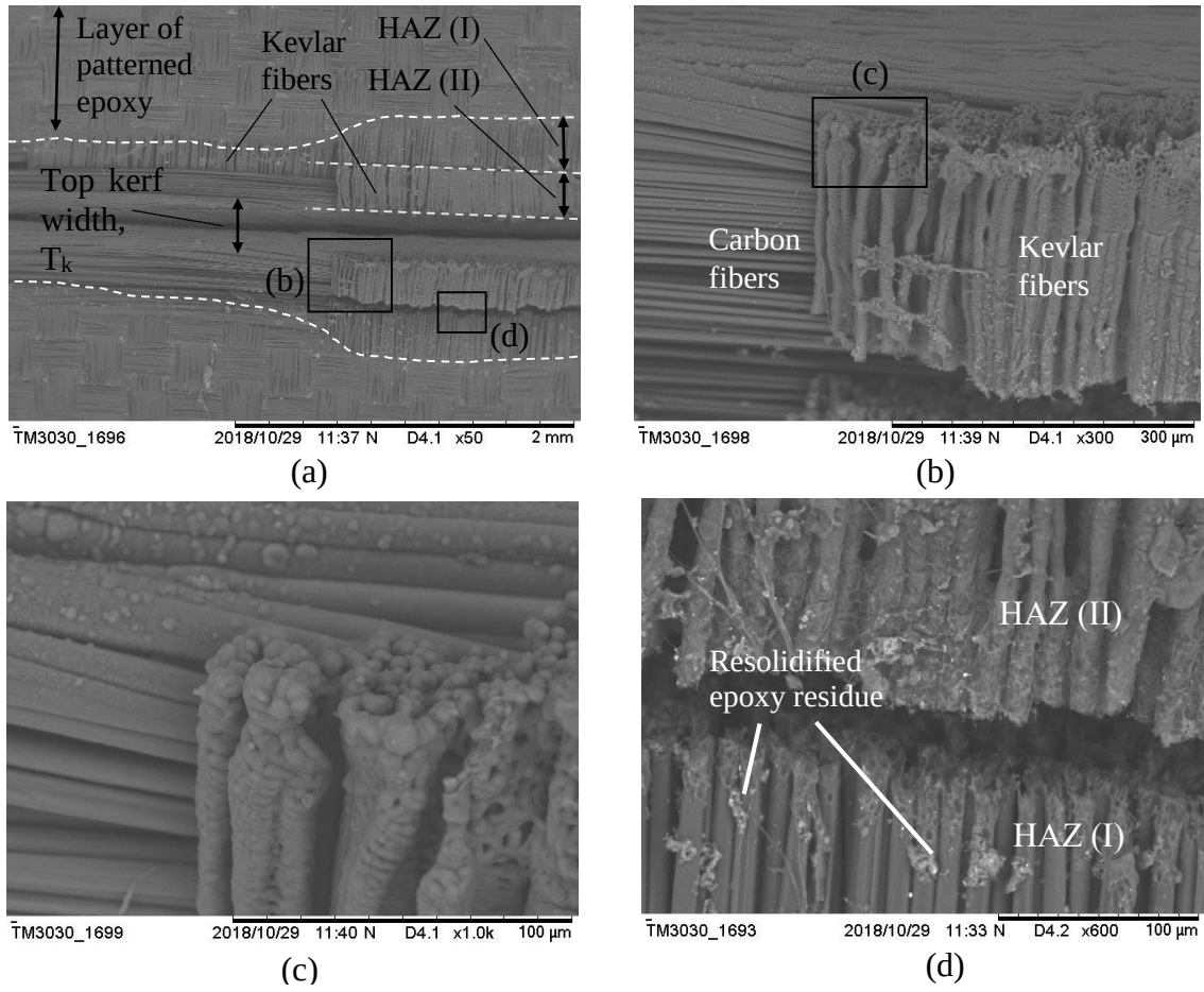
Figure 4.2: SEM micrographs of HAZ (experiment no. 4), (a) two dissimilar regions of heat affected zones; (b) completely burnt and separated Kevlar fibers; (c) swelling of burnt Kevlar fibers; (d) crack due to the brittle feature of charred Kevlar fibers
