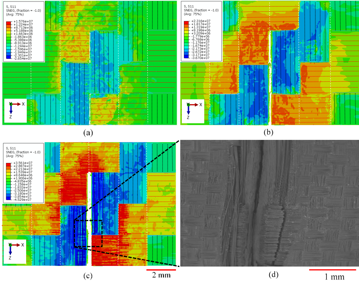
Figure 4.16: Element removal and residual thermal stress profile ( S_{xx} ); (a) 1 st pass, (b) 2 nd pass, (c) 3 rd pass, (d) SEM micrograph result from experiment after 3 rd pass
