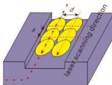
Figure 2.6: Characterization of laser scanning direction (Xu & Hu, 2017)
