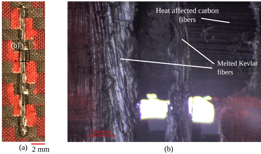
Figure 4.11: (a) Cutting area by moving the laser beam perpendicular to the carbon fibers; (b) remained heat affected carbon fibers and melted Kevlar fibers
