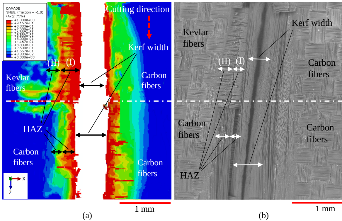
Figure 4.21: The effect of fiber orientation and thermal conductivity on HAZ and kerf width, (a) numerical simulation; (b) SEM micrograph from experiment
