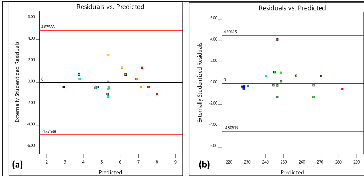
Figure 4.18: The residual versus predicted graph for first DoE (0% water, 100% methanol and 100% water, 0% methanol) (a) Tensile strength, (b) Young's modulus
