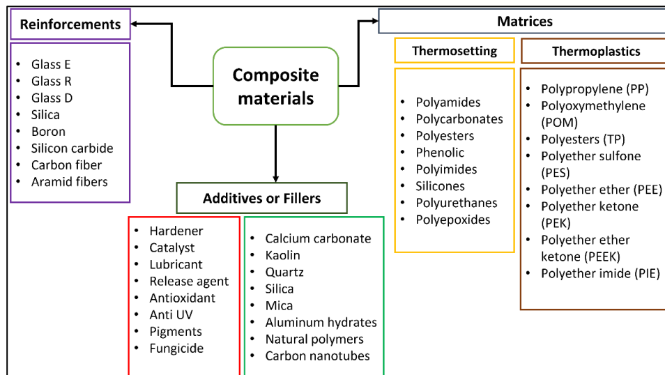
Figure 2.8: The formulation of composite materials (Hsissou et al., 2021)
