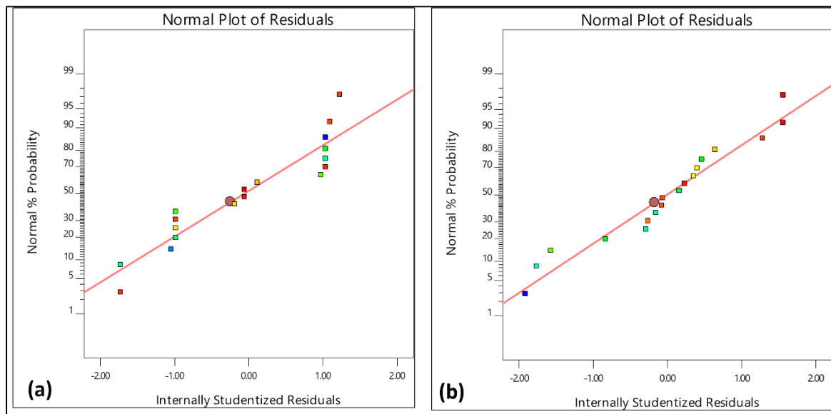
Figure 4.17: The normal plot of residual for second DoE (20% water, 80% methanol and 80% water, 20% methanol) (a) Tensile strength, (b) Young's modulus
