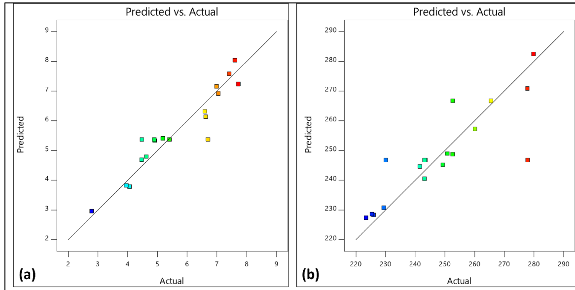
Figure 4.14: Prediction versus actual graph for first DoE (0% water, 100% methanol and 100% water, 0% methanol) (a) Tensile strength, (b) Young's modulus
