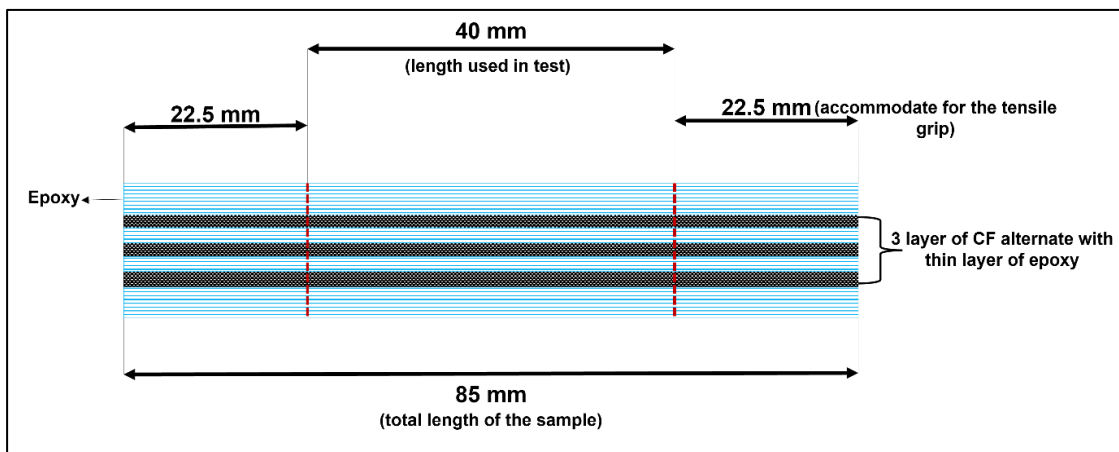
Figure 3.3: Schematic illustration of composites and their dimension
