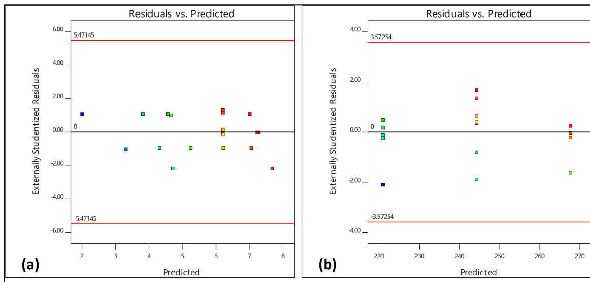
Figure 4.19: The residual versus predicted graph for second DoE (20% water, 80% methanol and 80% water, 20% methanol) (a) Tensile strength, (b) Young's modulus
