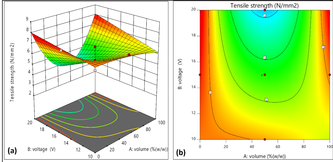
Figure 4.10: The response surface plot of tensile strength for first DoE (0% water, 100% methanol and 100% water, 0% methanol) (a) surface response (b) contour plot
