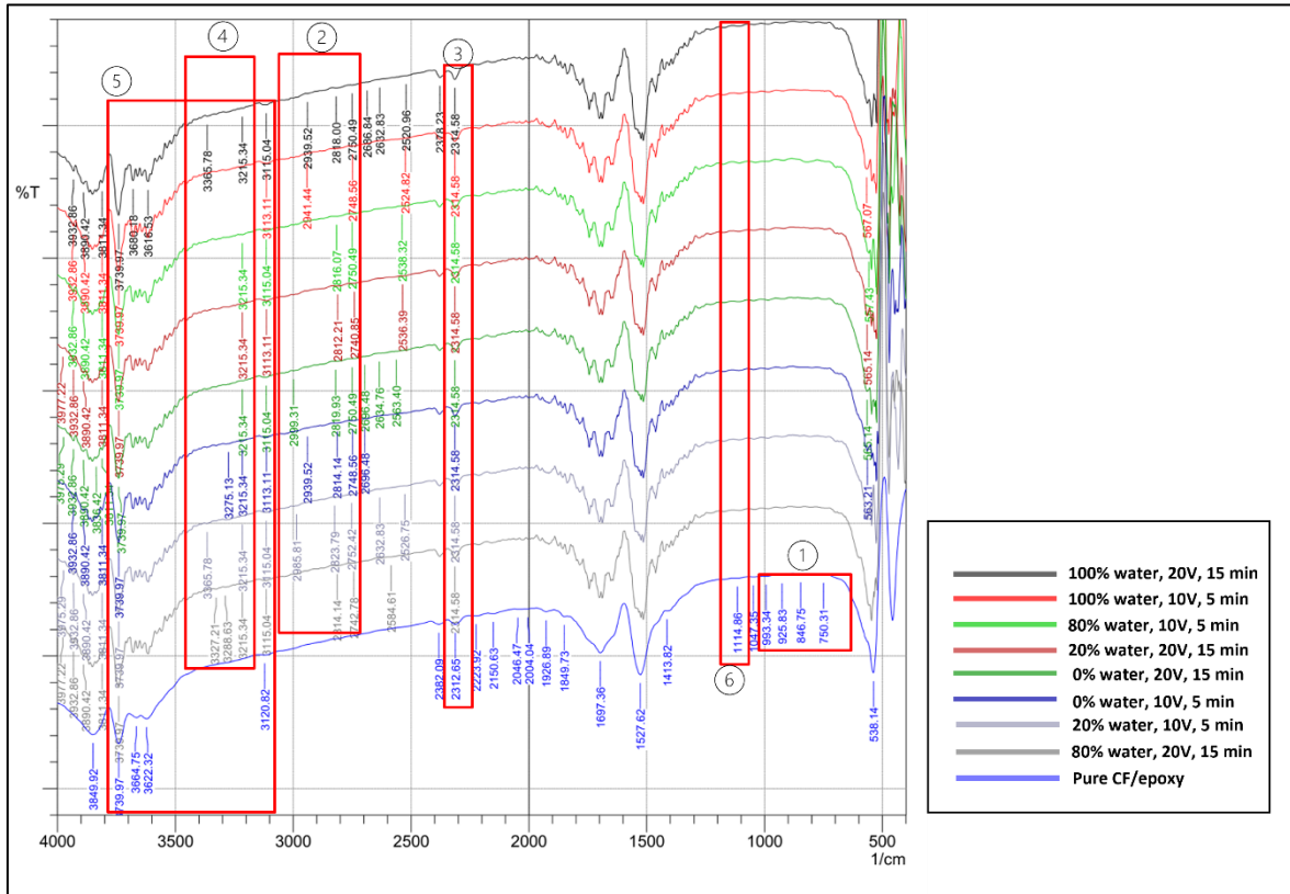
Figure 4.6: The FTIR analysis of composites
