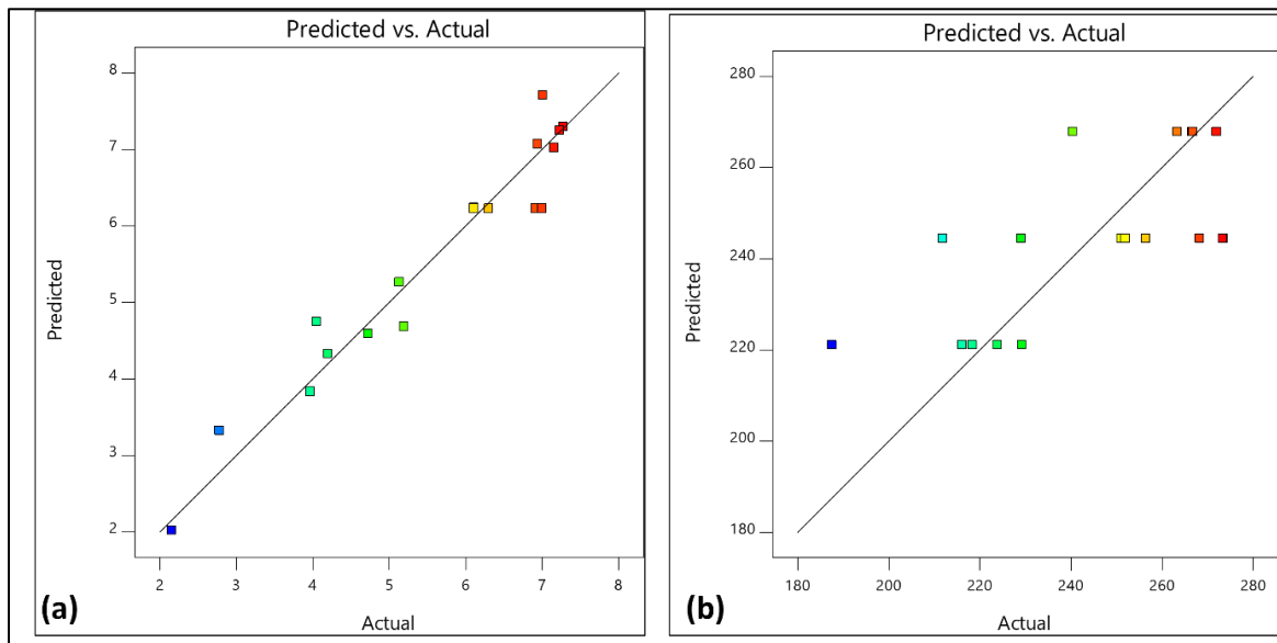
Figure 4.15: Prediction versus actual graph for second DoE (20% water, 80% methanol and 80% water, 20% methanol) (a) Tensile strength, (b) Young's modulus
