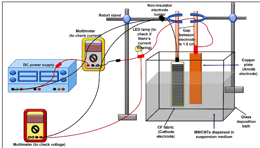
Figure 3.2: Schematic diagram of the EPD process for the fabrication of hybrid MWCNT-CF materials
