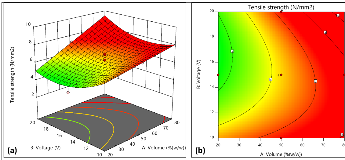
Figure 4.12: The response surface plot of tensile strength for second DoE (20% water, 80% methanol and 80% water, 20% methanol) (a) surface response (b) contour plot
