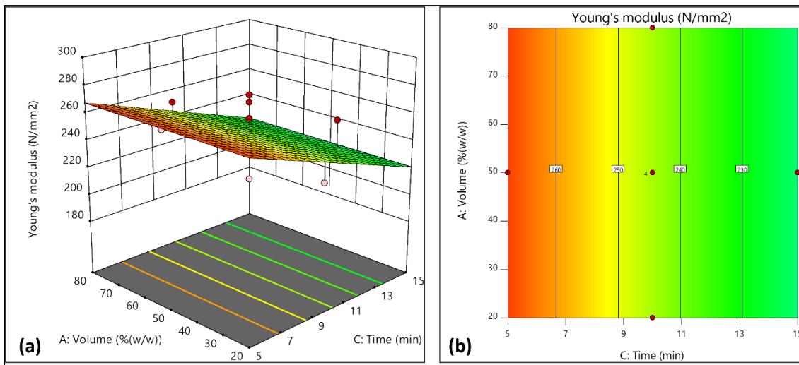
Figure 4.13: The response surface plot of Young's modulus for second DoE (20% water, 80% methanol and 80% water, 20% methanol) (a) surface response (b) contour plot
