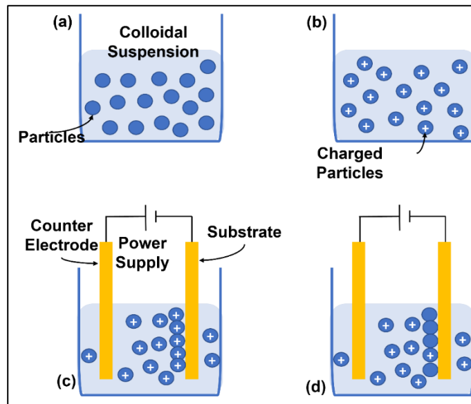
Figure 2.2: The four steps in EPD process (a) dispersion, (b) electrochemical charging, (c) electrophoresis, and (d) deposition (Amrollahi et al., 2016)
