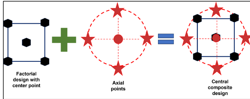
Figure 2.12: CCD schematic illustration (Veza et al., 2023)
