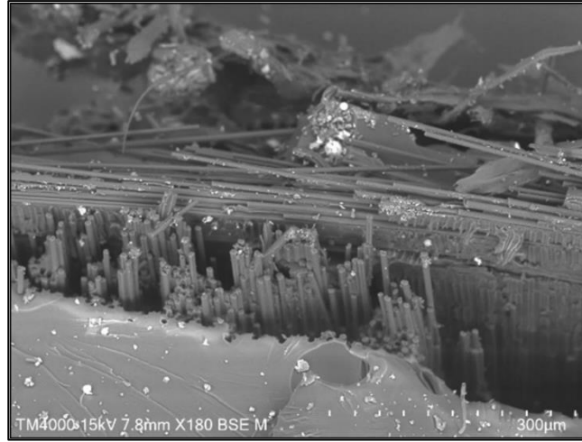
Figure 4.7: Surface morphology of pure CF/ epoxy composite
