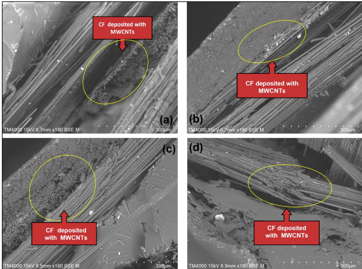
Figure 4.8: SEM images of CNT-CF/epoxy composites when deposition voltage: 20V, deposition time: 15 minutes: (a) 0% water, (b) 20% water, (c) 80% water, (d) 100% water
