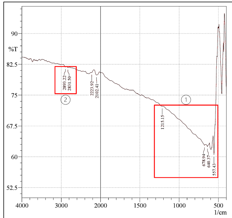
Figure 4.3: The FTIR analysis of pristine CF fabric
