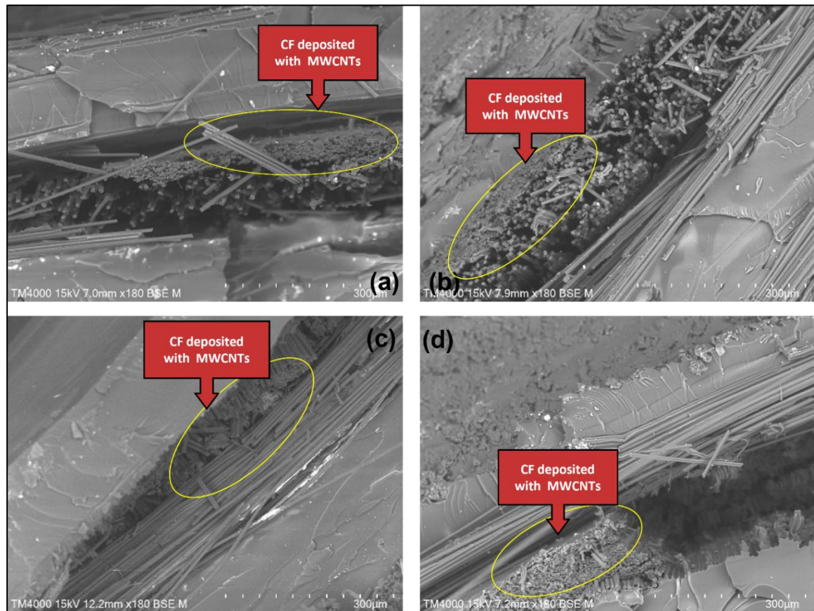
Figure 4.9: SEM images of CNT-CF/epoxy composites when deposition voltage: 10V, deposition time: 5 minutes: (a) 0% water, (b) 20% water, (c) 80% water, (d) 100% water
