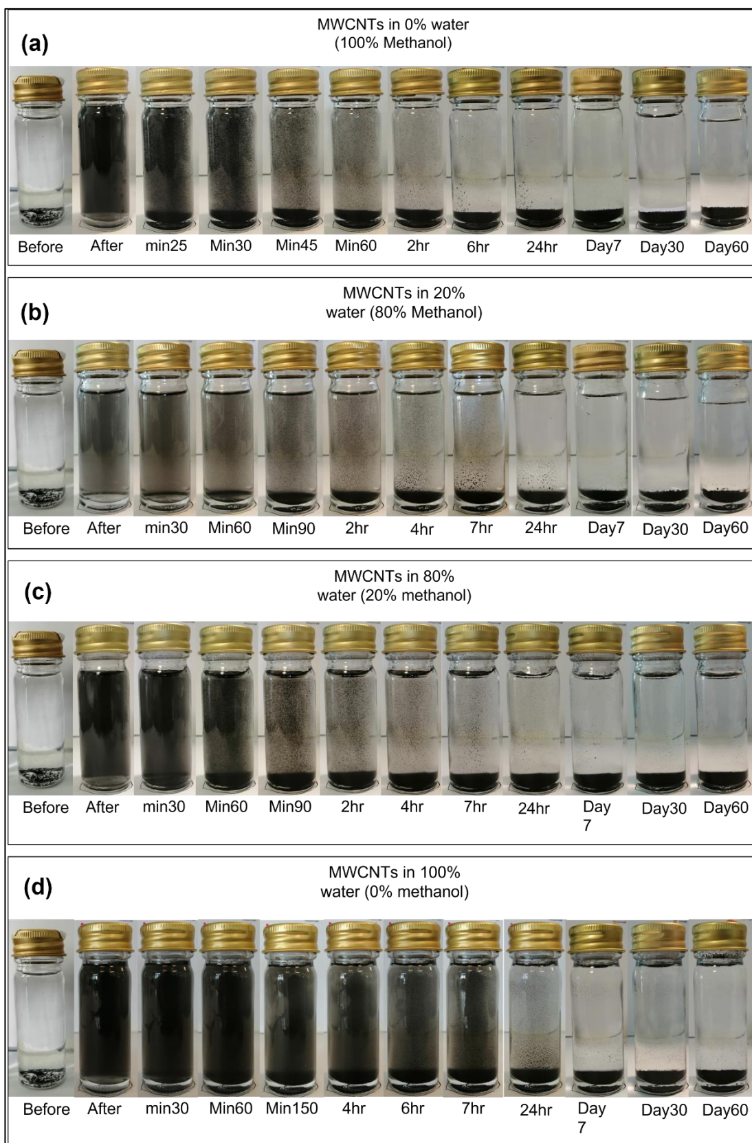
Figure 4.5: Optical observations of MWCNTs dispersed in suspension medium with different ratios of water-methanol
