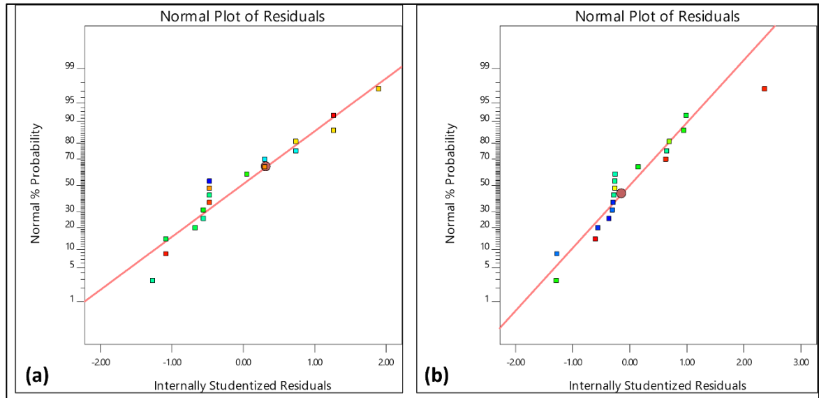
Figure 4.16: The normal plot of residual for first DoE (0% water, 100% methanol and 100% water, 0% methanol) (a) Tensile strength, (b) Young's modulus
