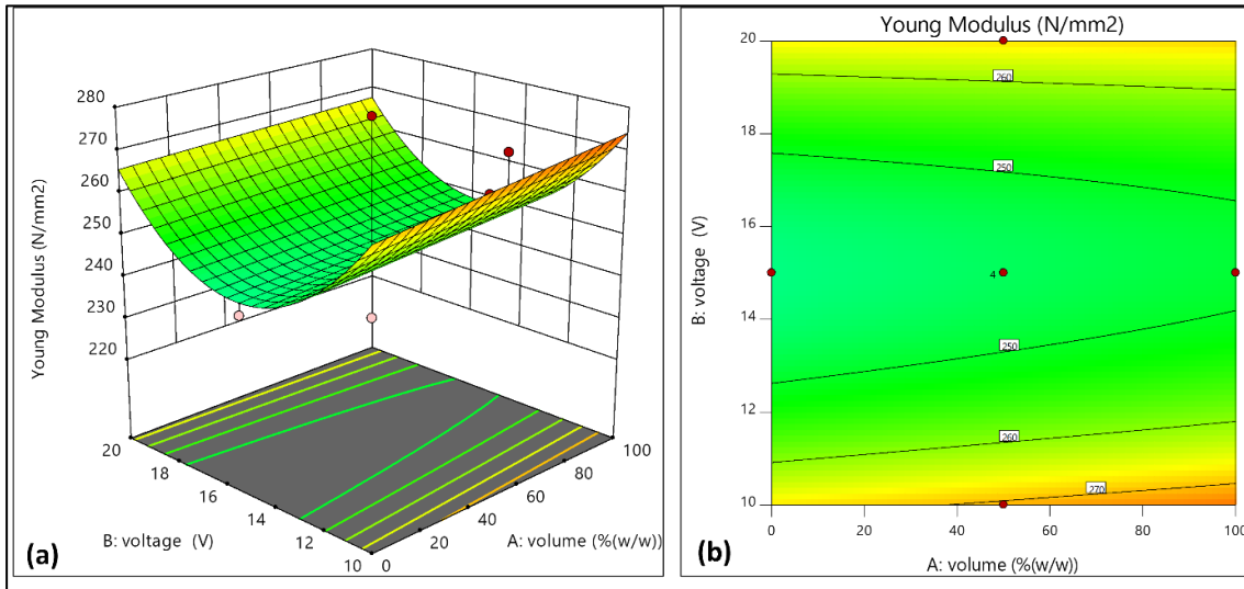
Figure 4.11: The response surface plot of Young's modulus for first DoE (0% water, 100% methanol and 100% water, 0% methanol) (a) surface response (b) contour plot
