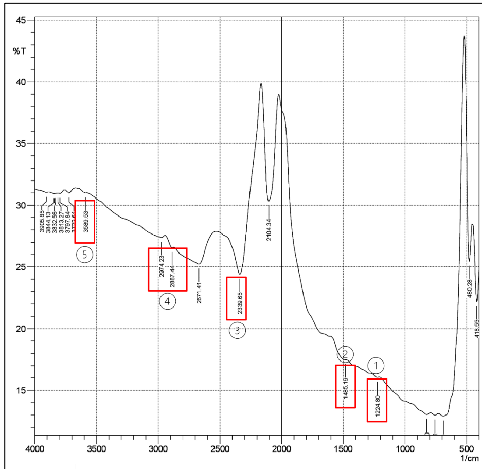
Figure 4.1: The FTIR analysis of pristine MWCNTs powder
