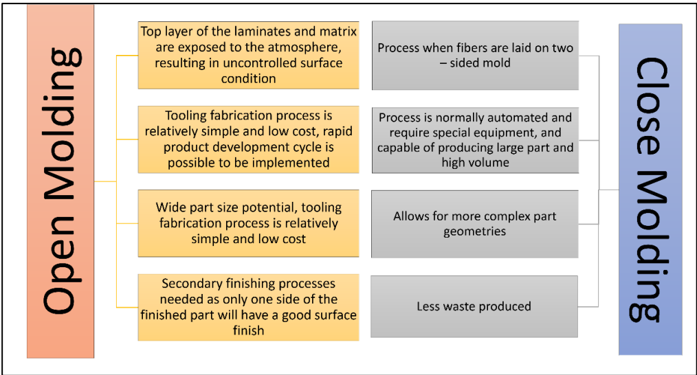
Figure 2.9: Comparison between open and closed molding processes (Lee et al., 2021)
