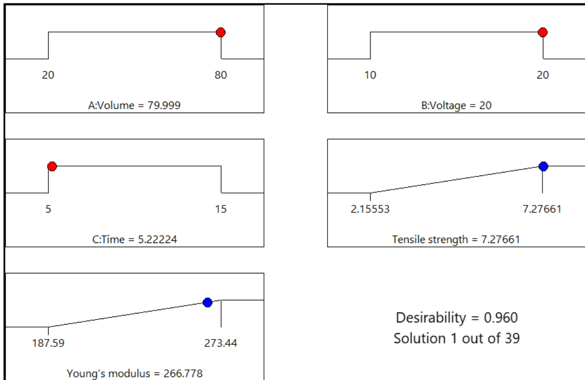
Figure 4.21: Numerical ramp graph for statistically optimized factors and response for second experimental design (20% water, 80% methanol and 80% water,20% methanol)
