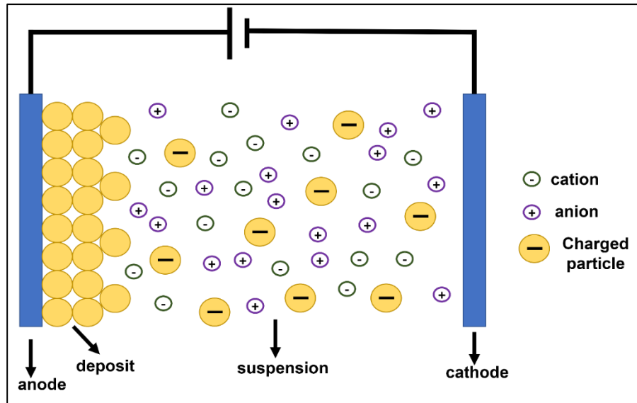
Figure 2.1: Simple schematic diagram of the EPD process (Hu et al., 2020)
