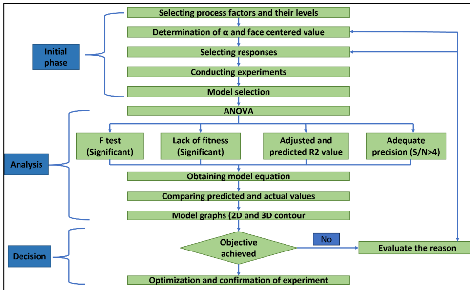
Figure 2.11: CCD flow diagram (Bhattacharya, 2021)
