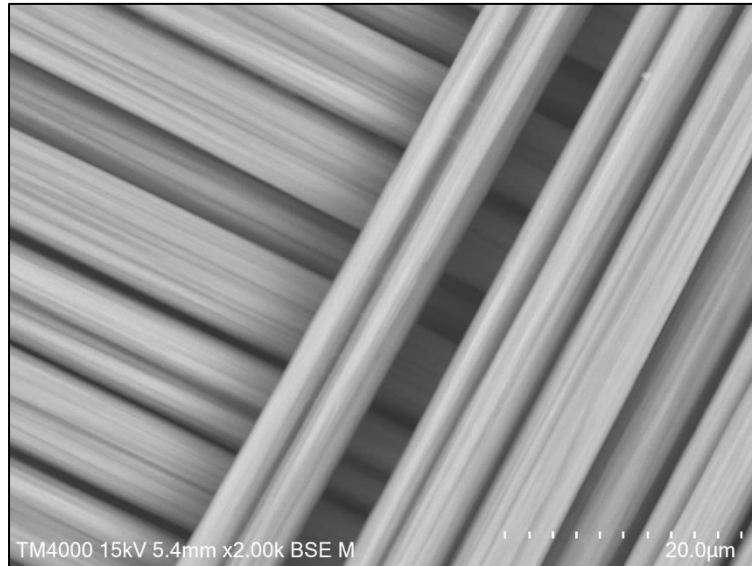
Figure 4.4: SEM of pristine CF fabric at a magnification of x2000
