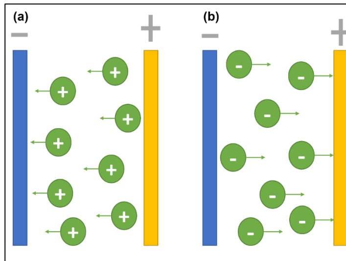
Figure 2.3: Schematic illustration of two types of EPD (a) cathodic and (b) anodic EPD (Ranjbar & Bakhtiary-Noodeh, 2020)
