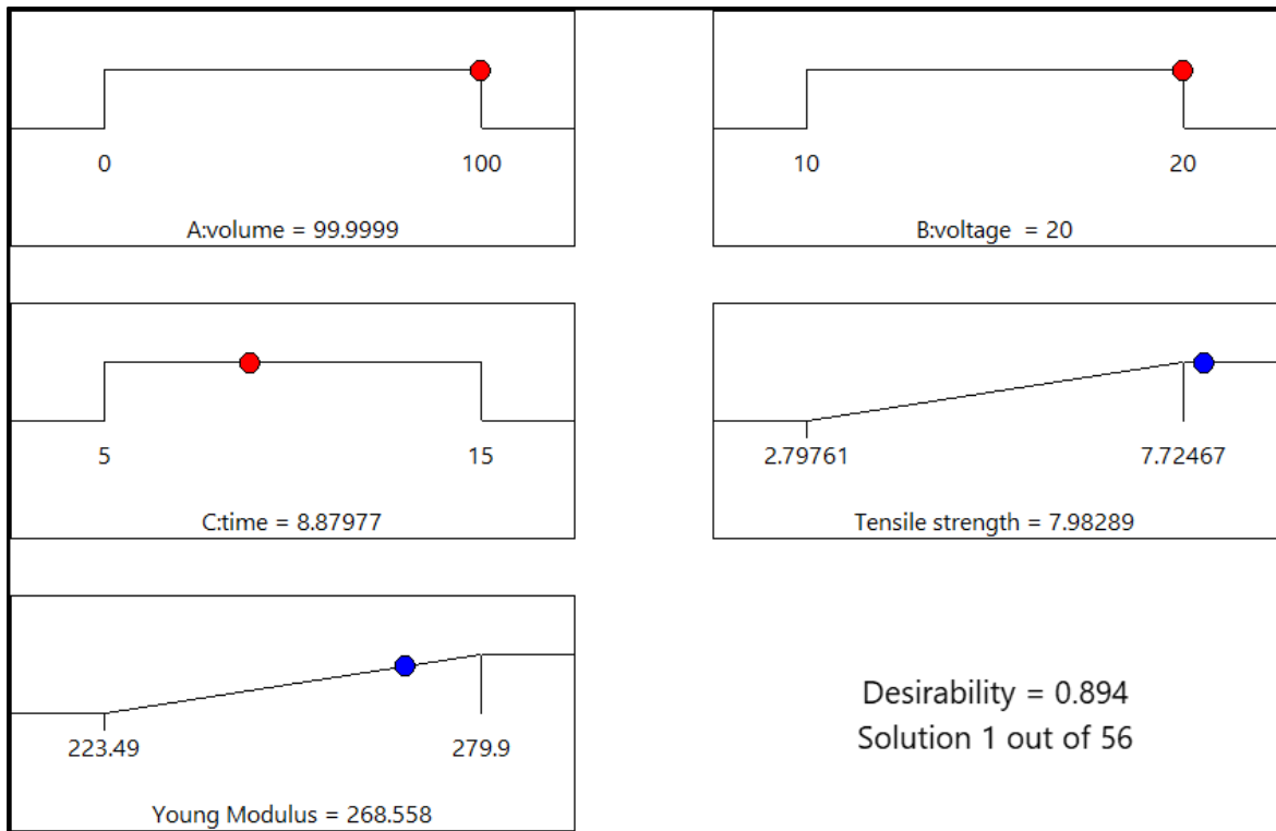
Figure 4.20: Numerical ramp graph for statistically optimized factors and response for first experimental design (0% water, 100% methanol and 100% water,0% methanol)
