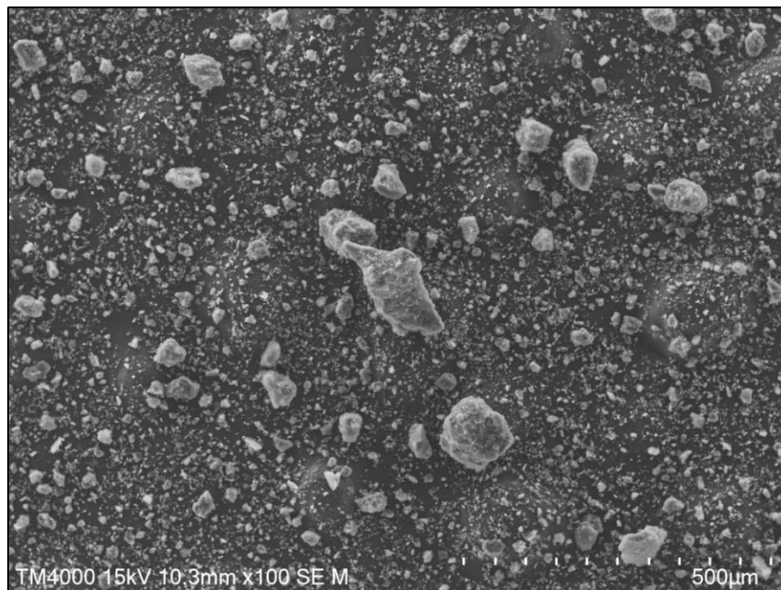
Figure 4.2: SEM of pristine MWCNTs powder at a magnification of x100
