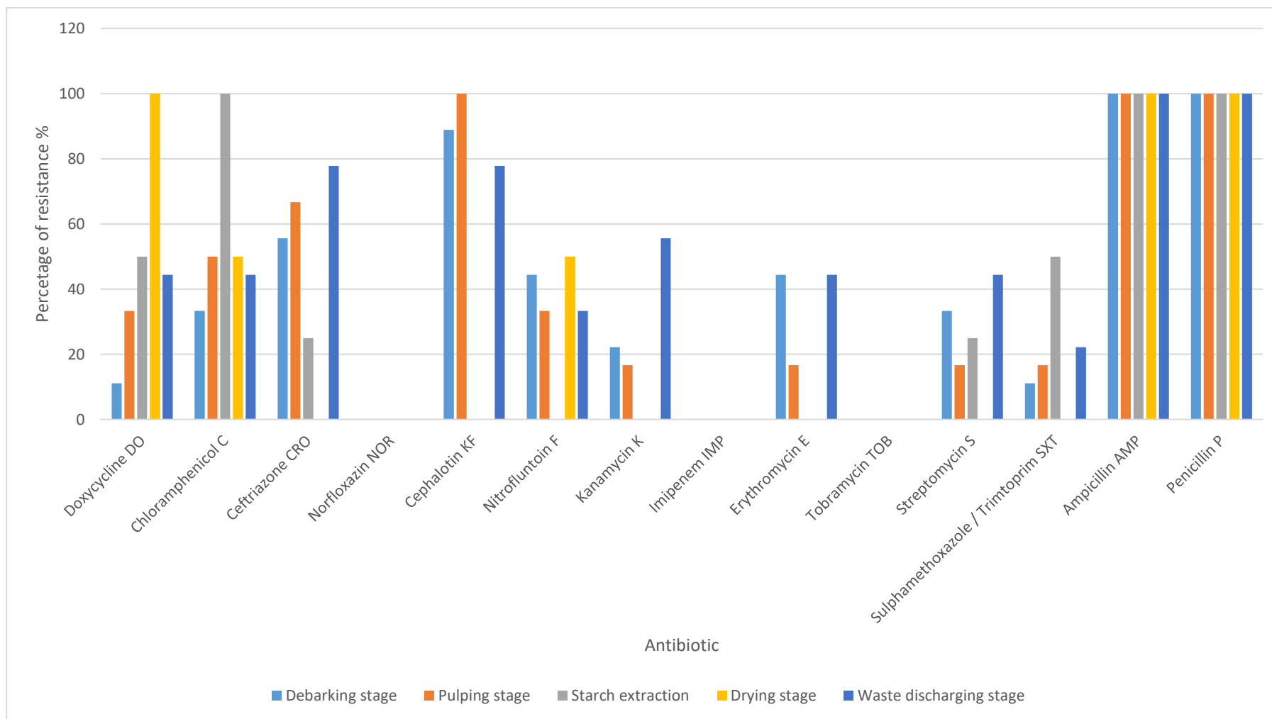
Figure 3.4: The percentage of antibiotic resistance of B. cereus in every stage of processing in sago processing mill B
