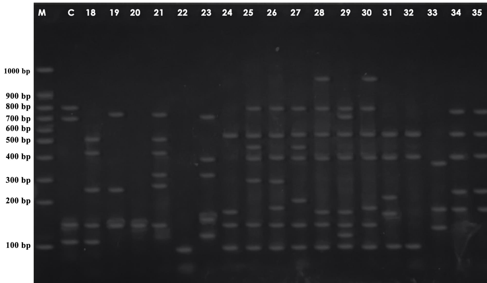
Figure 3.7: Banding profiles of ERIC PCR for sago processing mill B. Lane M: 100 bp ladder (Vivantis, USA), C: Positive control, 18: SPB 16, 19: SPB 17, 20: SPB 18, 21: SPB 19, 22: SPB 21, 23: SPB 22, 24: SPB 24, 25: SPB 27, 26: SPB 28, 27: SPB 29, 28: SPB 31, 29: SPB 35, 30: SPB 37, 31: SPB 39, 32: SPB 47, 33: SPB 48, 34: SPB 61, 35: SPB 62
