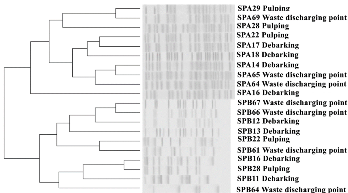
Figure 3.13: Dendrogram of PFGE profiles for sago processing mill
