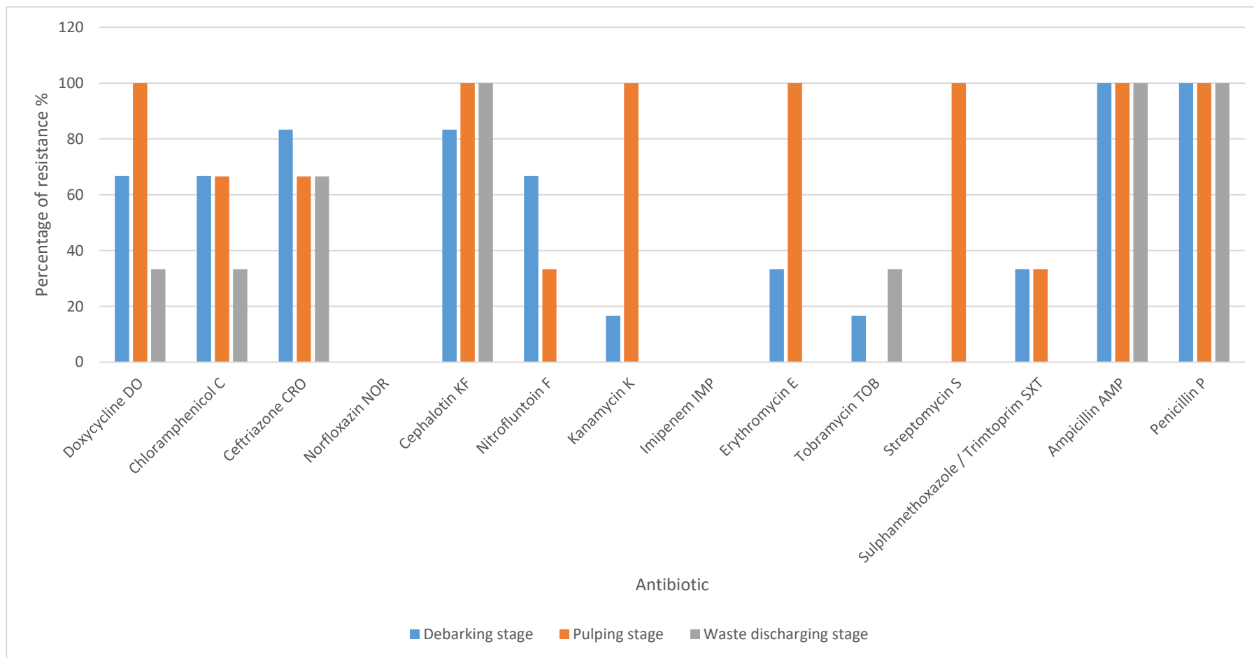
Figure 3.3: The percentage of antibiotic resistance of B. cereus in every stage of processing in sago processing mill A.
