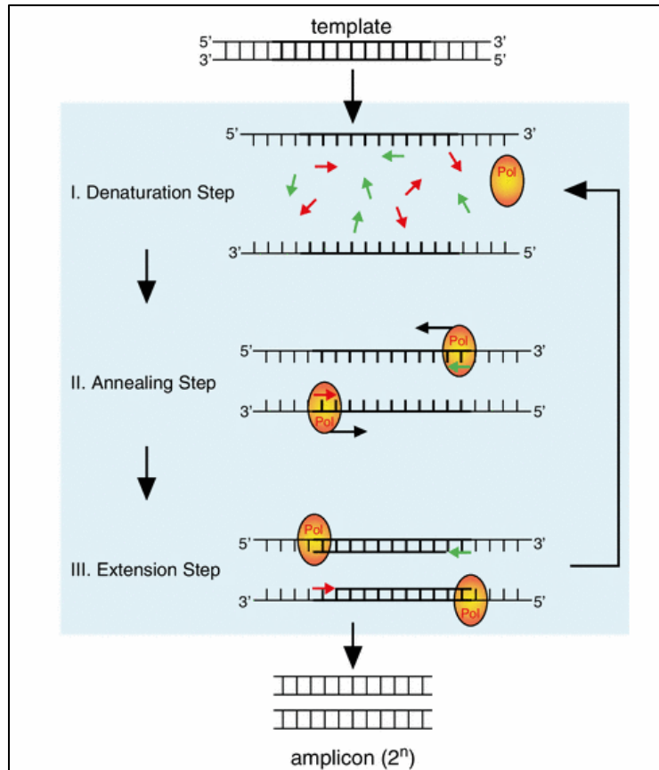
Figure 1.8: Overview of PCR amplification process (Pasic et al. , 2014).
