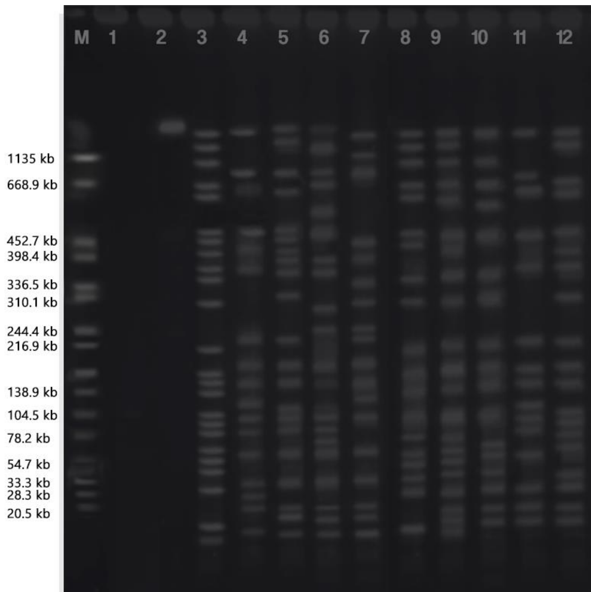
Figure 3.11: Banding profiles of PFGE for sago processing mill A. Lane M: DNA size marker, Salmonella enterica serotype Braenderup H9812. 3: SPA 14, 4: SPA 16, 5: SPA 17, 6: SPA 18, 7: SPA 22, 8: SPA 28, 9: SPA 29, 10: SPA 64, 11: SPA 65, 12: SPA 69
