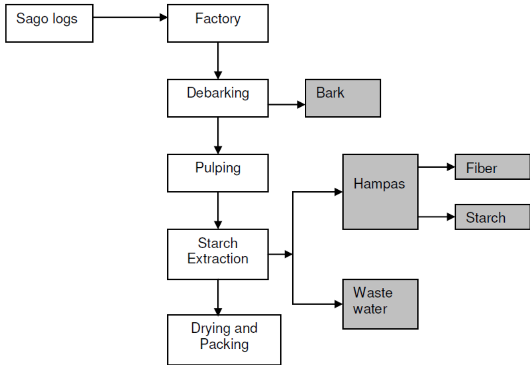
Figure 1.7: Schematic flow diagram of the sago processing (Bujang, 2008).
