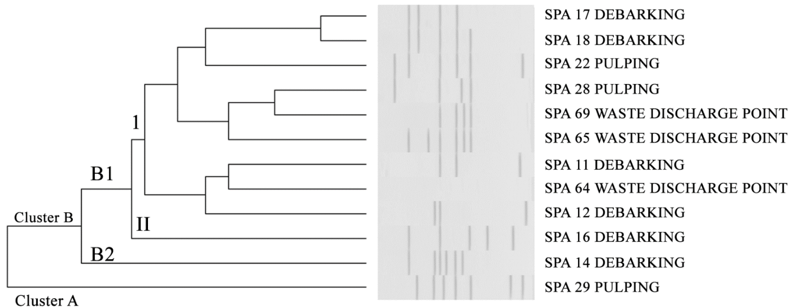
Figure 3.9: Dendrogram of ERIC-PCR profiles for sago processing mill A
