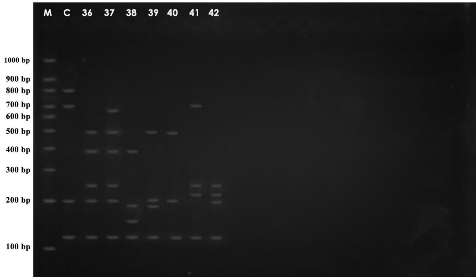
Figure 3.8: Banding profiles of ERIC PCR for sago processing mill B. Lane M: 100 bp ladder (Vivantis, USA), C: Positive control, 36: SPB 63, 37: SPB 64 38: SPB 65, 39: SPB 66, 40: SPB 67, 41: SPB 68, 42: SPB 6
