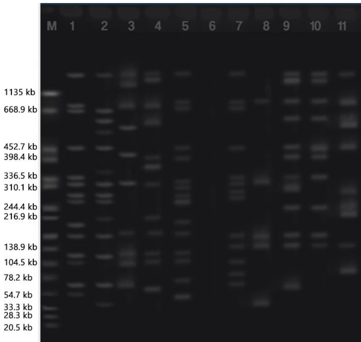
Figure 3.12 Banding profiles of PFGE for sago processing mill B. Lane M: DNA size marker, Salmonella enterica serotype Braenderup H9812. 1: SPB 11, 2: SPB 12, 3: SPB 13, 4: SPB 14, 5: SPB 22, 7: SPB 28, 8: SPB 61, 9: SPB 66, 10: SPB 67
