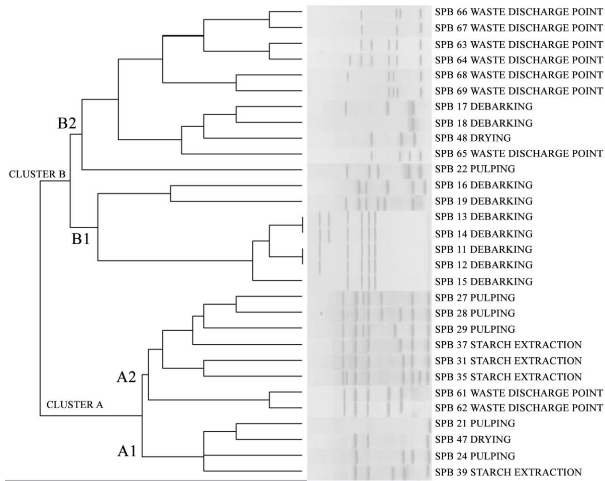
Figure 3.10: Dendrogram of ERIC-PCR profiles for sago processing mill B
