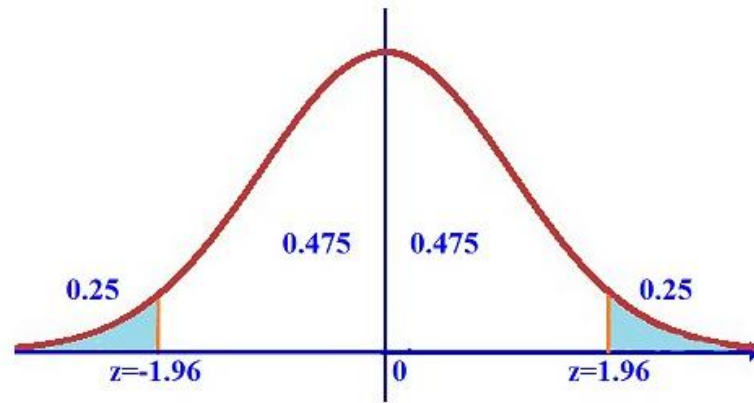
Figure 3.2: Standard Normal Curve (Math Captain, 2015)
