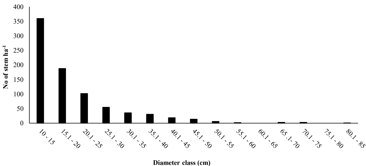
Fig. 3. Tree distribution by diameter classes in Division 5.
