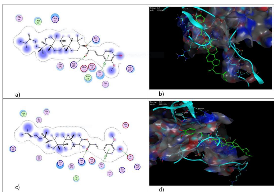
Fig. 5: 2D and 3D representation of binding interactions of 24-methylenecycloartenyl ferulate (a and b) and cycloartenyl ferulate (c and d) with the active site of NF- \kappa B (1IKN)
