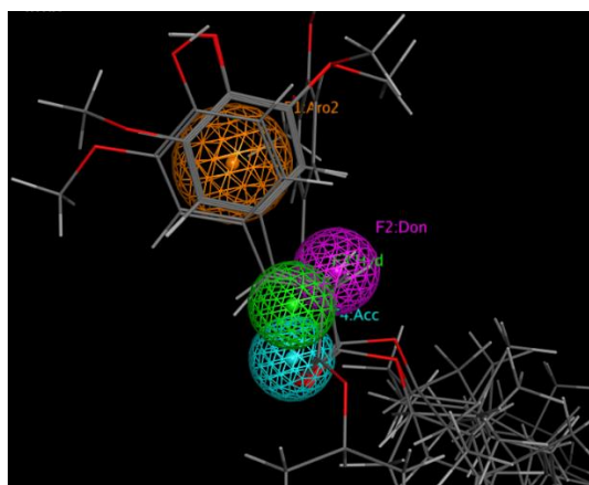
Fig. 3: The pharmacophore mapping of all four compounds on the model, \gamma -oryzanol compounds i. e. 24-methylenecycloartenyl ferulate, cycloartenyl ferulate, campesteryl ferulate, and \beta -sitosterol ferulate exhibited fit score >2 and RMSD <1 as given in table 2
