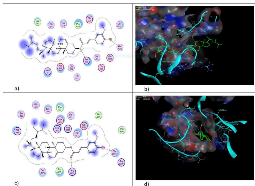
Fig. 6: 2D and 3D representation of binding interactions of campesteryl ferulate (a and b) and \beta -sitosteryl ferulate (c and d) with the active site of NF- \kappa B (11KN)
