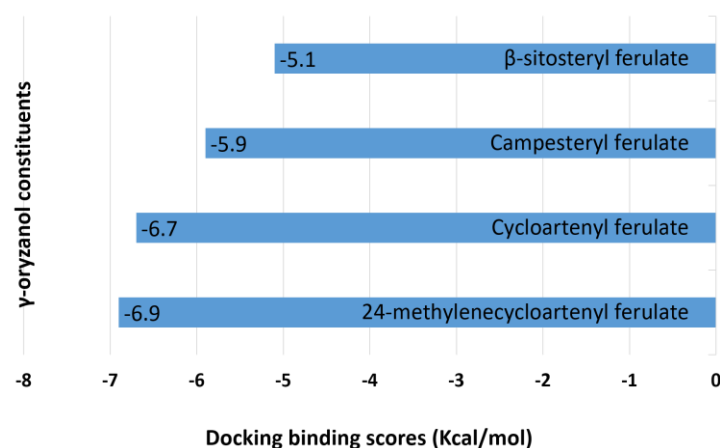
Fig. 4: Molecular docking binding scores (kilocalorie per mole) of gamma oryzanol constituents with NF- \kappa B
