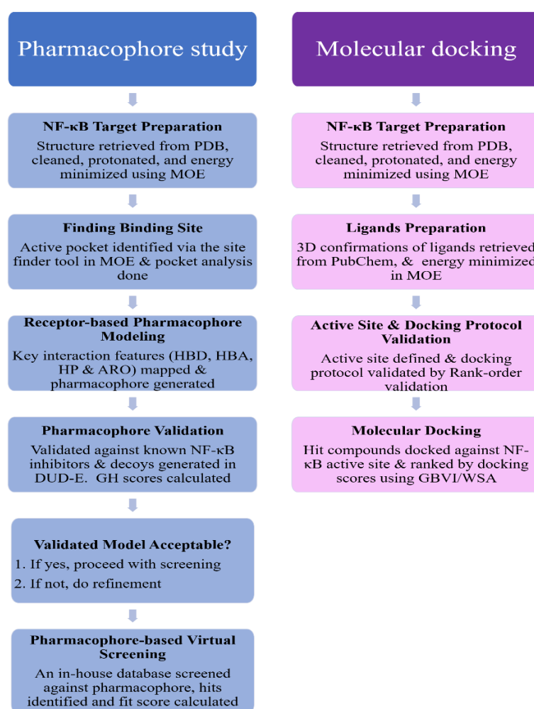
Fig. 1: Workflow of receptor structure preparation, pharmacophore generation, and molecular docking
