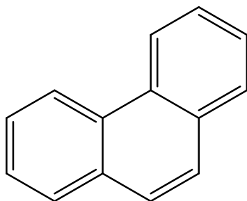
Phenanthrene
