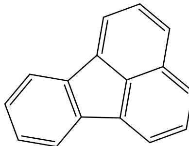
Fluoranthene
