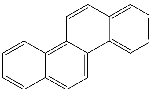
Chrysene
