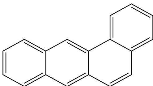
Benzo[a]anthracene
