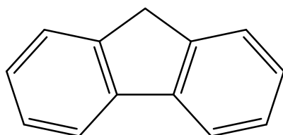
Fluorene
