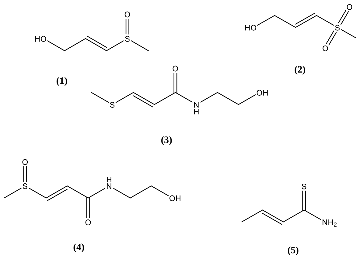
Figure 2.3: Chemical structure of trans -3-methylsulfinyl-2-propenol (1), trans -3-methylsulfonyl-2-propenol (2), entadamide A (3), entadamide C (4), and trans -3-methylthioacrylamide (5).
