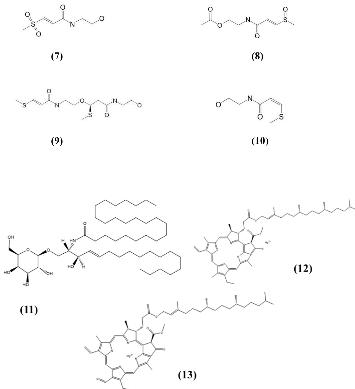
Figure 2.4: Chemical structure of bioactive compounds isolated from C. nutans . Vitexin (1), orientin (2), isovitexin (3), shaftoside (4), isoorientin (5), and apigenin 6,8-C- \alpha -L-pyranarabinoside (6), clinamides A (7), B (8), and C (9), 2-cis-entadamide A (10), cerebrosides (11), chlorophyll A (12), and chlorophyll B (13).
