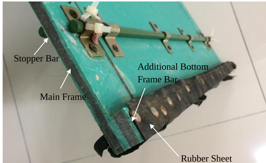
Figure 2.8: Components of gate frame subsystem
