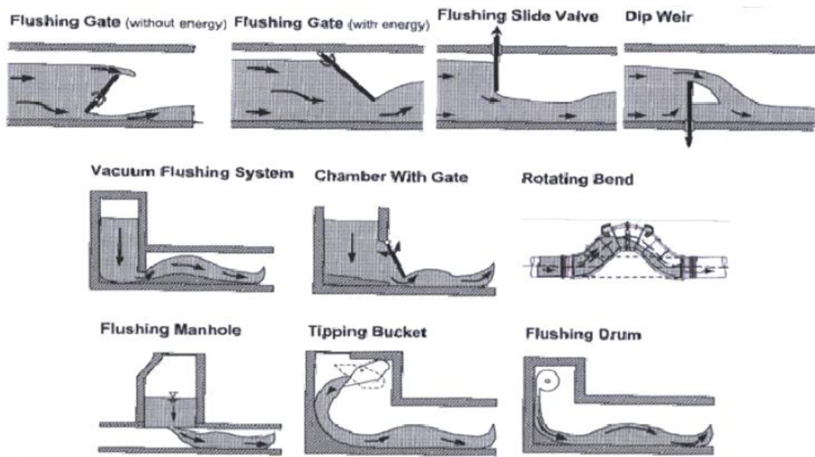
Figure 2.1: Flushing devices implemented for sewer and basin cleaning (Dettmar et al., 2002)
