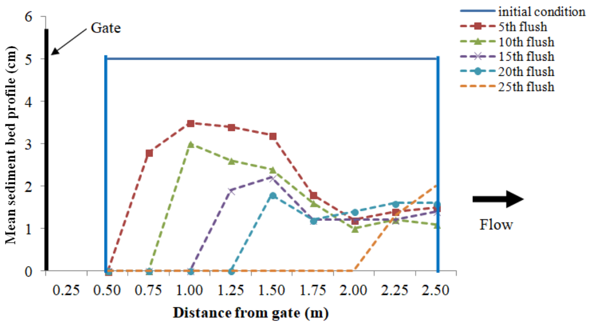
Figure 4.4: Sediment profiles for sediment d_{50} of 0.71 mm laid starting from 0.5 m from the gate with \theta = 75^\circ after flushes for 5 cm initial sediment deposition thickness
