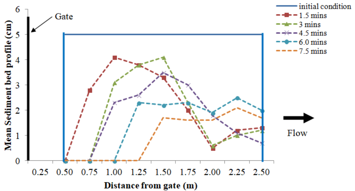
Figure 4.10: Sediment profiles for sediment d_{50} of 2 mm laid starting from 0.5 m from the gate with \theta = 60^\circ after flushes for 5 cm initial sediment deposition thickness for long flush operation
