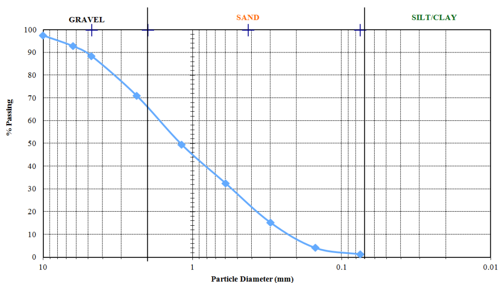
Figure 4.12: Sediment size distributions for the selected open storm sewer
