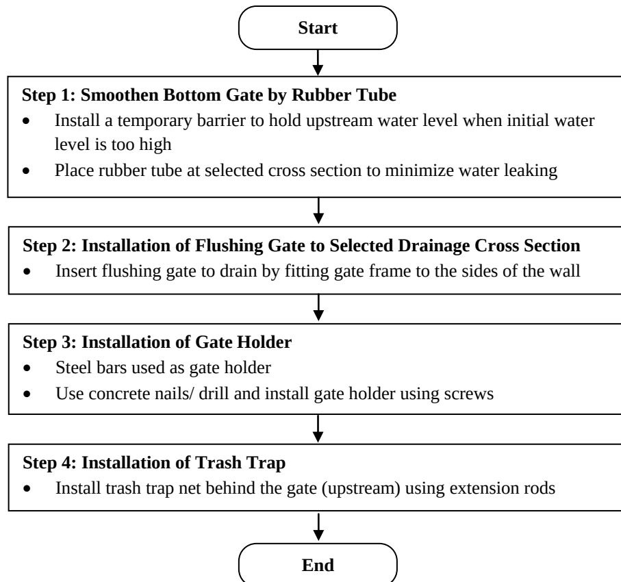
Figure 5.7: Flushing gate installation process
