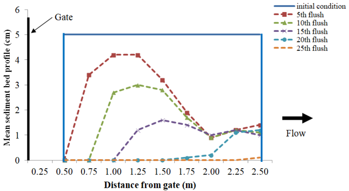
Figure 4.3: Sediment profiles for sediment d_{50} of 0.71 mm laid starting from 0.5 m from the gate with \theta = 90^\circ after flushes for 5 cm initial sediment deposition thickness
