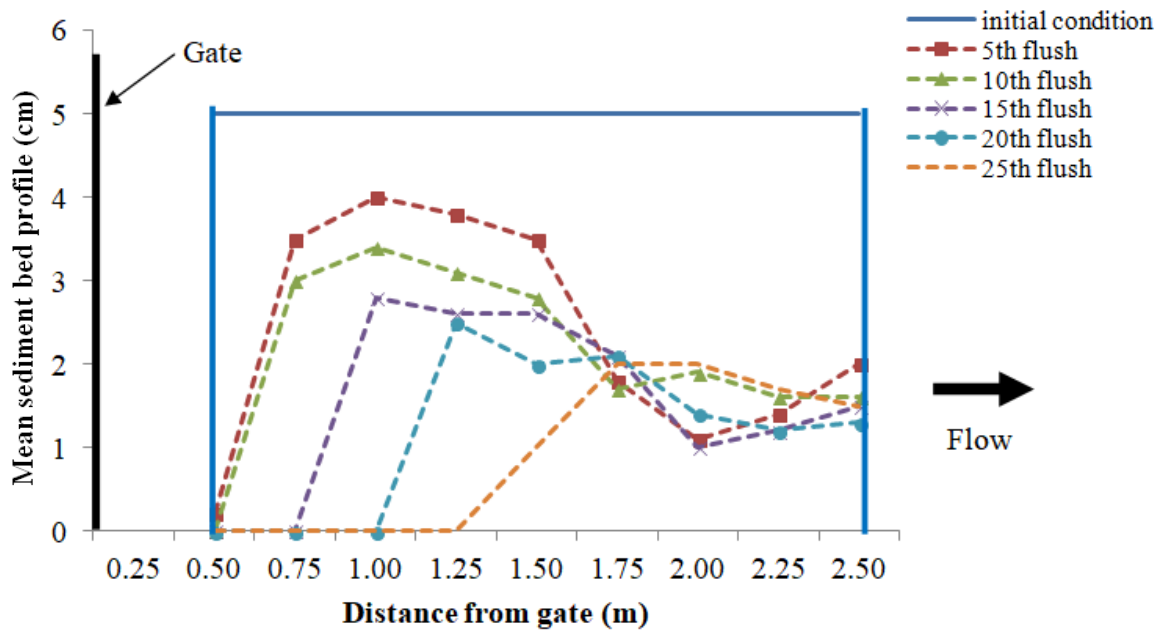
Figure B.2: Sediment profiles for sediment d_{50} of 1.18 mm laid starting from 0.5 m from the gate with \theta = 75^\circ after flushes for 5 cm initial sediment deposition thickness
