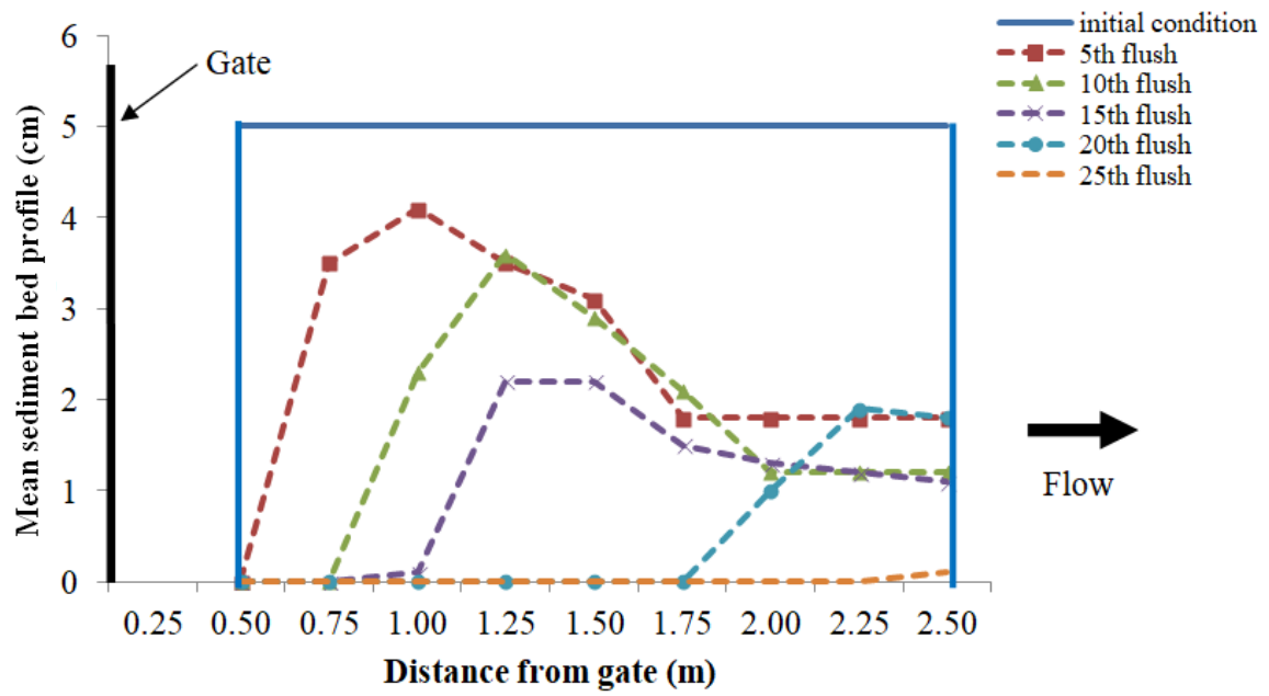
Figure B.1: Sediment profiles for sediment d_{50} of 1.18 mm laid starting from 0.5 m from the gate with \theta = 90^\circ after flushes for 5 cm initial sediment deposition thickness
