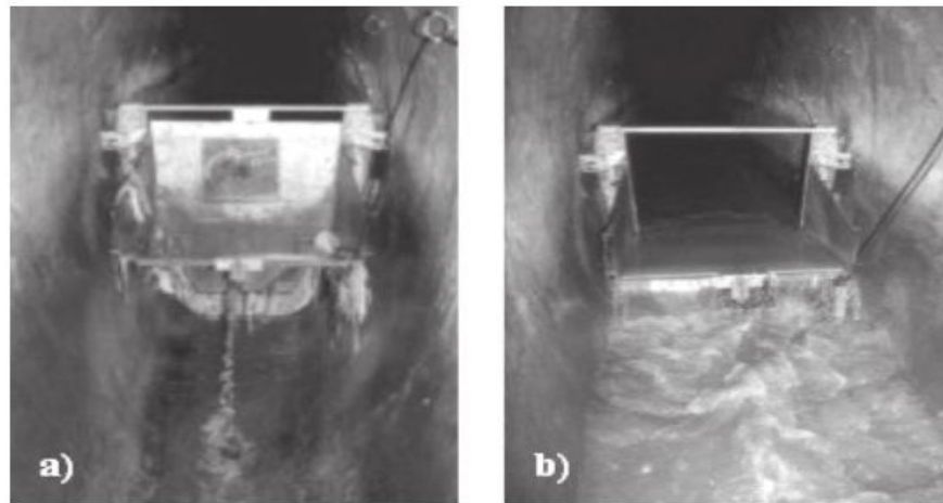
Figure 2.2: Hydrass gate (a) storage phase (b) flushing phase (Bertrand-Krajewski et al., 2005)
