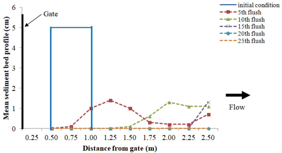
Figure B.7: Sediment profiles for sediment d_{50} of 1.18 mm laid starting from 0.5 m to 1.0 m from the gate with \theta = 60^\circ after flushes for 5 cm initial sediment deposition thickness
