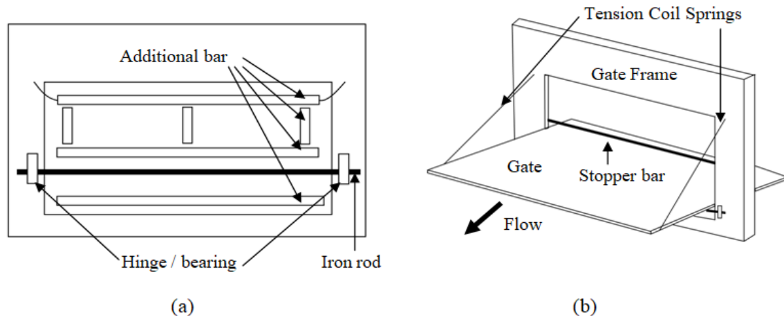
Figure 5.2: Typical tipping flush gate structure (a) front view (b) isometric view
