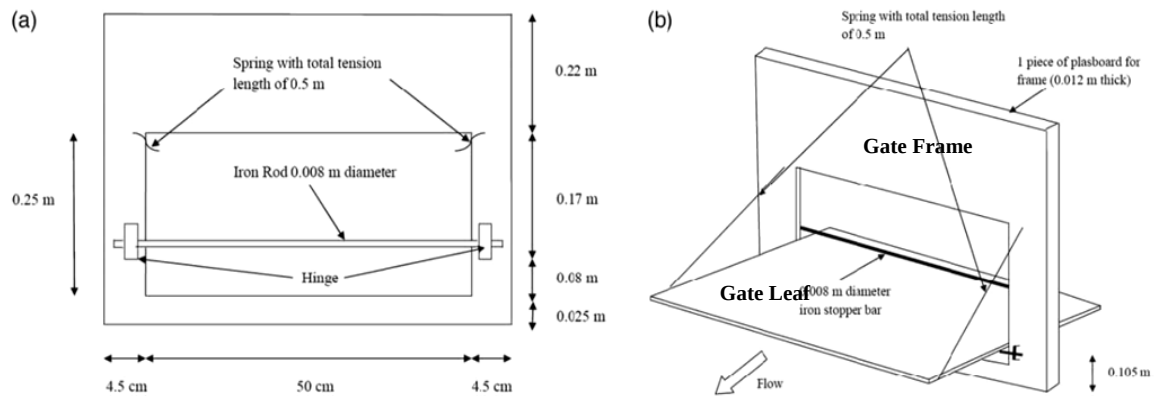
Figure 2.4: Views of the tipping flush gate model (a) front view; and (b) isometric view (not to scale) (Bong, Lau, & Ab. Ghani, 2013)
