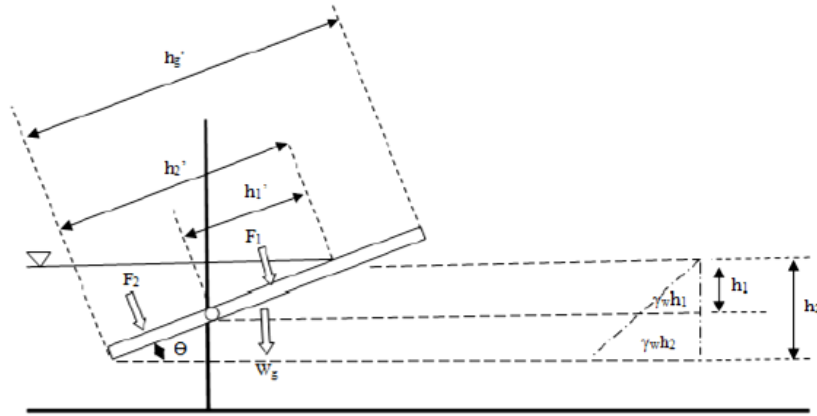
Figure 5.5: Forces acting on tipping flushing gate when open (Bong et al., 2016).
