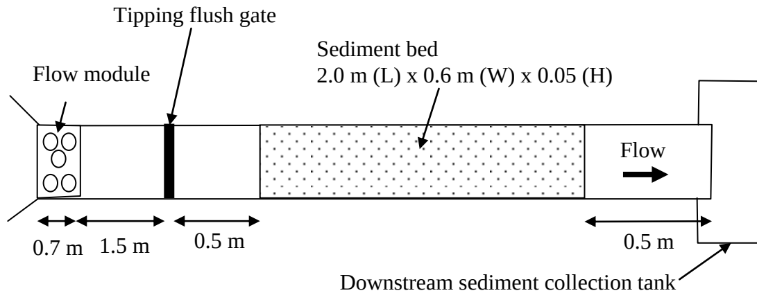
Figure 3.5: Plan view schematic of flushing experiment in flume (not to scale)
