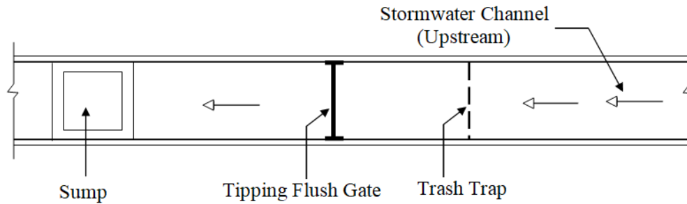
Figure 5.1: Typical layout and system components of tipping flush gate system
