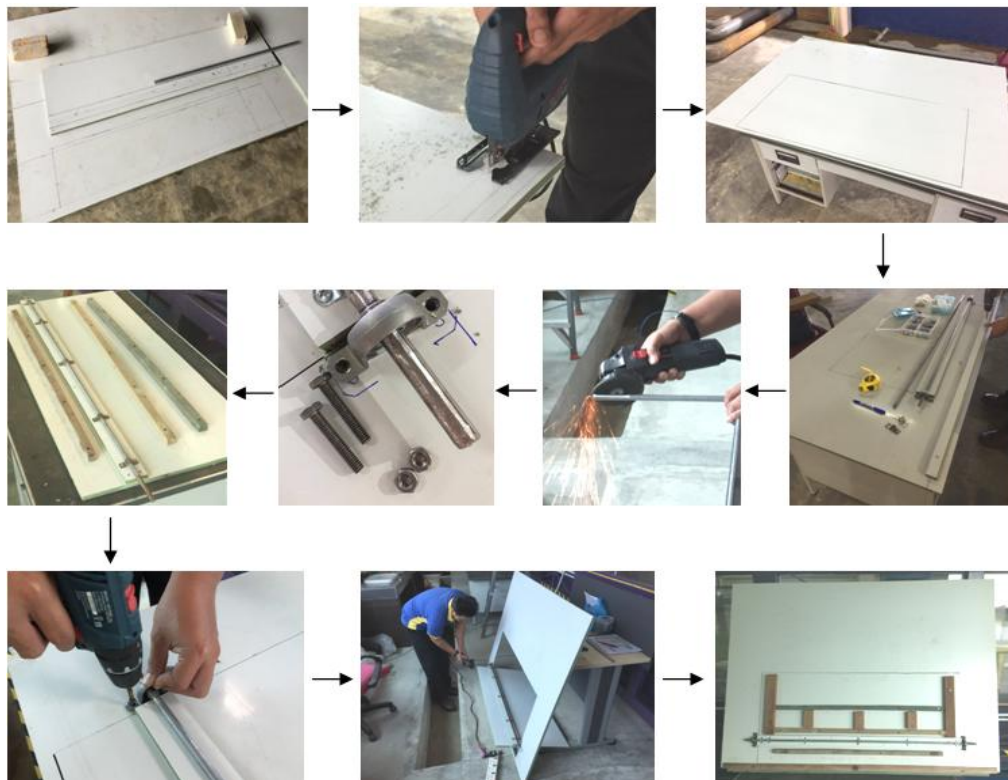
Figure 3.3: Tipping flush gate construction and assembly process
