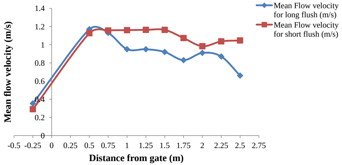
Figure 4.9: Mean flow velocity for long flush and short at \theta = 60^\circ
