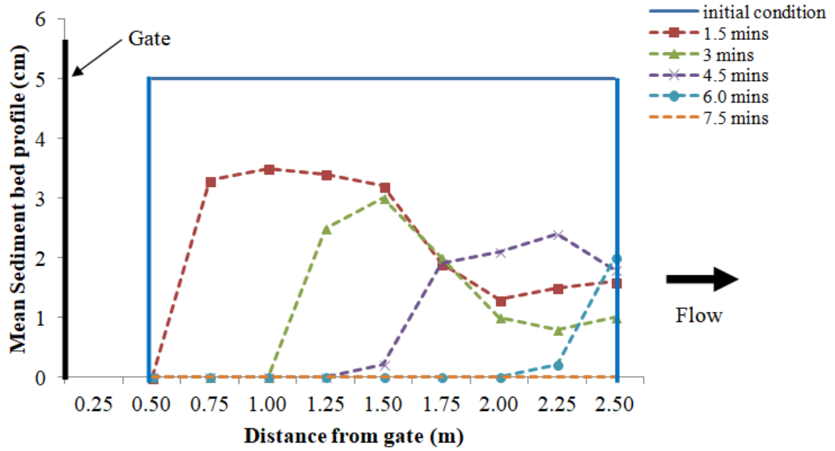
Figure 4.11: Sediment profiles for sediment d_{50} of 2 mm laid starting from 0.5 m from the gate with \theta = 60^\circ after flushes for 5 cm initial sediment deposition thickness for short flush operation (more frequent flush)
