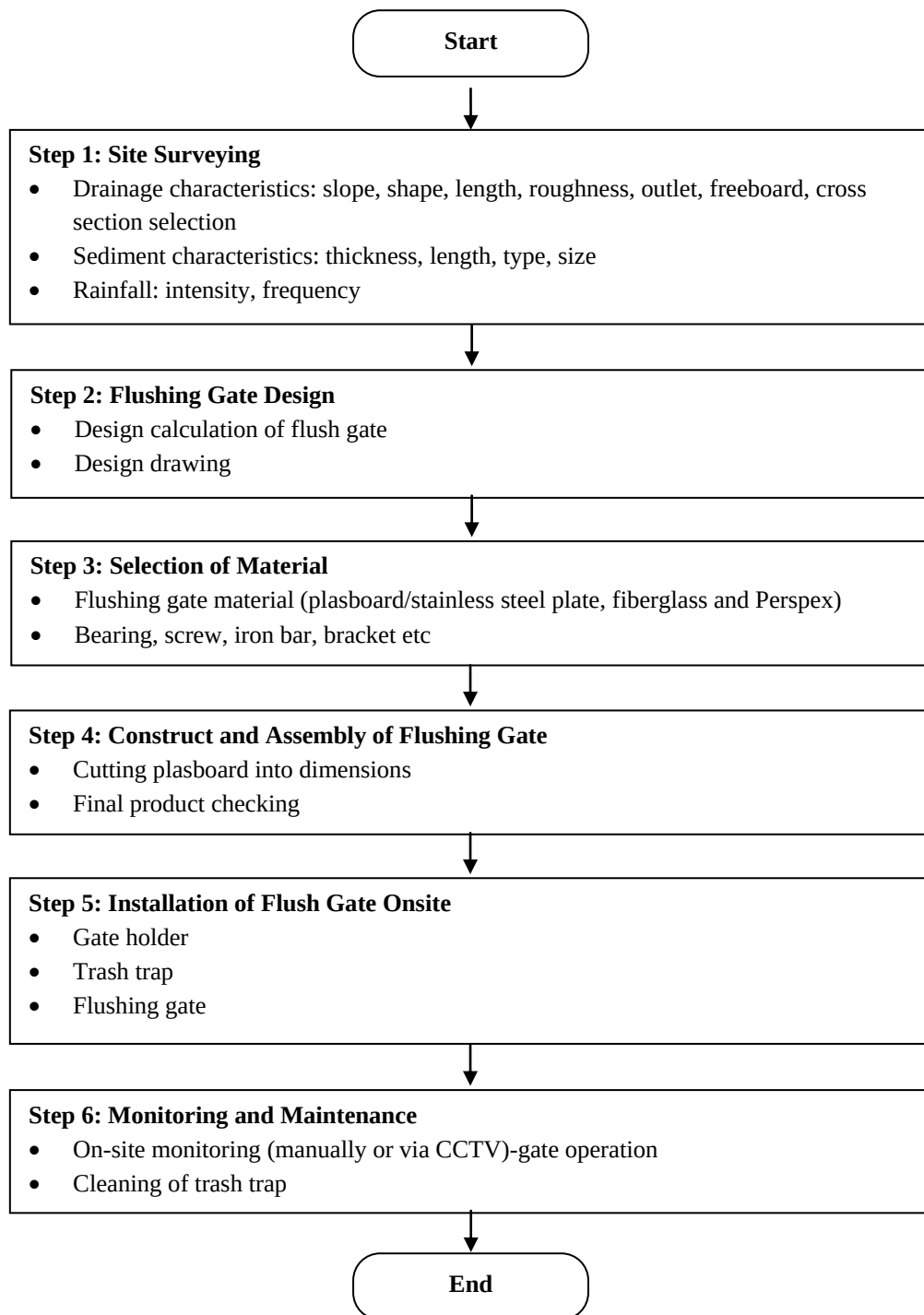
Figure 5.3: Workflow for flushing gate in open stormwater system
