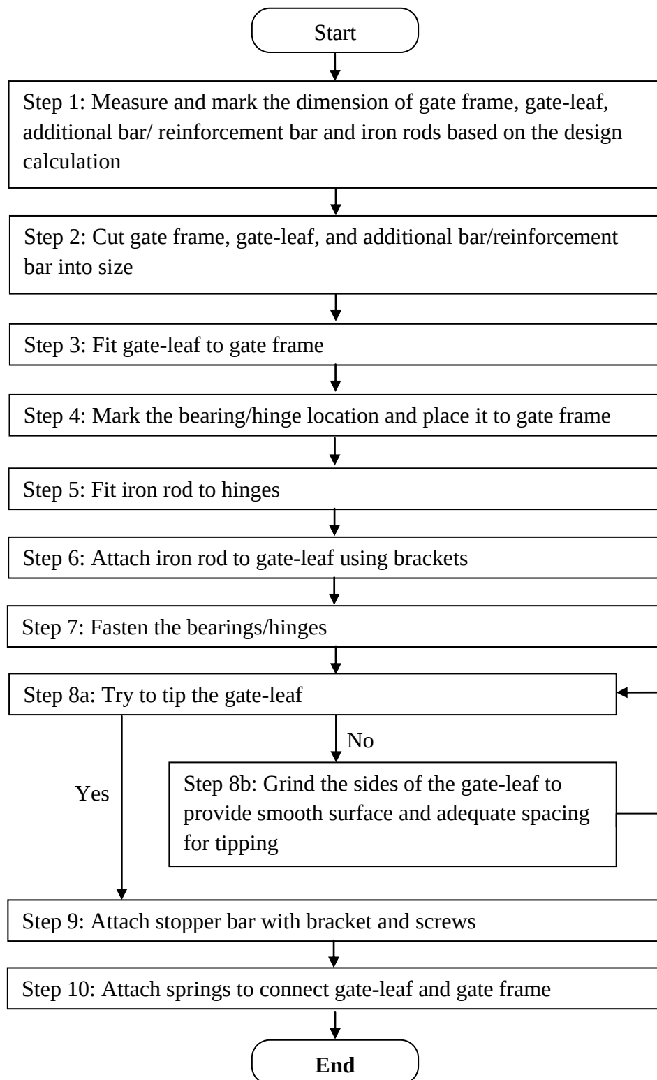
Figure 3.4: Tipping flush gate construction and assembly process chart
