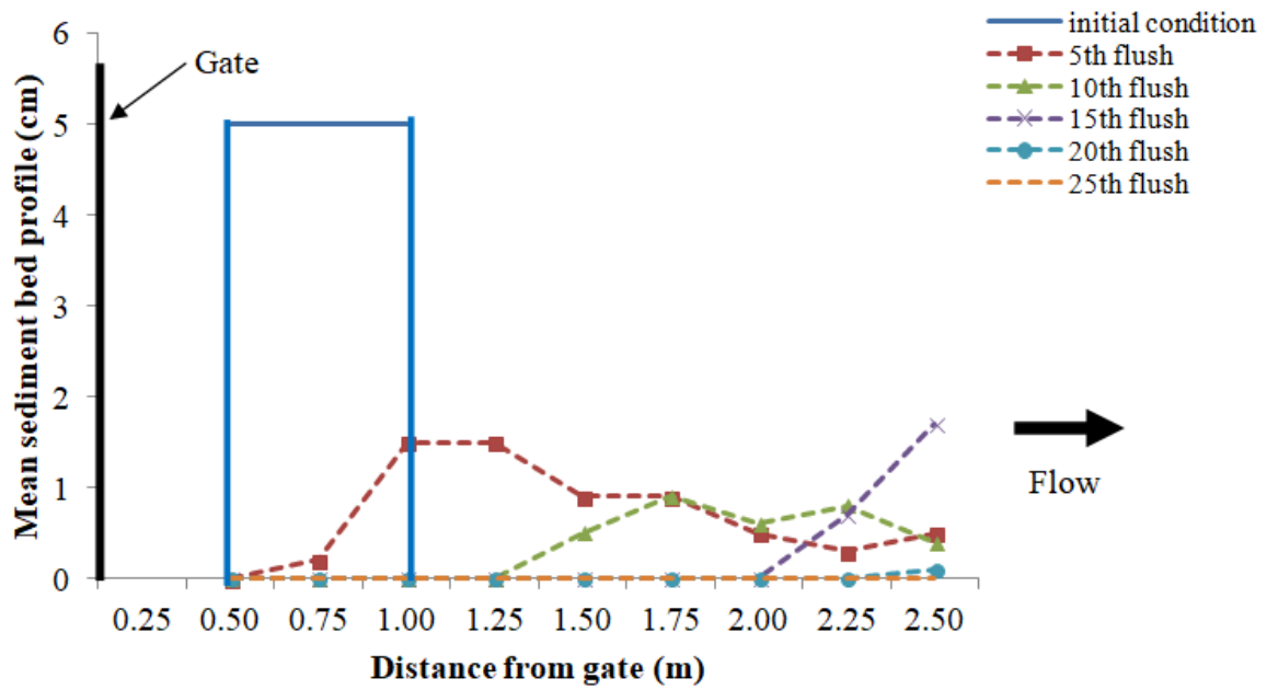
Figure 4.6: Sediment profiles for sediment d_{50} of 2 mm laid starting from 0.5 m to 1.0 m from the gate with \theta = 60^\circ after flushes for 5 cm initial sediment deposition thickness
