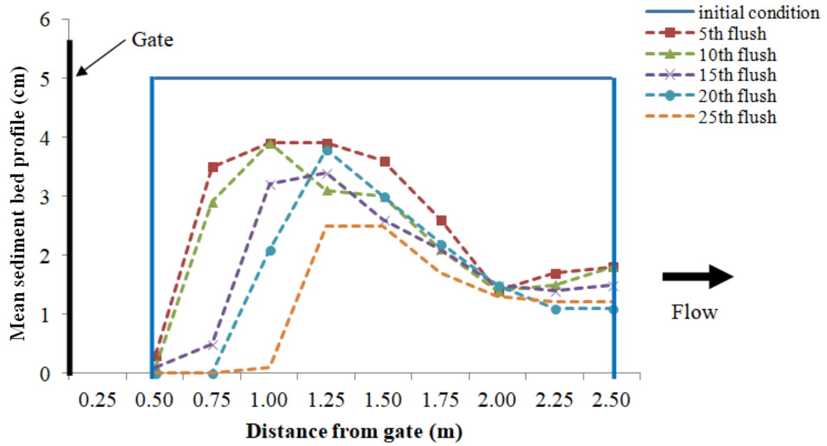
Figure B.3: Sediment profiles for sediment d_{50} of 1.18 mm laid starting from 0.5 m from the gate with \theta = 60^\circ after flushes for 5 cm initial sediment deposition thickness
