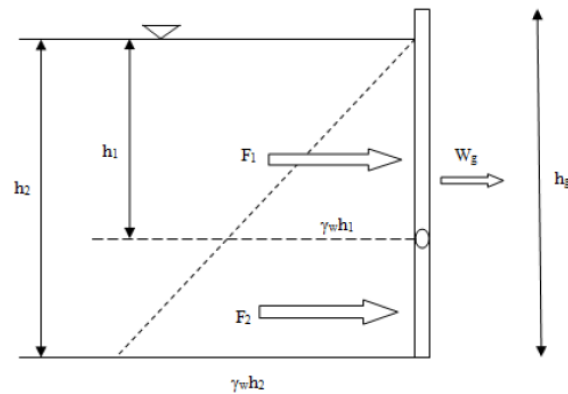
Figure 5.4: Forces acting on tipping flush gate before opening (Bong et al., 2016)
