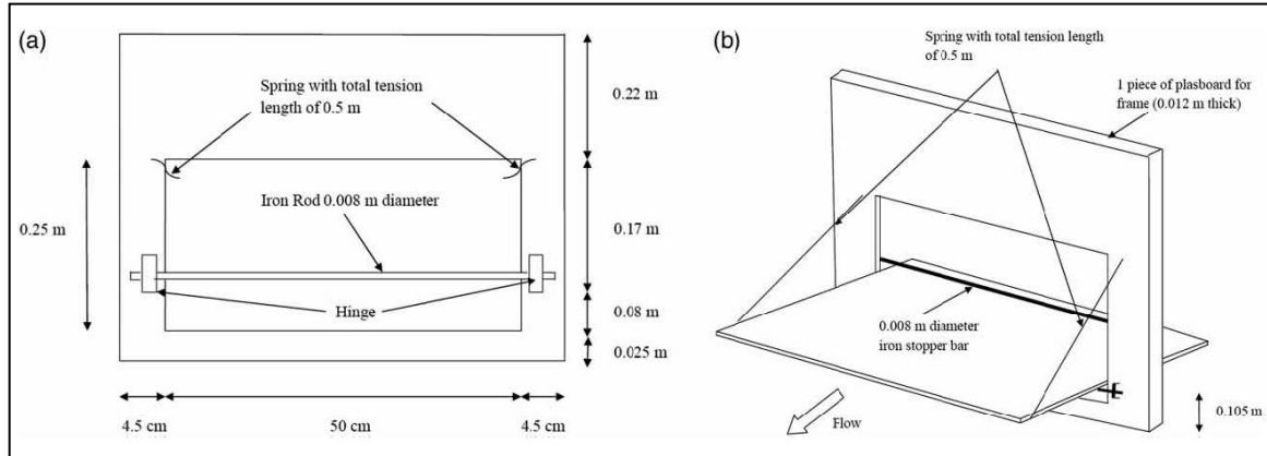
Figure 1. Views of the model tipping flush gate (a) front view; and (b) isometric view (not to scale) (Bong, Lau and Ab. Ghani, 2013)
