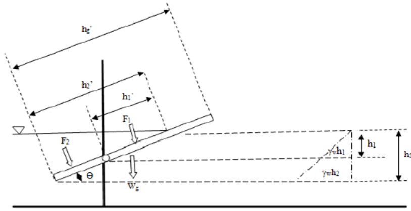
Figure 2.10: Forces acting on tipping flushing gate when open (Bong et al., 2016).
