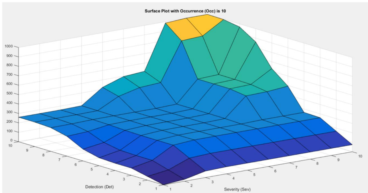
Figure 4.30: A surface plot of FRPN versus Sev and Det with Occ was 10
