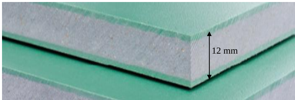
Figure 2.5: Thickness of double layer GCV Plasboard
