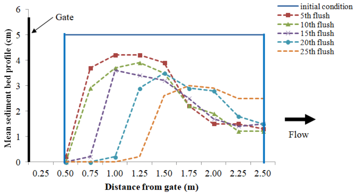
Figure 4.8: Sediment profiles for sediment d_{50} of 2 mm laid starting from 0.5 m to 2.5 m from the gate with \theta = 60^\circ after flushes for 5 cm initial sediment deposition thickness
