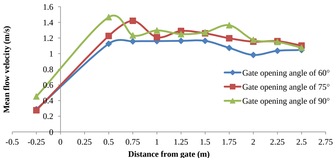
Figure 4.1: Mean flow velocity for \theta = 60^\circ
