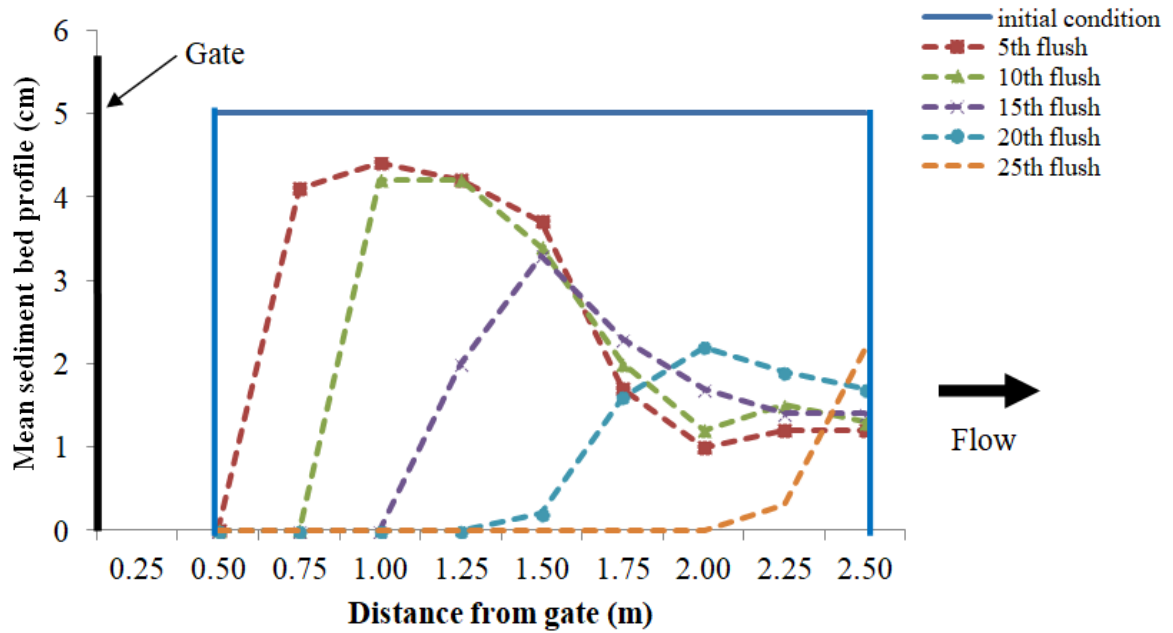
Figure B.4: Sediment profiles for sediment d_{50} of 2 mm laid starting from 0.5 m from the gate with \theta = 90^\circ after flushes for 5 cm initial sediment deposition thickness
