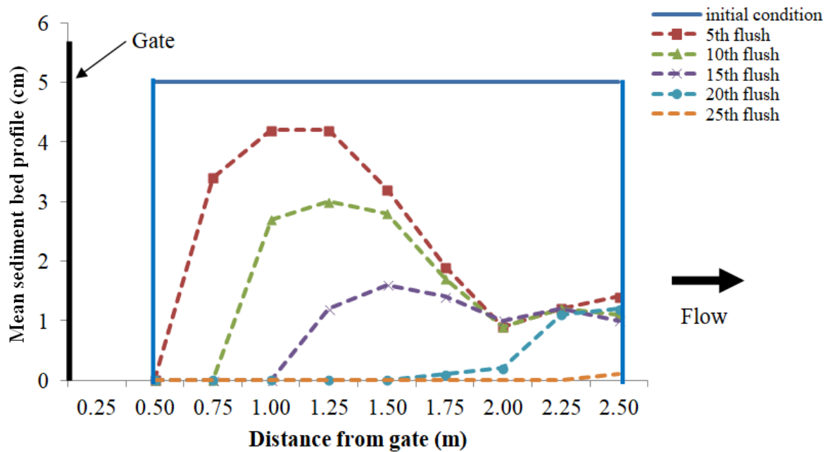
Figure B.12: Sediment profiles for sediment d_{50} of 0.71 mm laid starting from 0.5 m to 2.5 m from the gate with \theta = 90^\circ after flushes for 5 cm initial sediment deposition thickness
