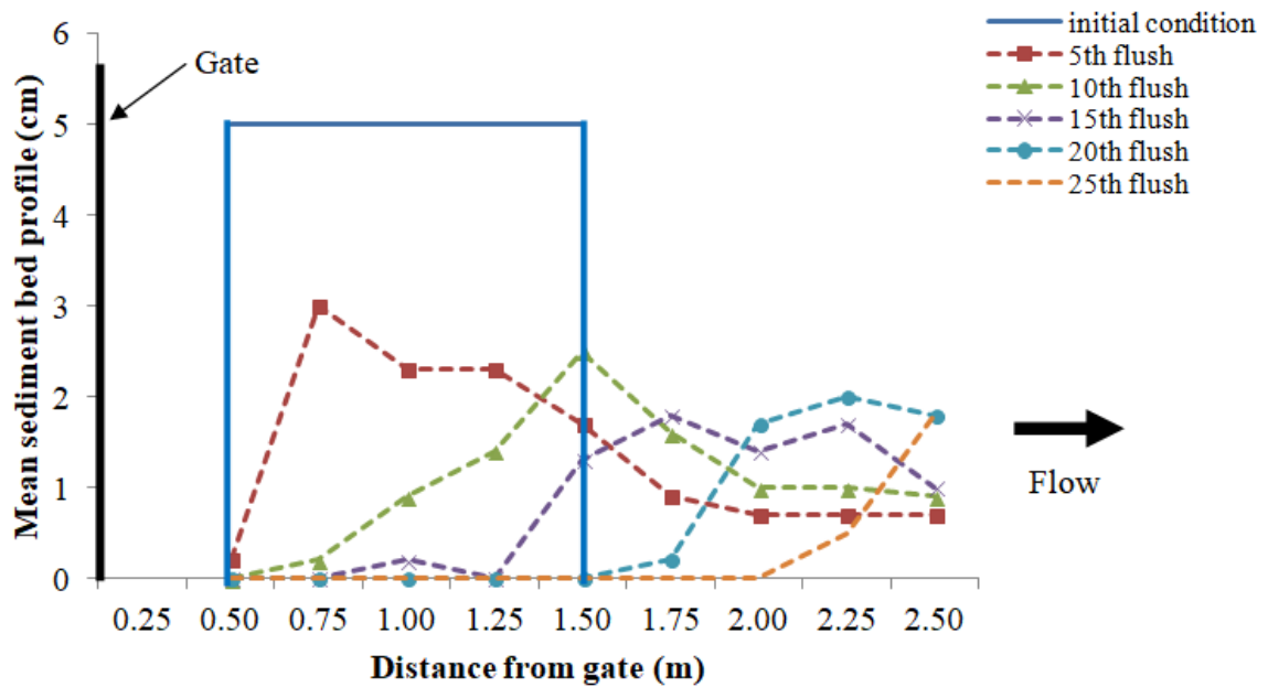
Figure 4.7: Sediment profiles for sediment d_{50} of 2 mm laid starting from 0.5 m to 1.5 m from the gate with \theta = 60^\circ after flushes for 5 cm initial sediment deposition thickness
