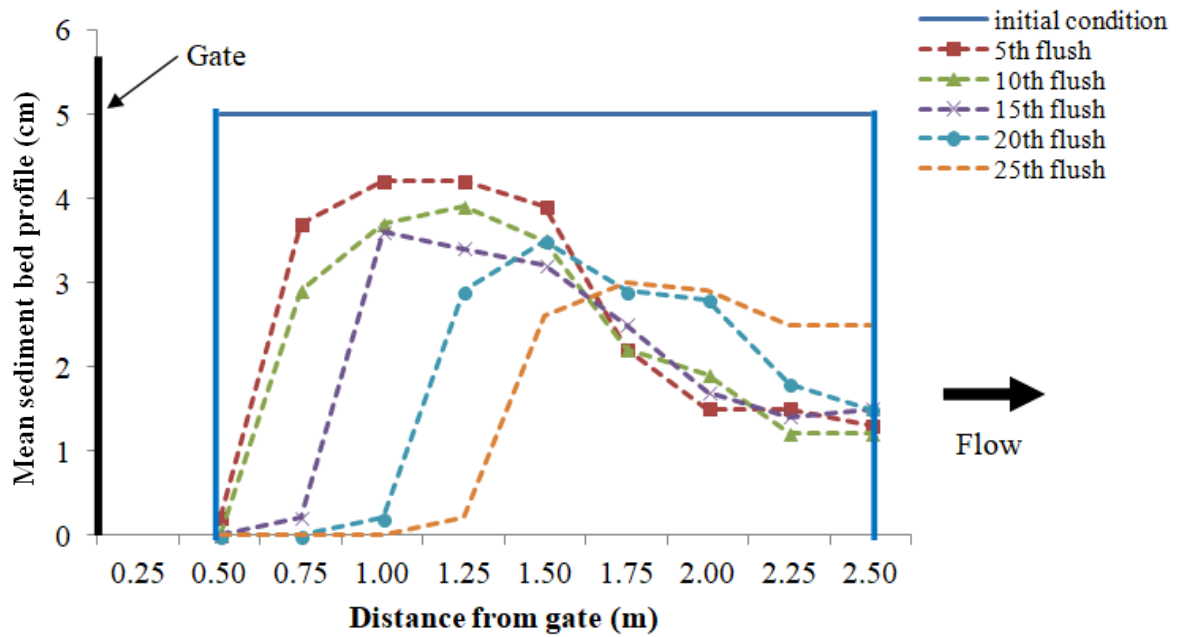
Figure B.6: Sediment profiles for sediment d_{50} of 2 mm laid starting from 0.5 m from the gate with \theta = 60^\circ after flushes for 5 cm initial sediment deposition thickness
