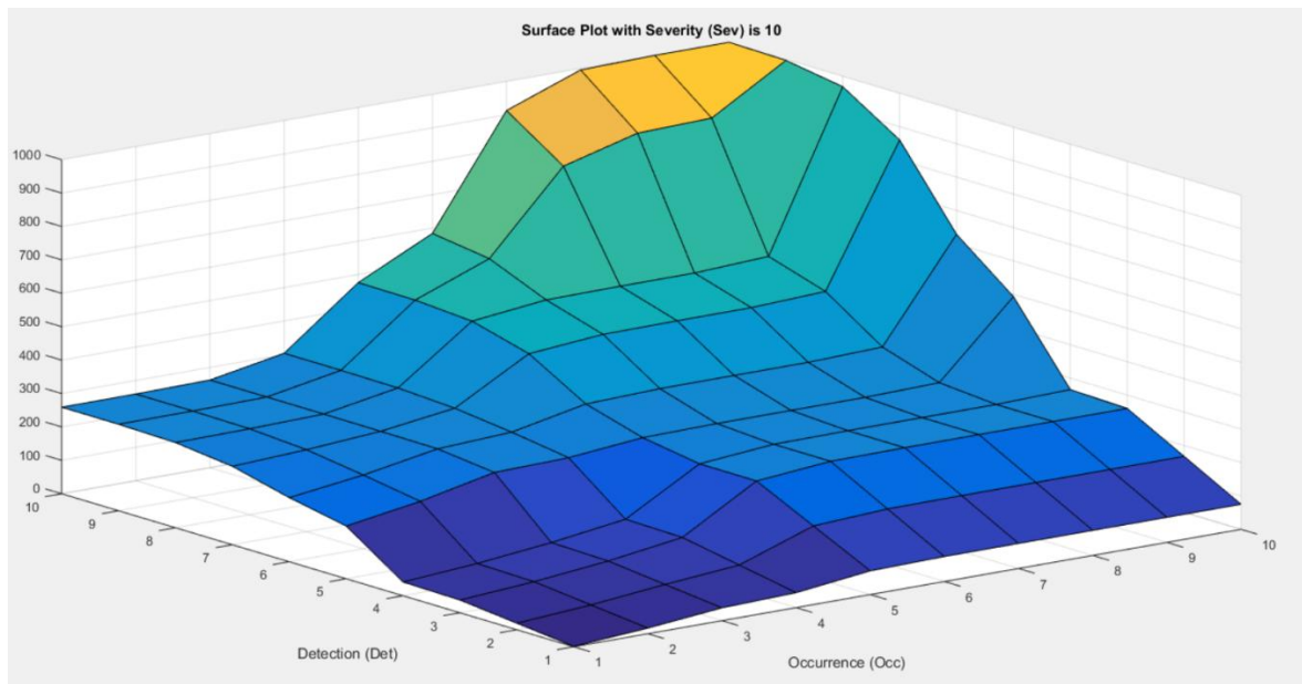
Figure 4.29: A surface plot of FRPN versus Occ and Det with Sev was 10
