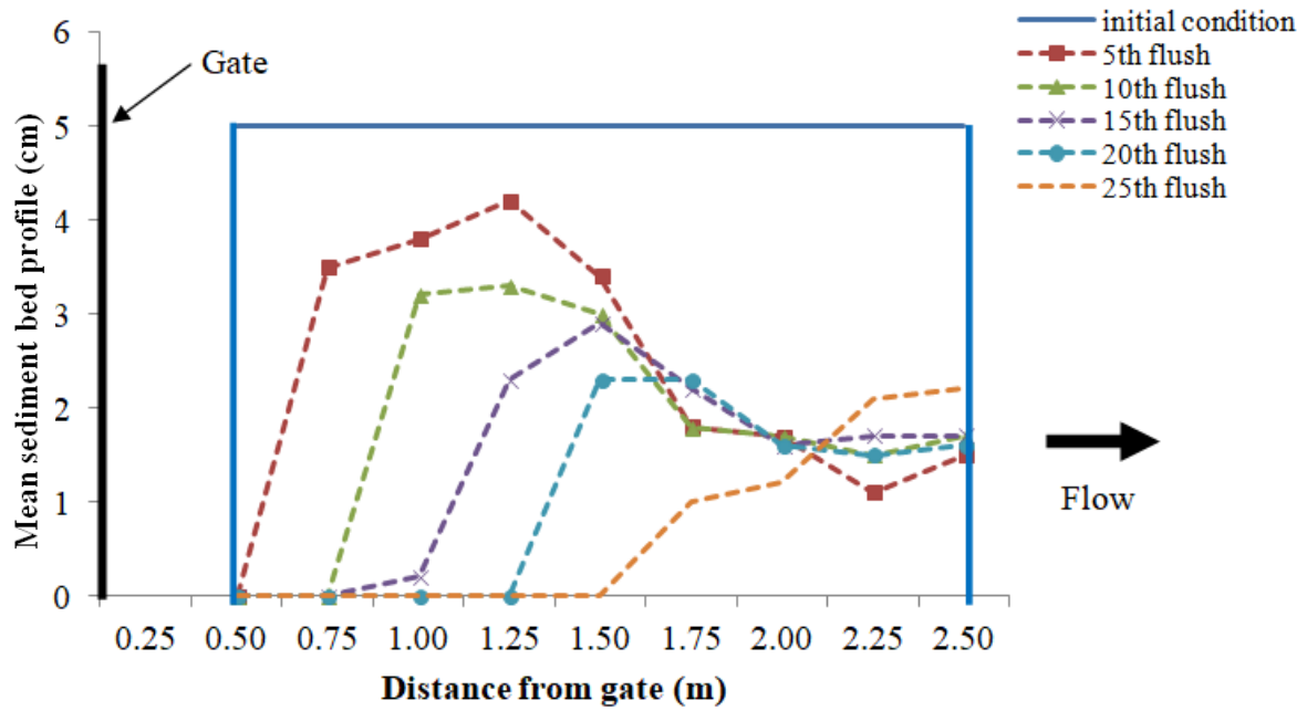
Figure 4.5: Sediment profiles for sediment d_{50} of 0.71 mm laid starting from 0.5 m from the gate with \theta = 60^\circ after flushes for 5 cm initial sediment deposition thickness
