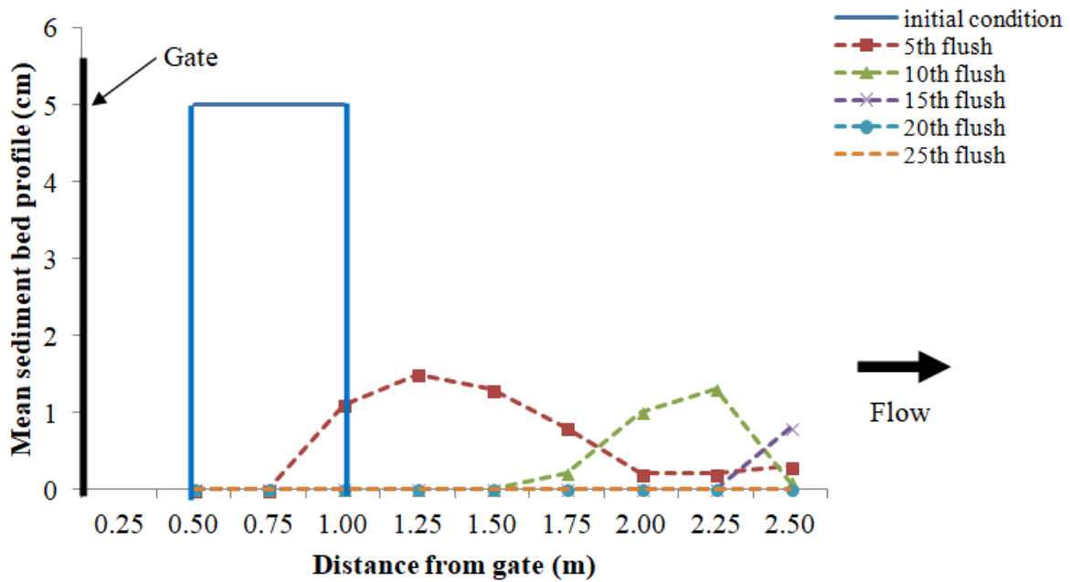
Figure B.10: Sediment profiles for sediment d_{50} of 0.71 mm laid starting from 0.5 m to 1.0 m from the gate with \theta = 60^\circ after flushes for 5 cm initial sediment deposition thickness
