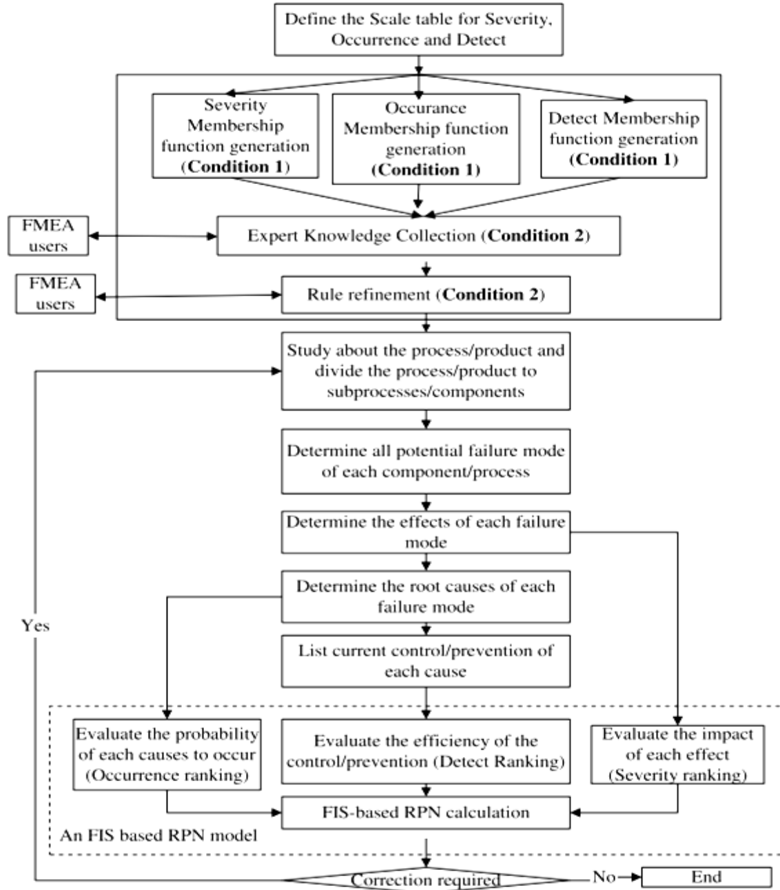
Figure 2.11: Enhancement of FMEA methodology with the FIS_RPN model (Tay & Lim, 2010)
