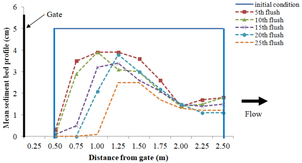
Figure B.9: Sediment profiles for sediment d_{50} of 1.18 mm laid starting from 0.5 m to 2.5 m from the gate with \theta = 60^\circ after flushes for 5 cm initial sediment deposition thickness
