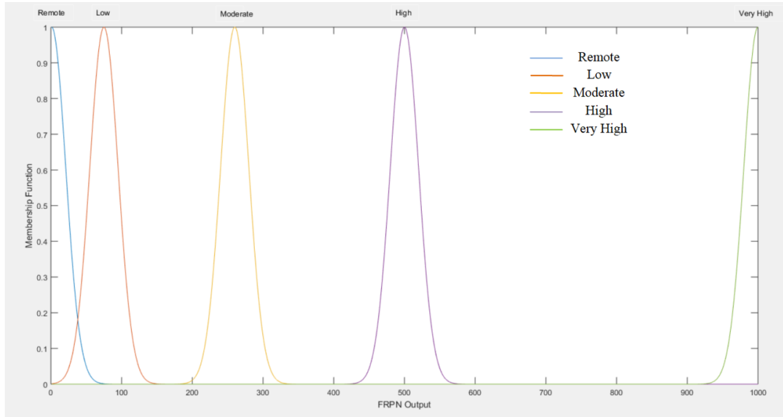
Figure 4.28: The fuzzy sets for FRPN output
