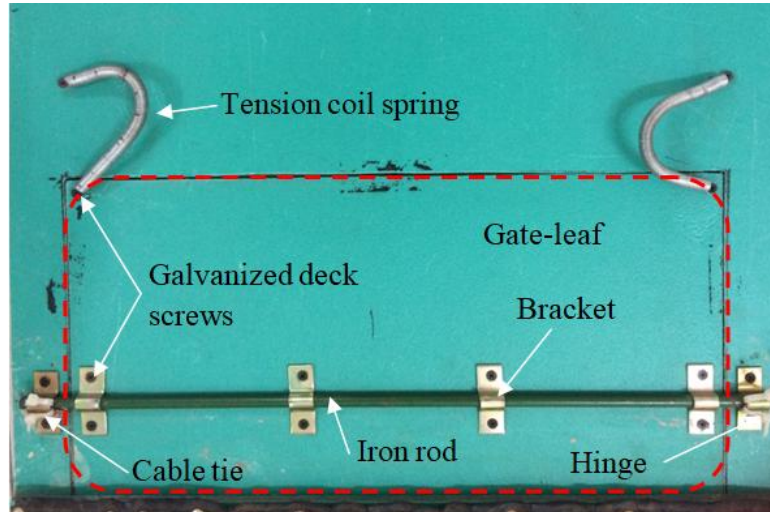
Figure 2.7: Components of gate-opening subsystem
