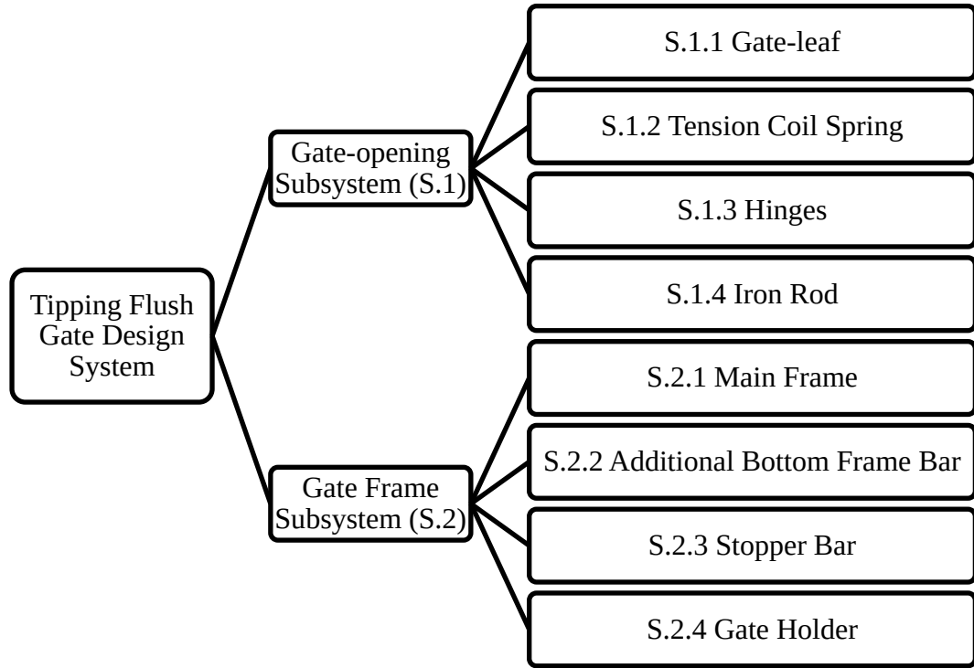
Figure 2.6: Hierarchy structure of tipping flush gate
