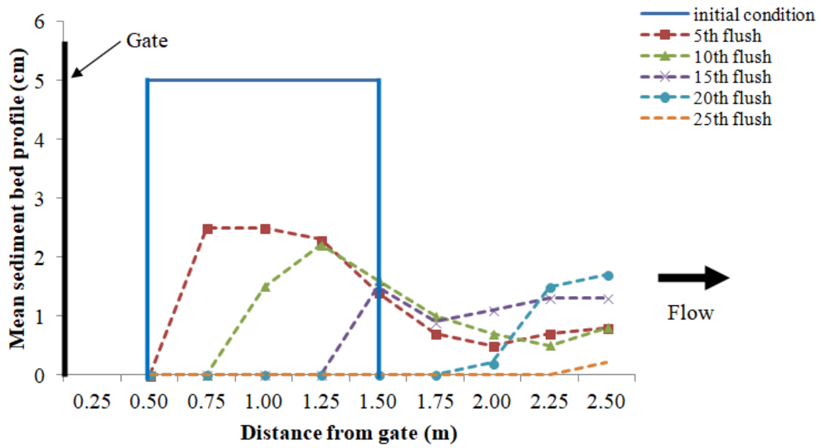
Figure B.11: Sediment profiles for sediment d_{50} of 0.71 mm laid starting from 0.5 m to 1.5m from the gate with \theta = 60^\circ after flushes for 5 cm initial sediment deposition thickness
