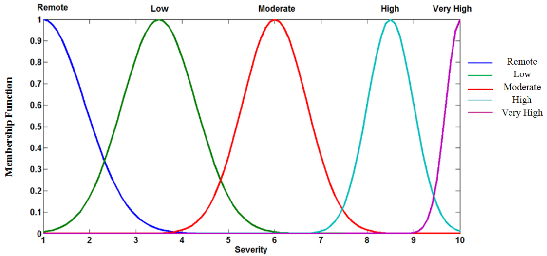
Figure 4.25: Membership functions for Sev
