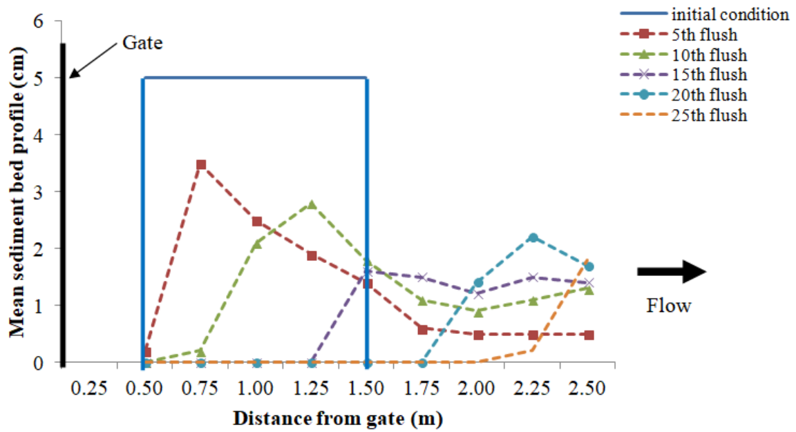
Figure B.8: Sediment profiles for sediment d_{50} of 1.18 mm laid starting from 0.5 m to 1.5 m from the gate with \theta = 60^\circ after flushes for 5 cm initial sediment deposition thickness
