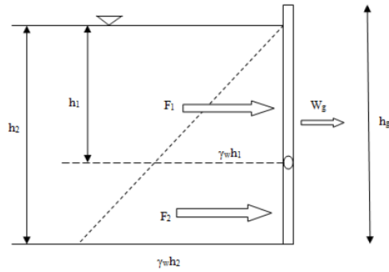
Figure 2.9: Forces acting on tipping flush gate before opening (Bong et al., 2016)
