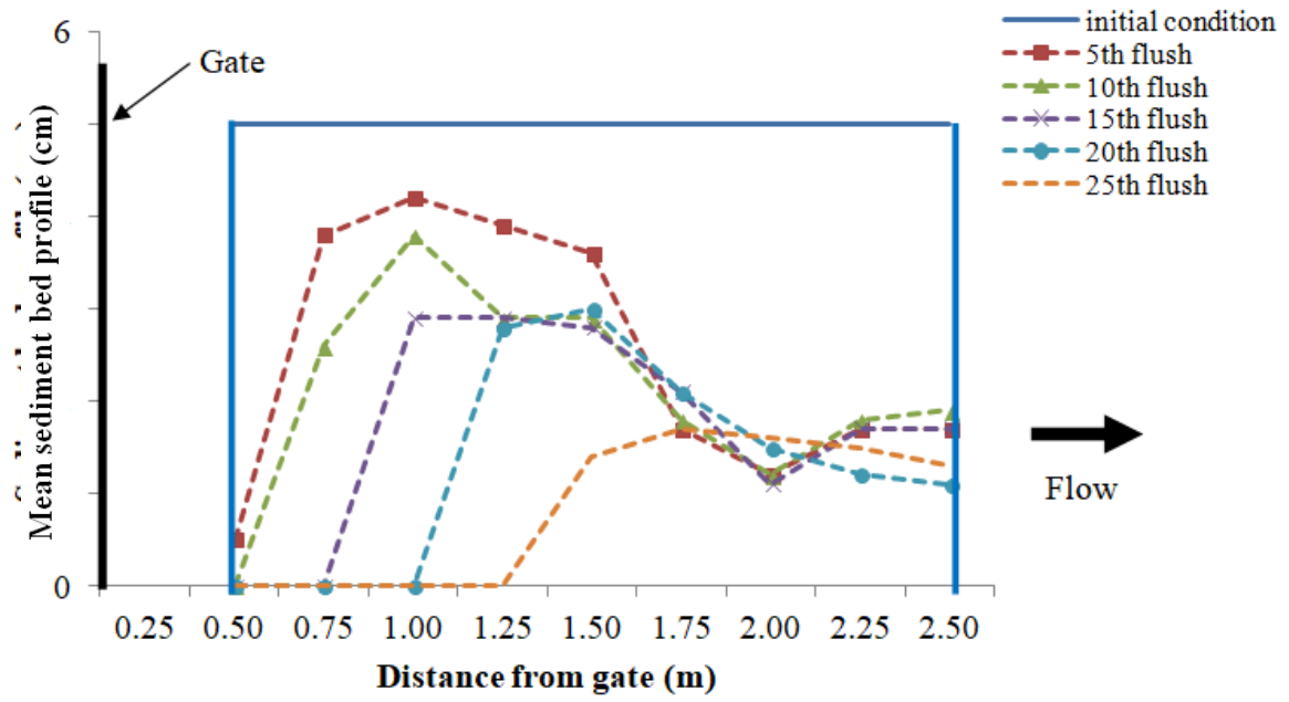
Figure B.5: Sediment profiles for sediment d_{50} of 2 mm laid starting from 0.5 m from the gate with \theta = 75^\circ after flushes for 5 cm initial sediment deposition thickness
