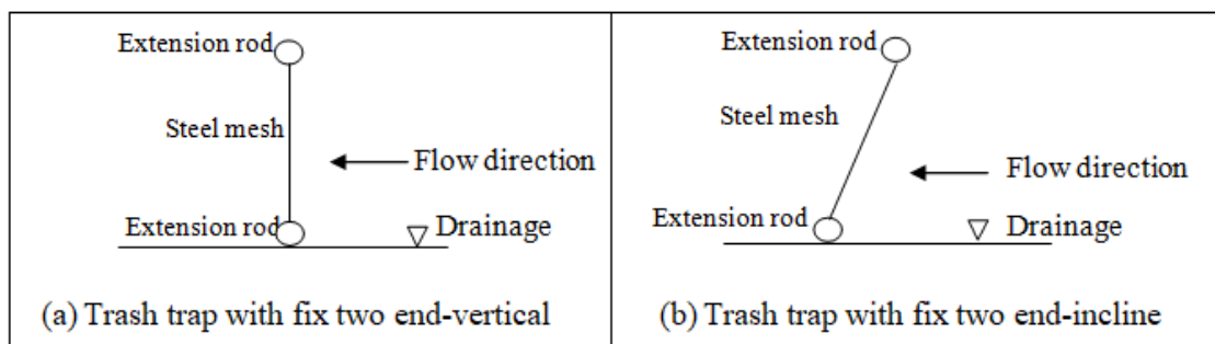
Figure 4.23: Schematic diagrams of the trash trap (side view)
