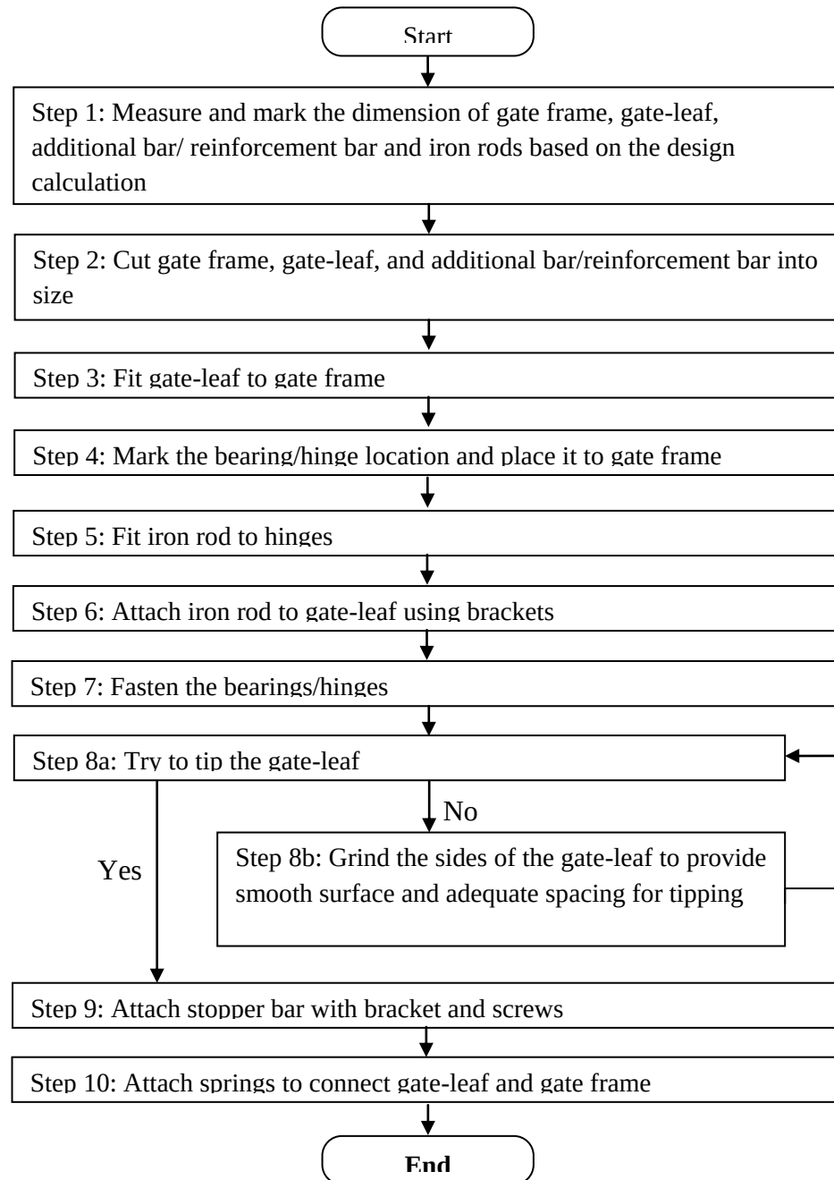
Figure 5.6: Tipping flush gate construction and assembly process chart
