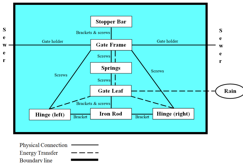
Figure 3.2: FMEA block diagram for tipping flush gate
