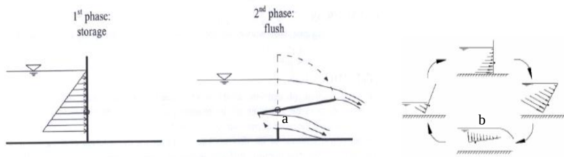
Figure 2.3: Sequences of Hydrass gate operation (Campisano et al., 2006)
